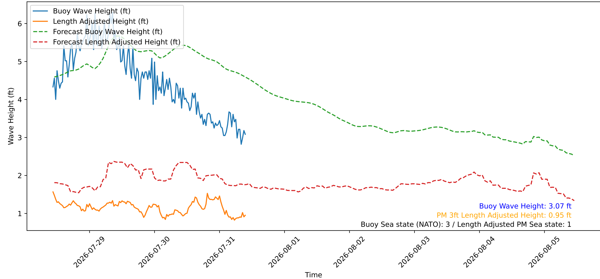
Wave Heights over Time for Green Beach at 2026-07-31 10:31:09
