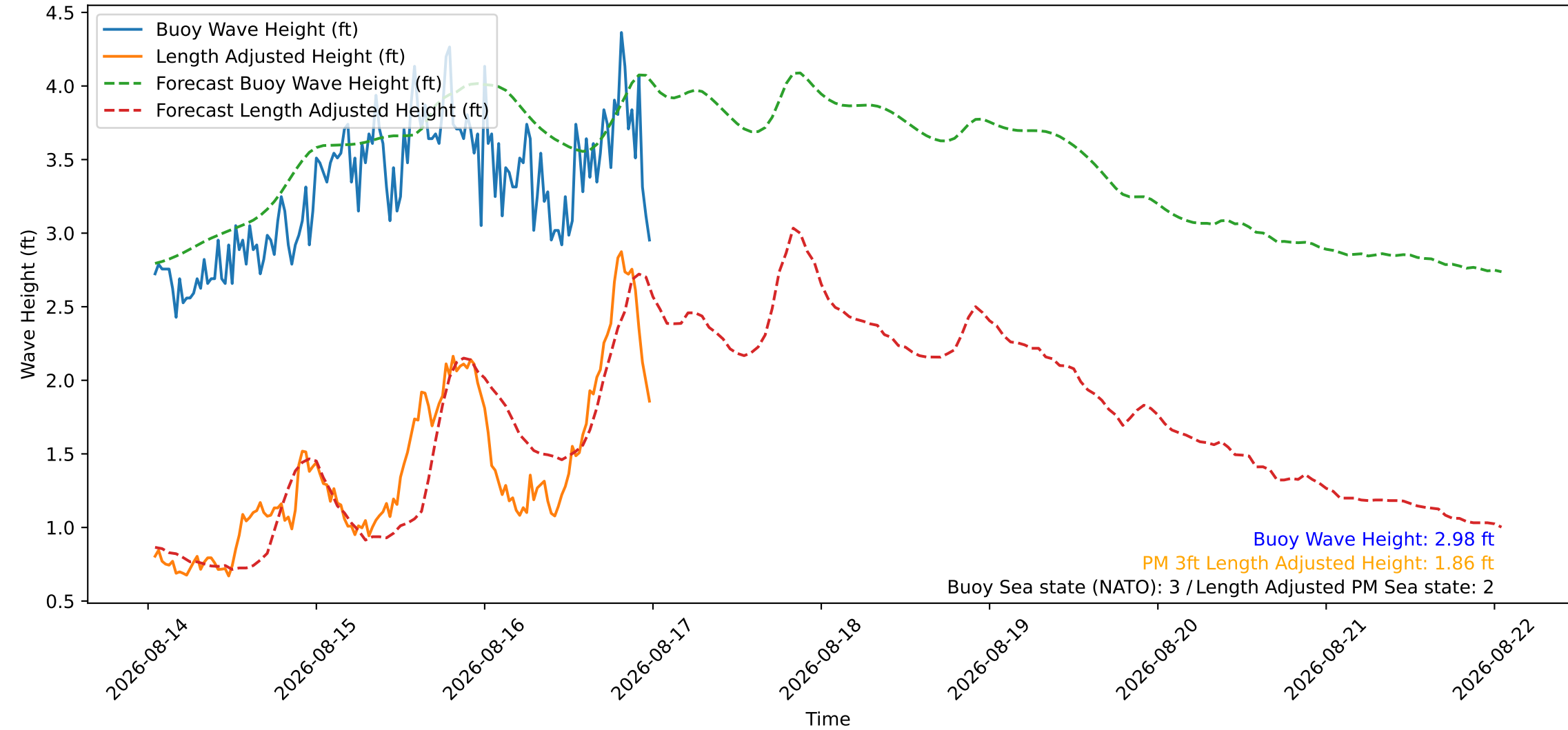
Wave Heights over Time for Green Beach at 2026-08-17 00:31:08
