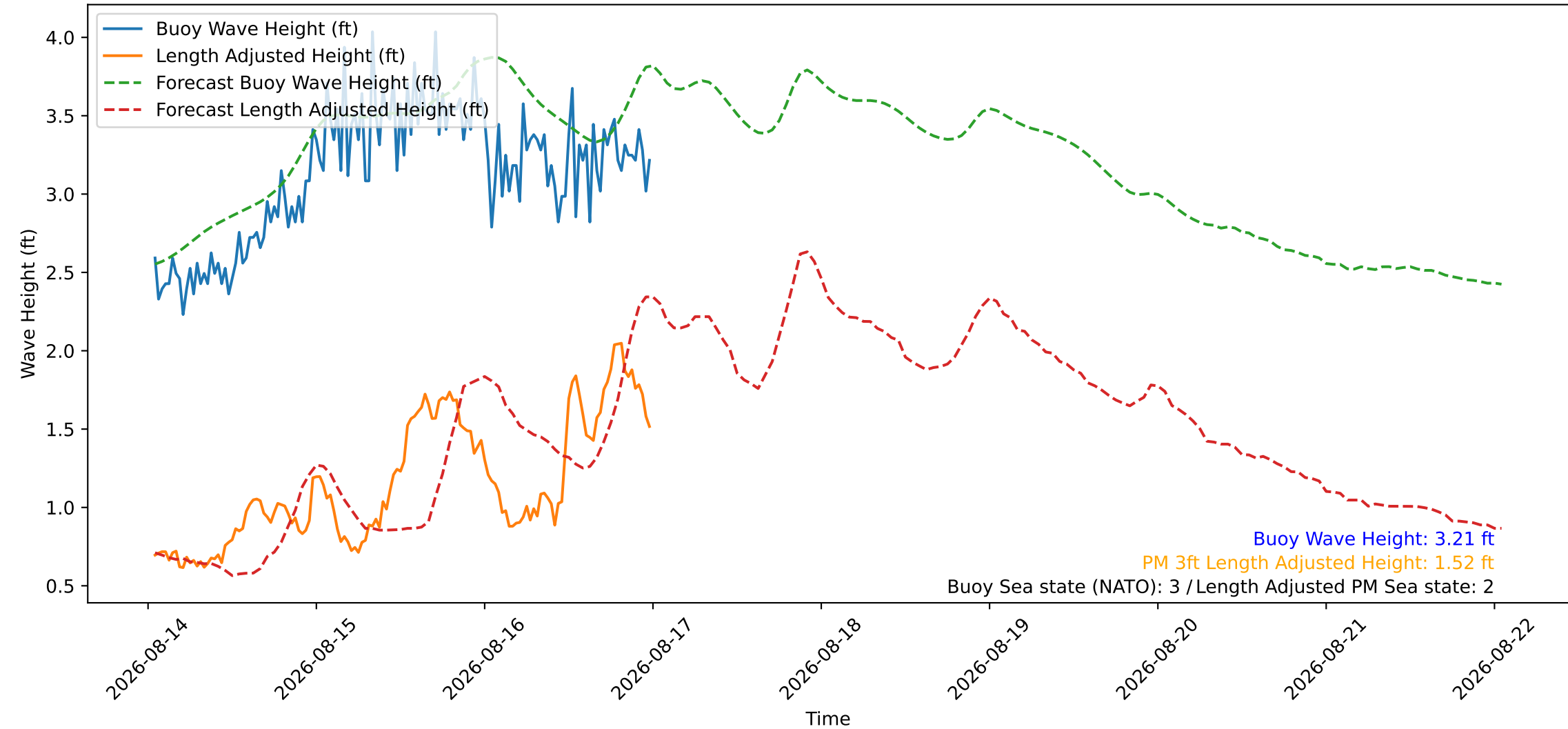
Wave Heights over Time for Red Beach at 2026-08-17 00:30:46
