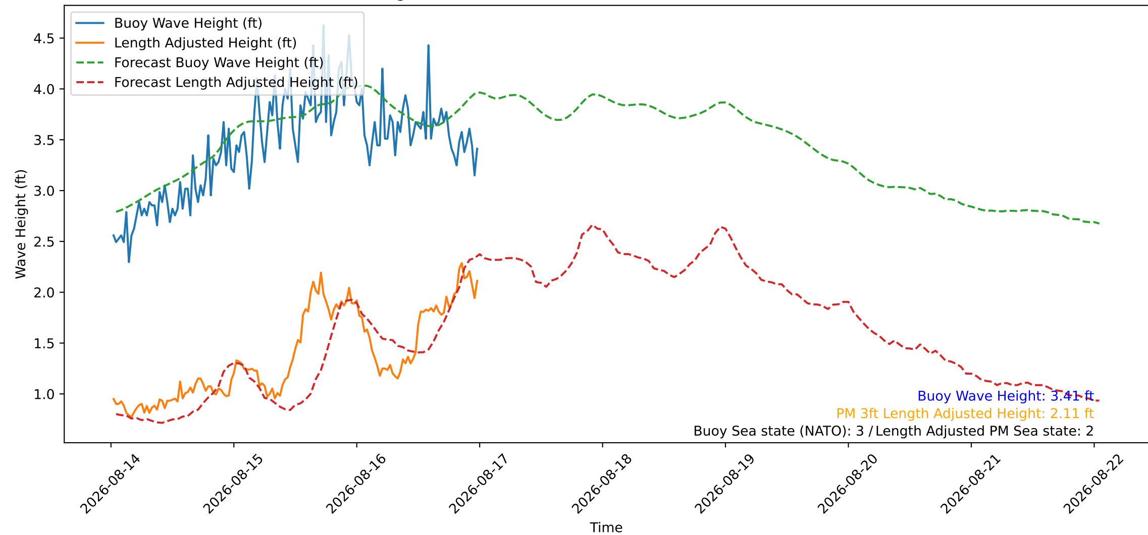
Wave Heights over Time for Oceanside Harbor at 2026-08-17 00:30:26
