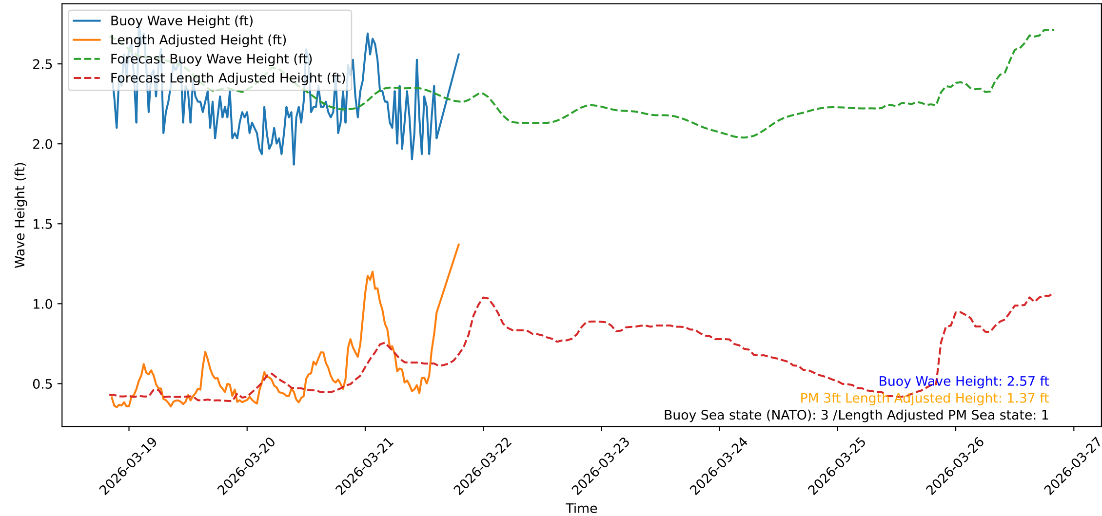
Wave Heights over Time for Red Beach at 2026-03-21 20:00:48
