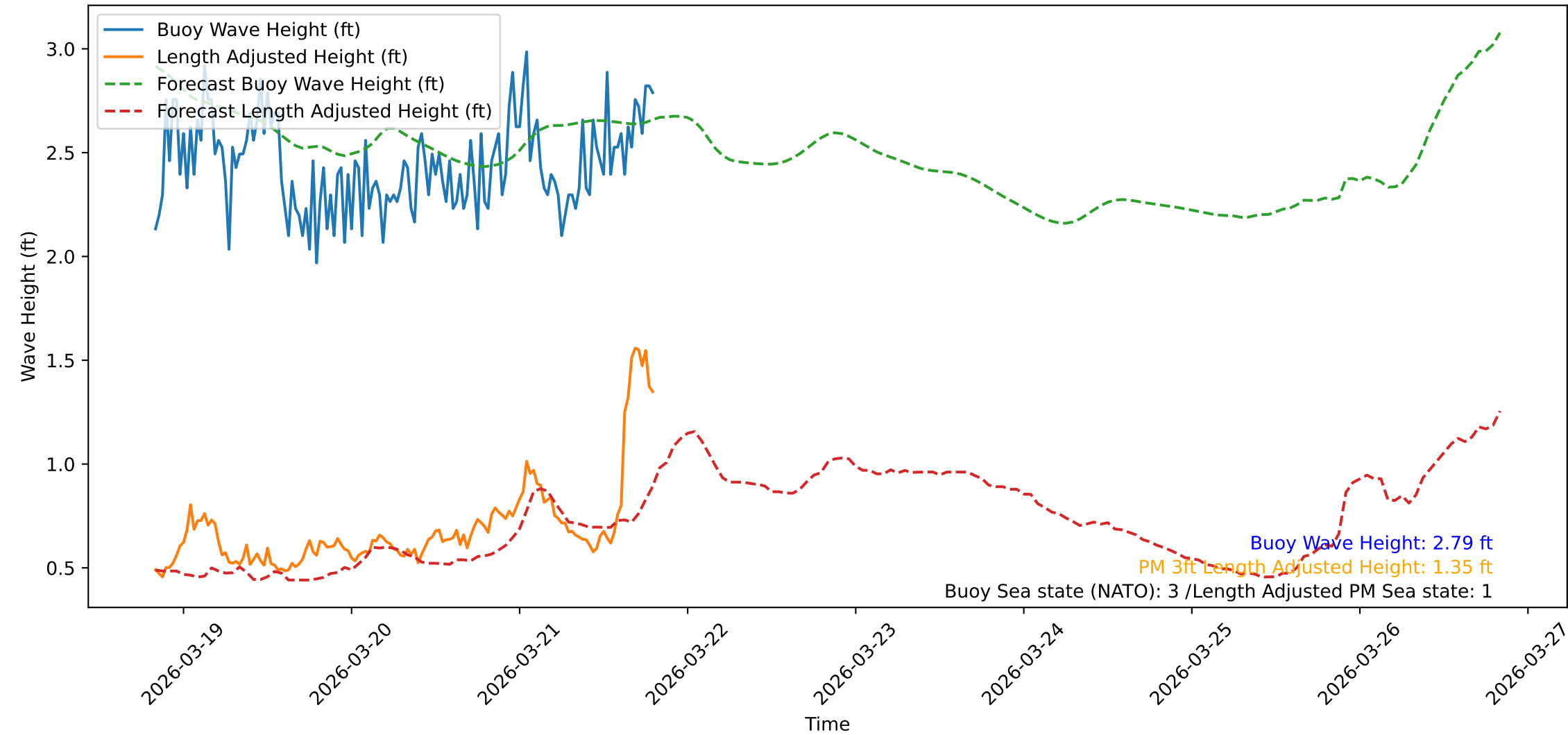
Wave Heights over Time for Oceanside Harbor at 2026-03-21 20:00:33
