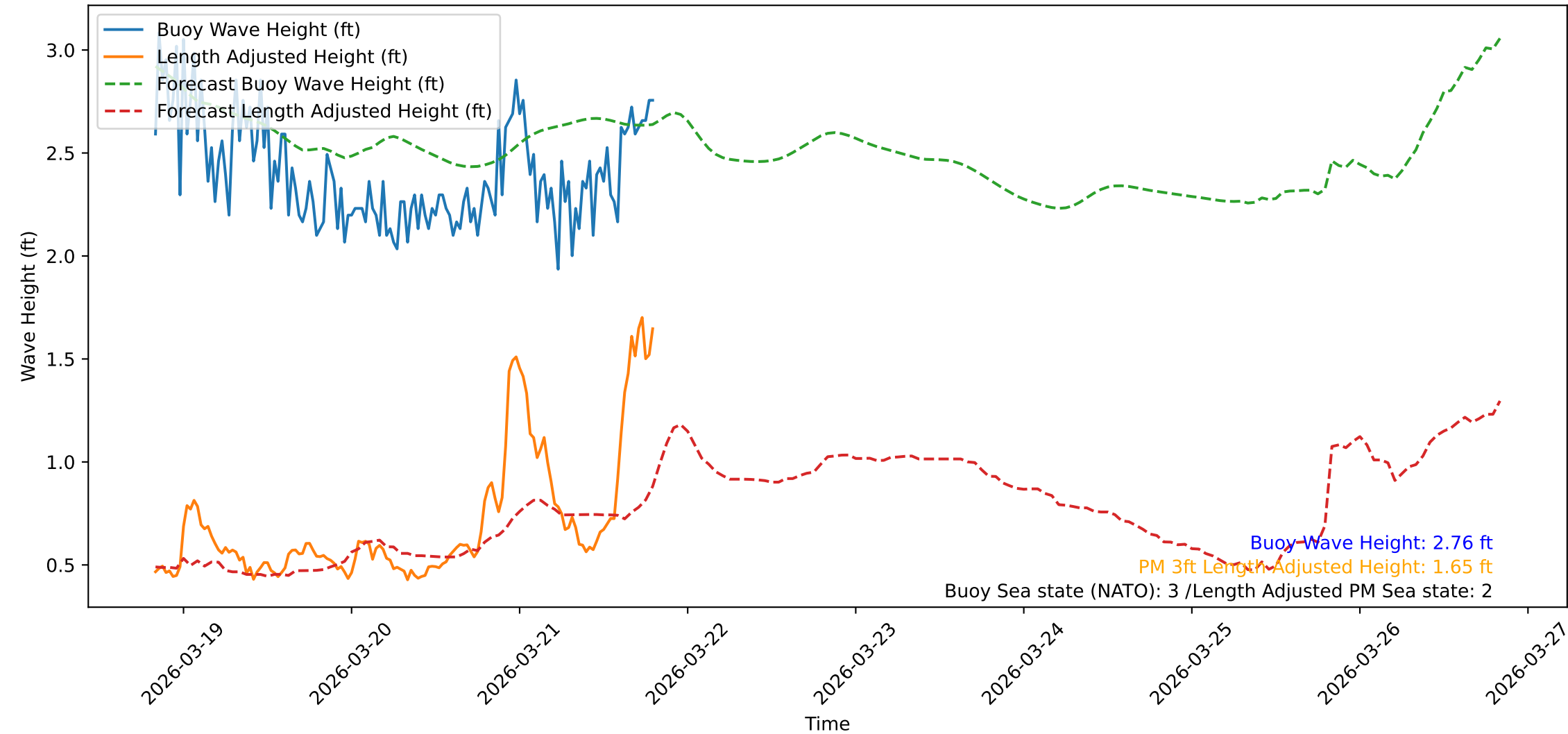
Wave Heights over Time for Green Beach at 2026-03-21 20:01:10
