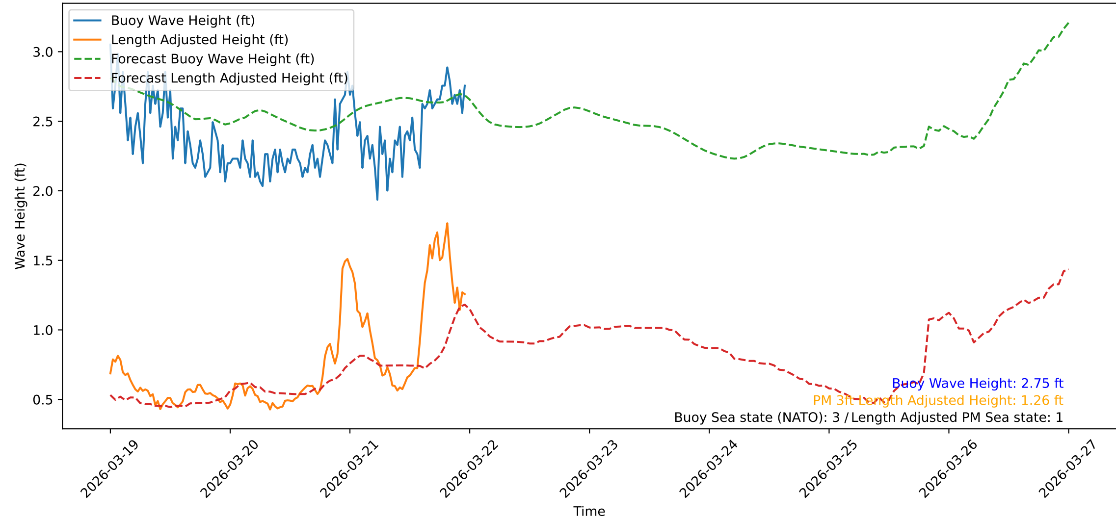
Wave Heights over Time for Green Beach at 2026-03-21 23:51:09
