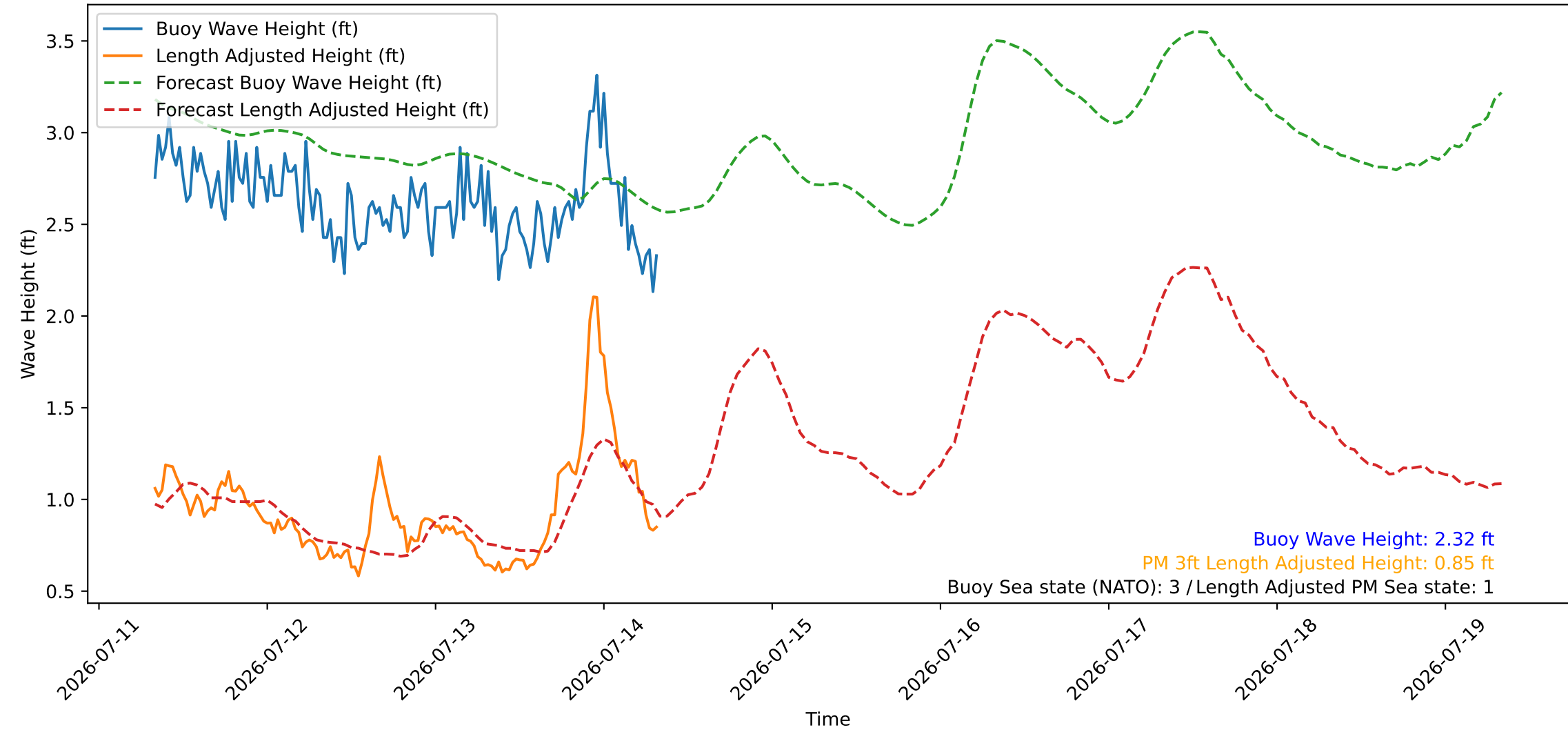
Wave Heights over Time for Green Beach at 2026-07-14 08:11:08
