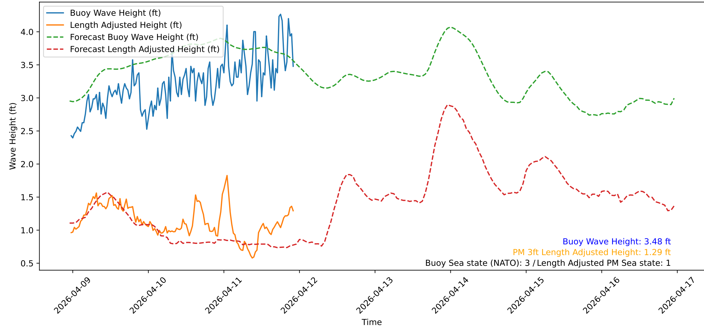
Wave Heights over Time for Red Beach at 2026-04-11 23:20:52
