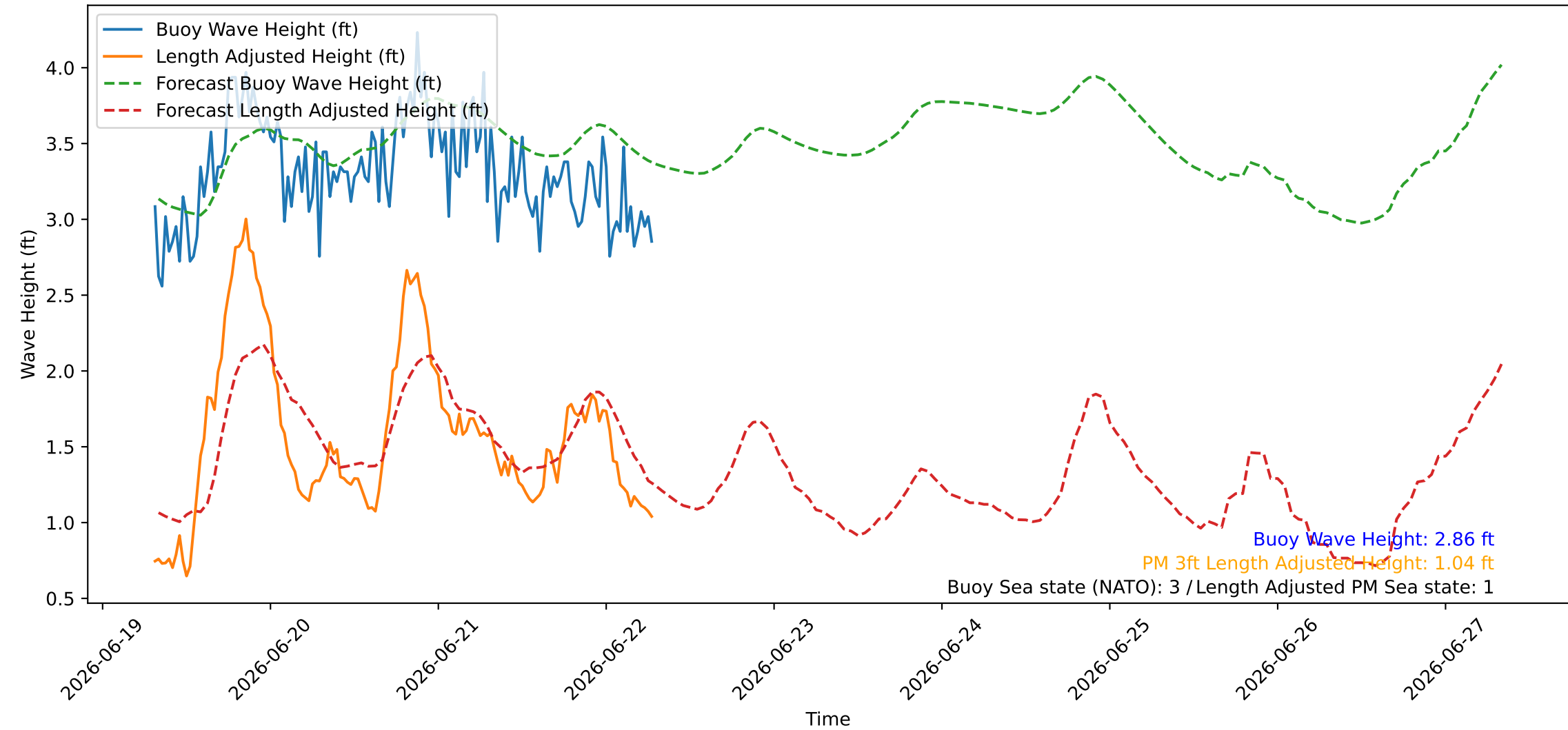
Wave Heights over Time for Green Beach at 2026-06-22 07:31:07
