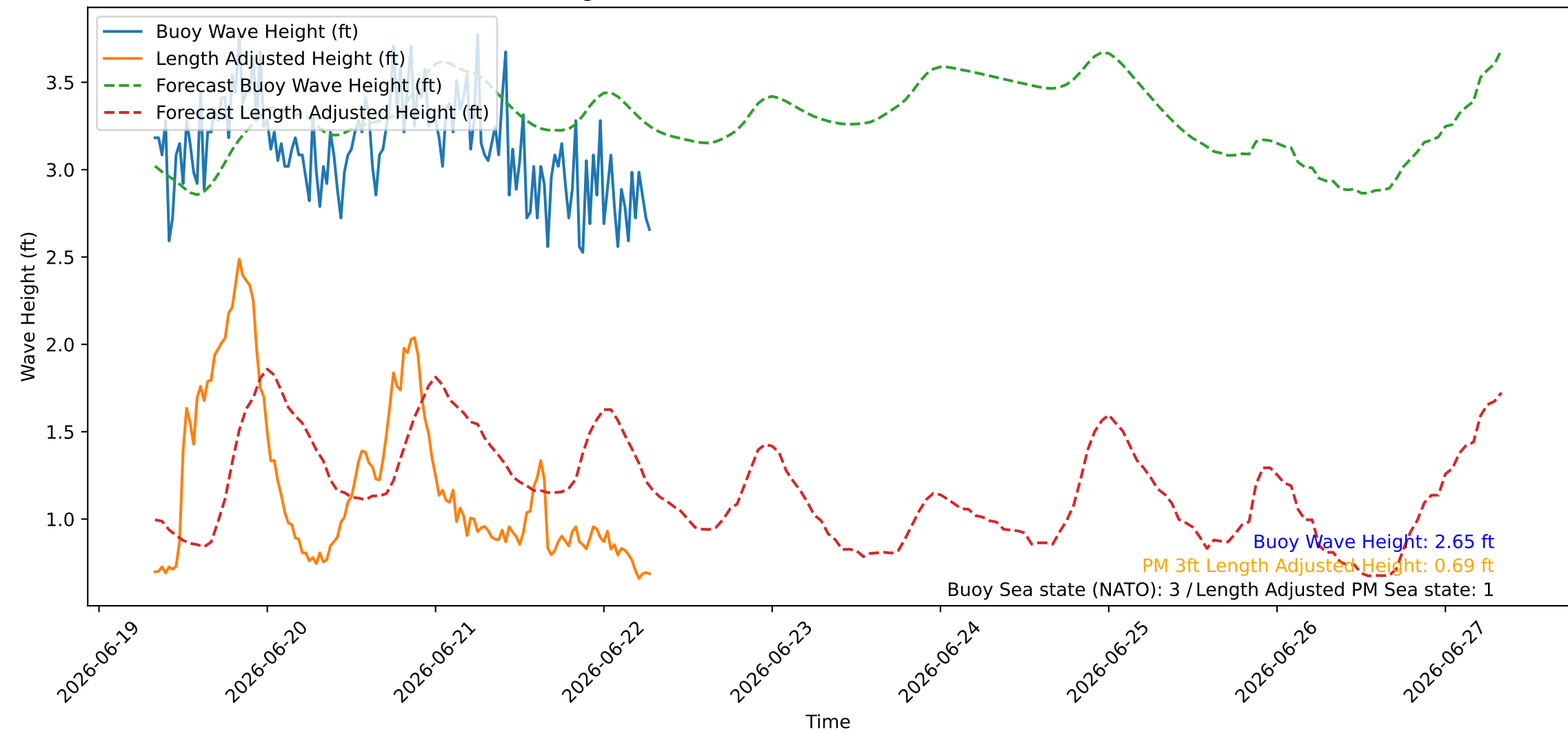
Wave Heights over Time for Red Beach at 2026-06-22 07:30:45
