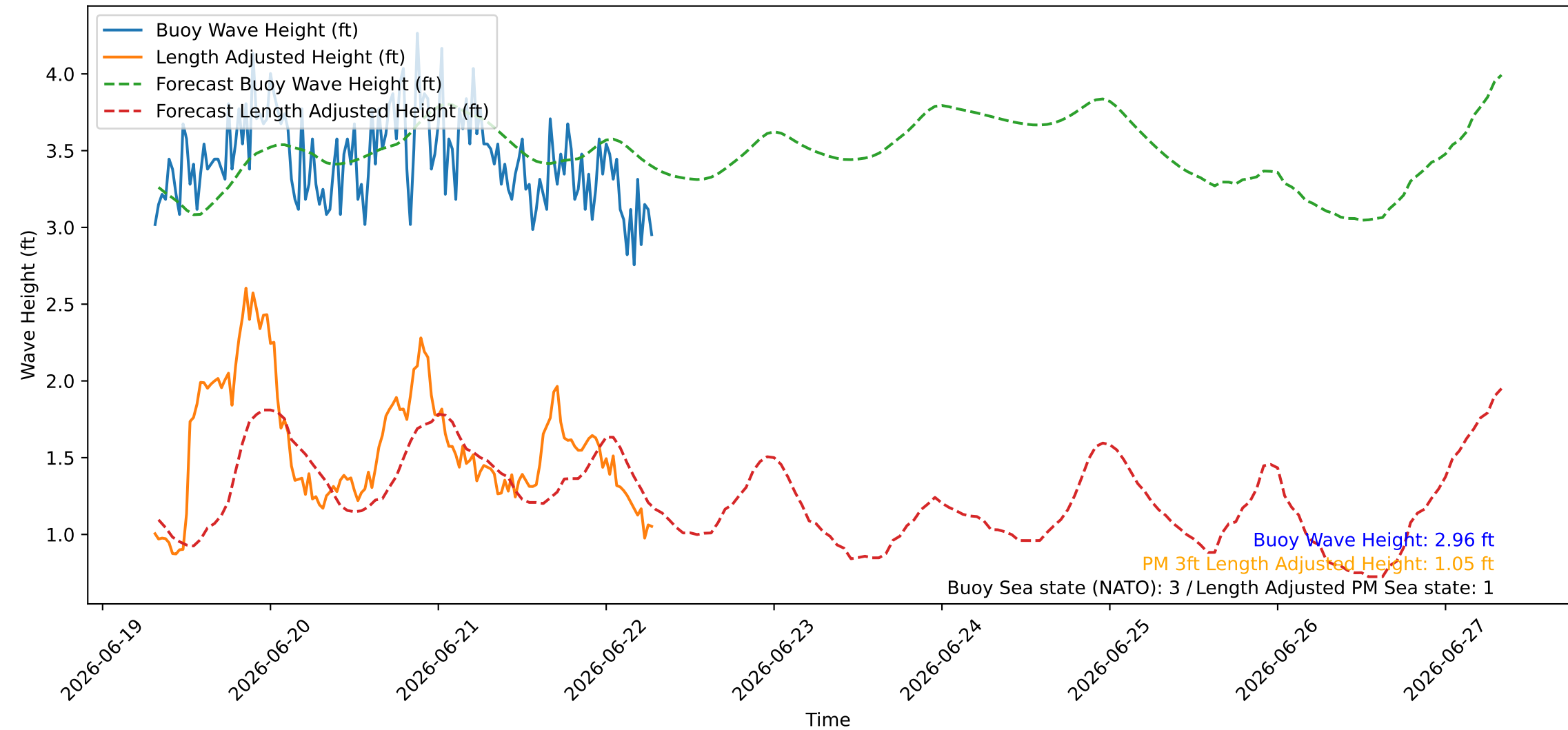
Wave Heights over Time for Oceanside Harbor at 2026-06-22 07:30:26
