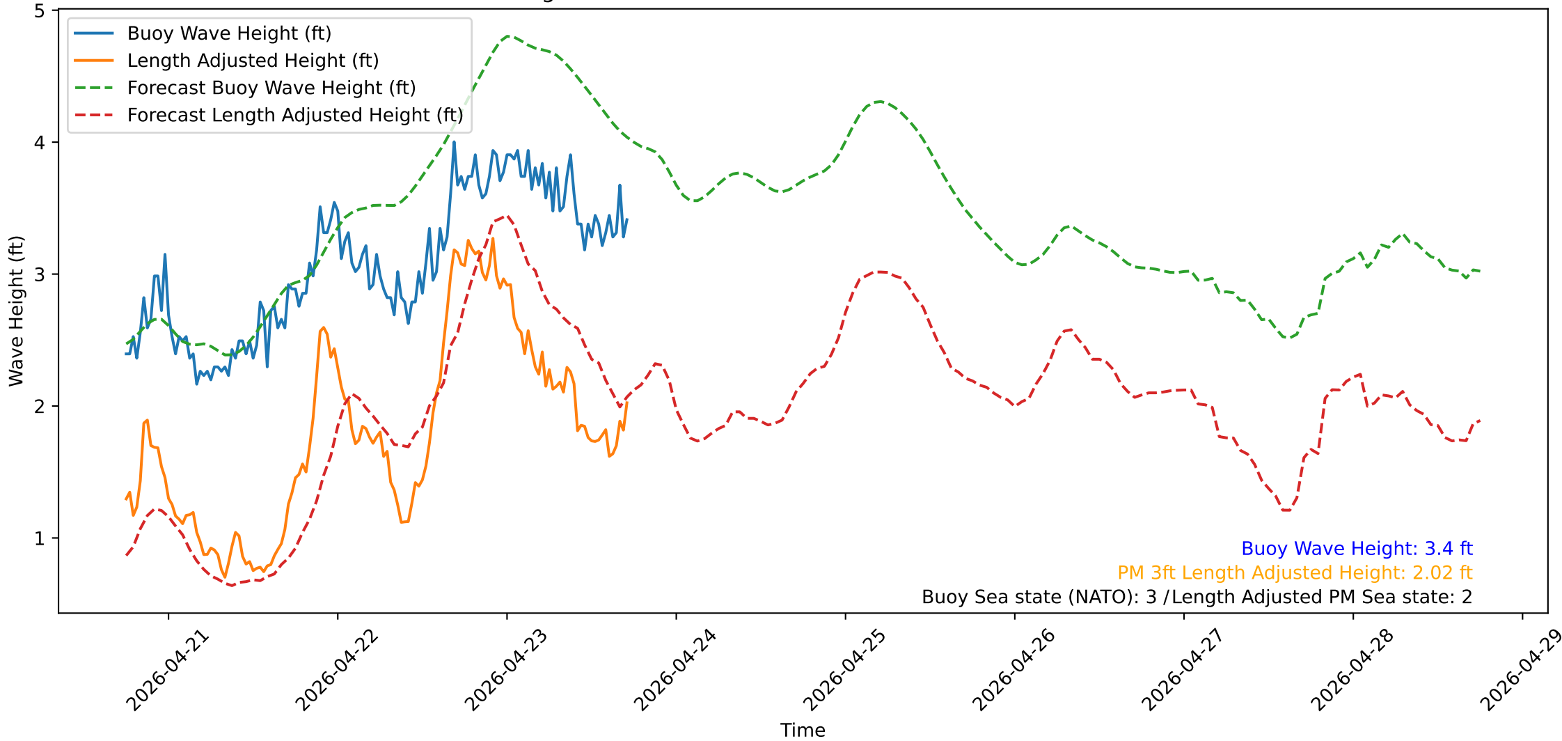
Wave Heights over Time for Green Beach at 2026-04-23 18:01:12
