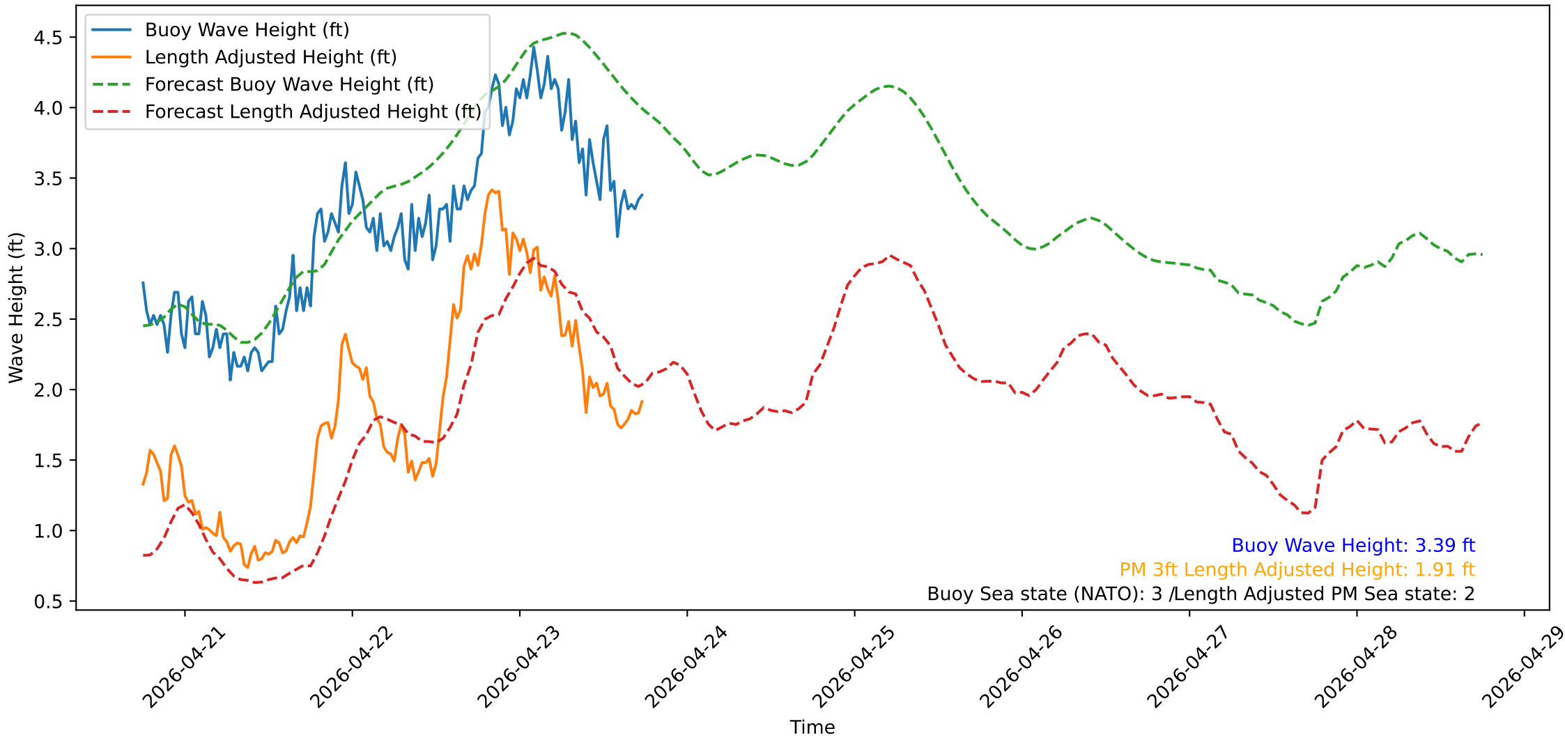
Wave Heights over Time for Oceanside Harbor at 2026-04-23 18:00:31
