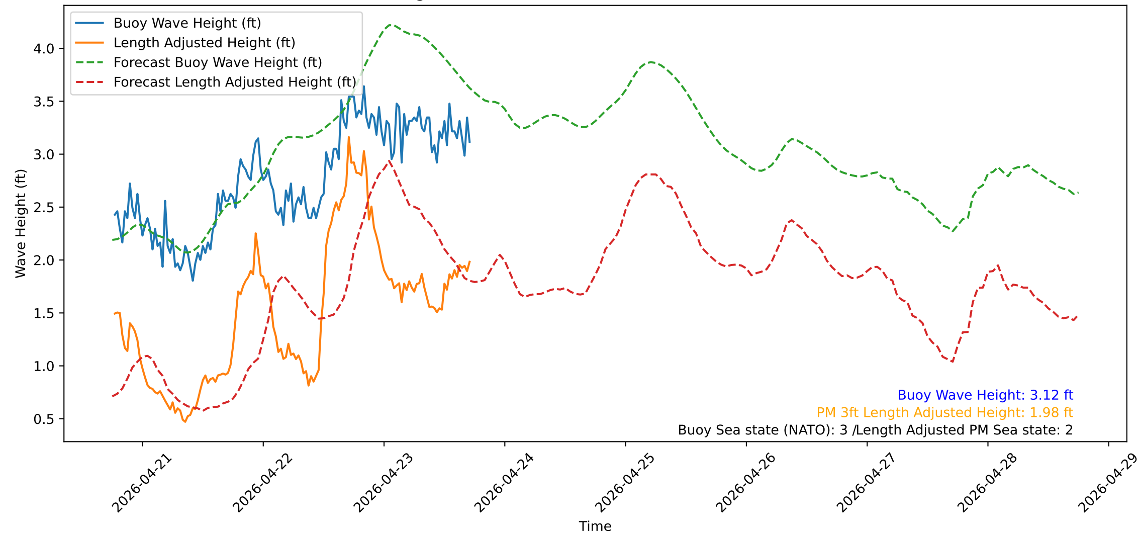
Wave Heights over Time for Red Beach at 2026-04-23 18:00:50
