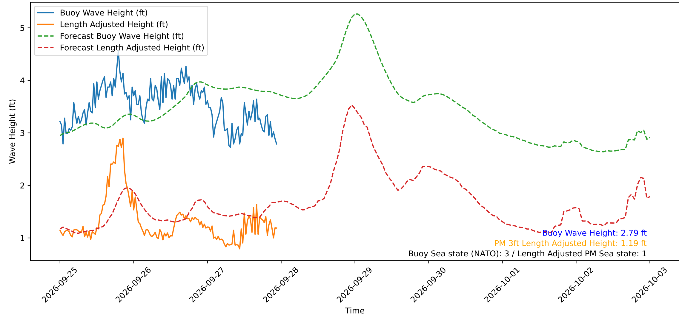
Wave Heights over Time for Green Beach at 2026-09-27 23:31:12
