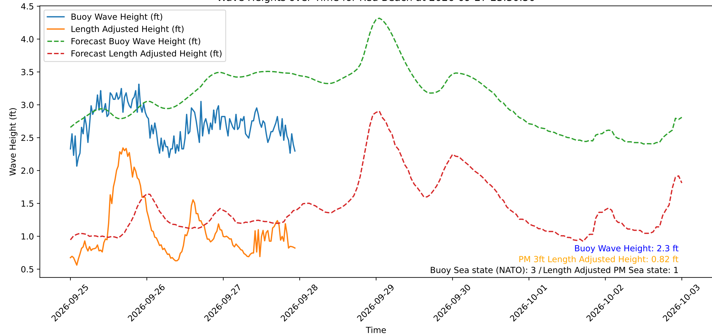
Wave Heights over Time for Red Beach at 2026-09-27 23:30:50
