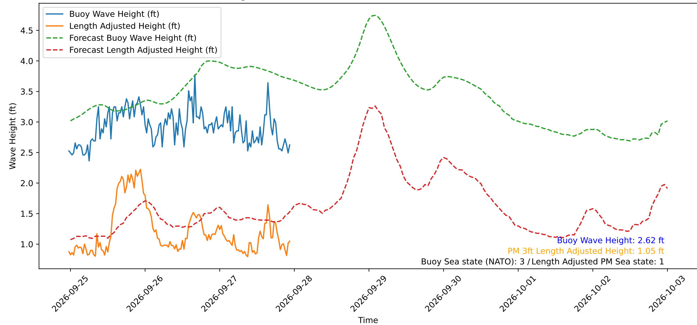
Wave Heights over Time for Oceanside Harbor at 2026-09-27 23:30:30
