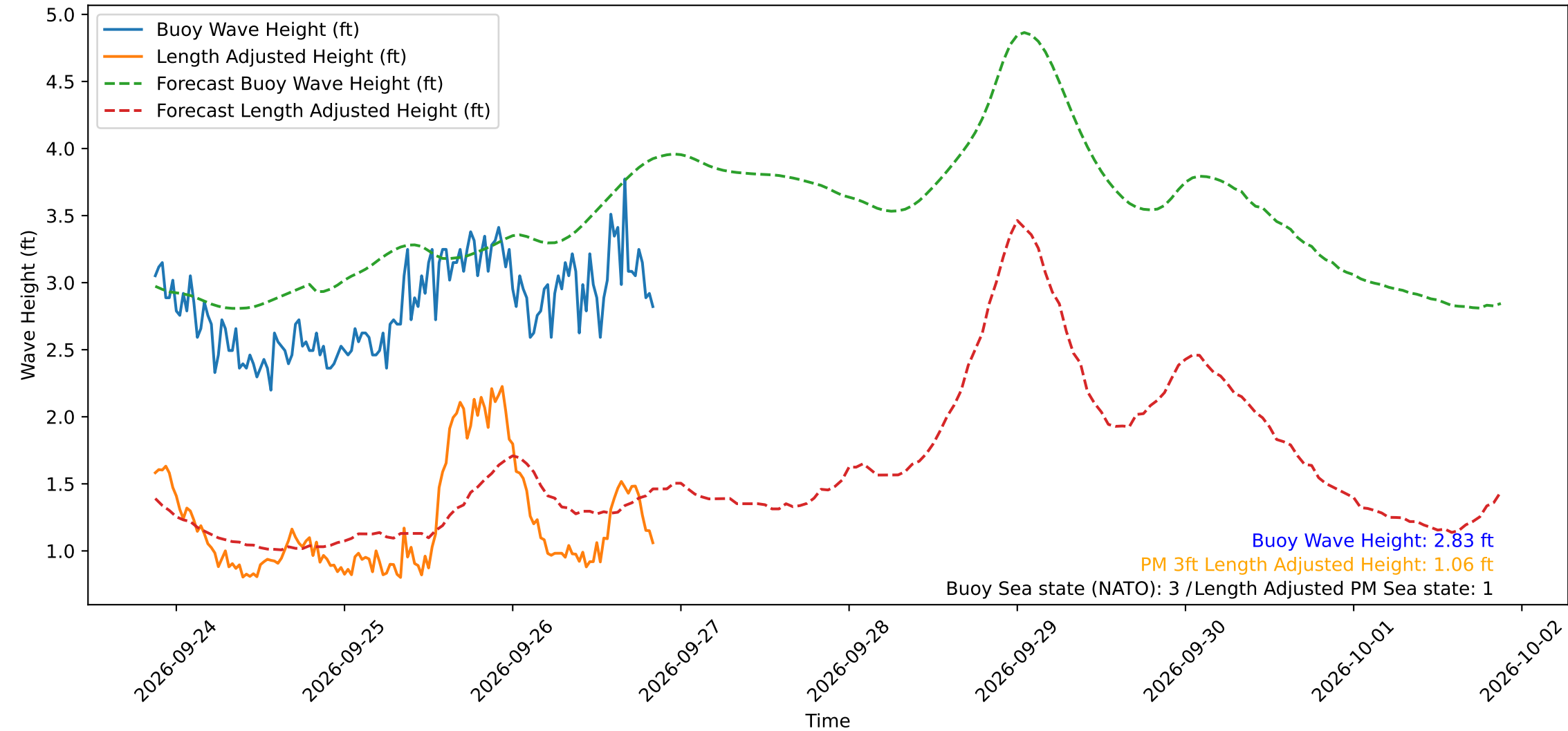
Wave Heights over Time for Oceanside Harbor at 2026-09-26 20:50:30
