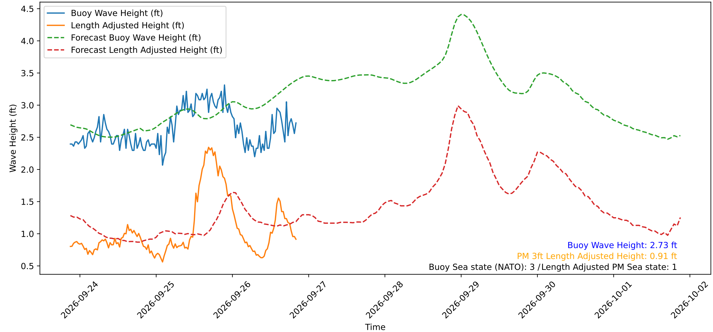
Wave Heights over Time for Red Beach at 2026-09-26 20:50:51
