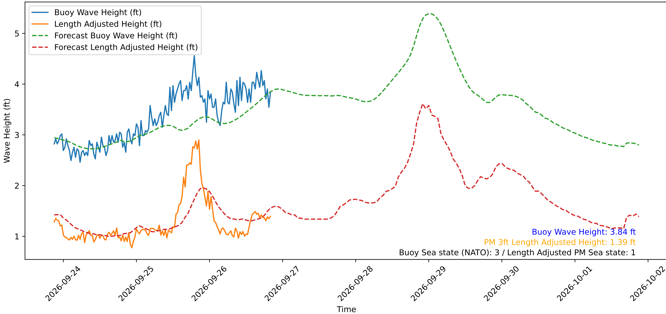
Wave Heights over Time for Green Beach at 2026-09-26 20:51:15
