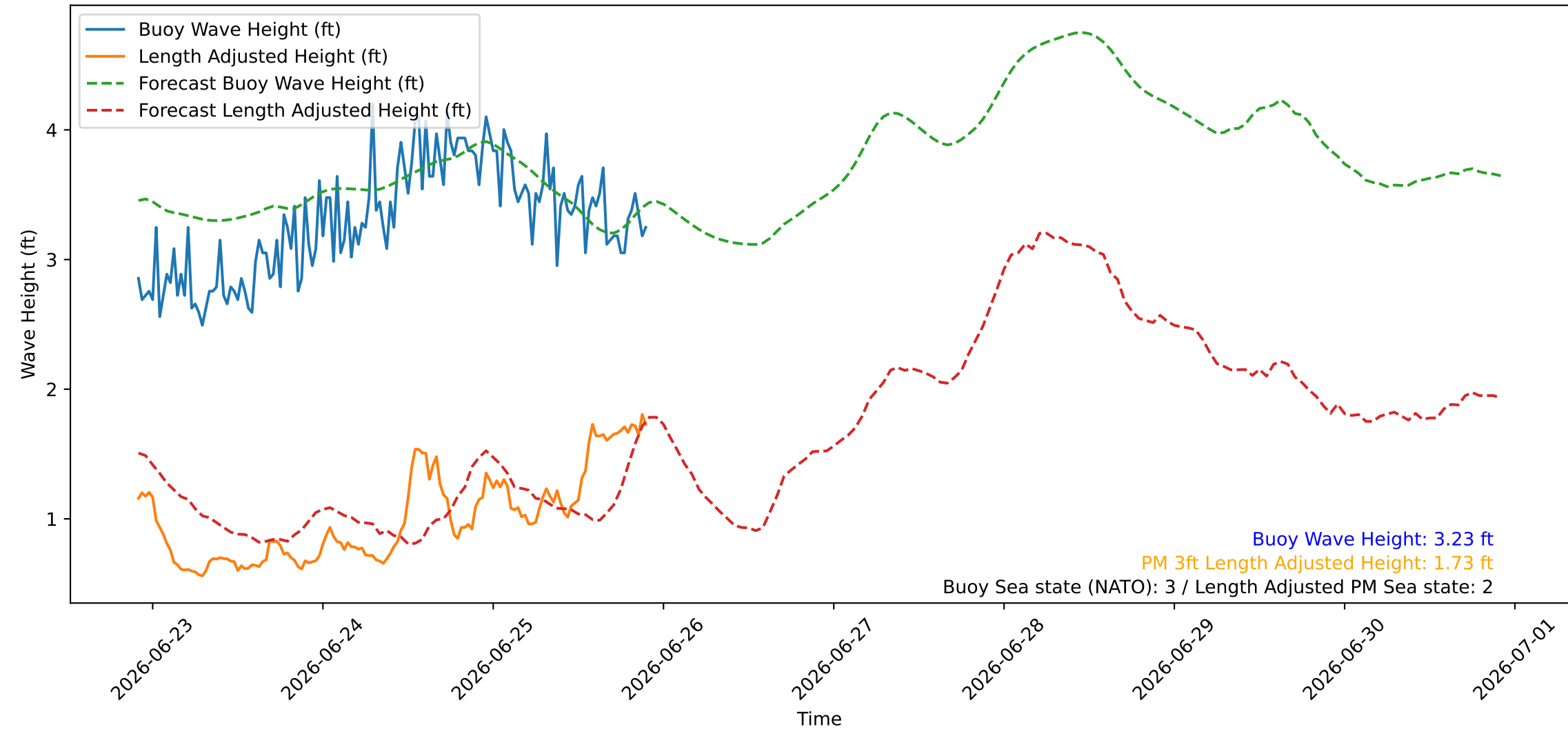
Wave Heights over Time for Green Beach at 2026-06-25 22:11:08
