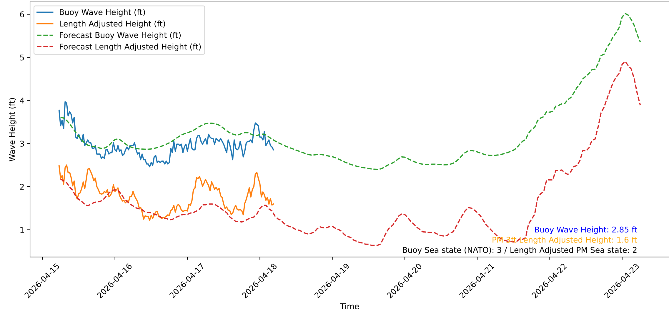
Wave Heights over Time for Green Beach at 2026-04-18 05:31:12
