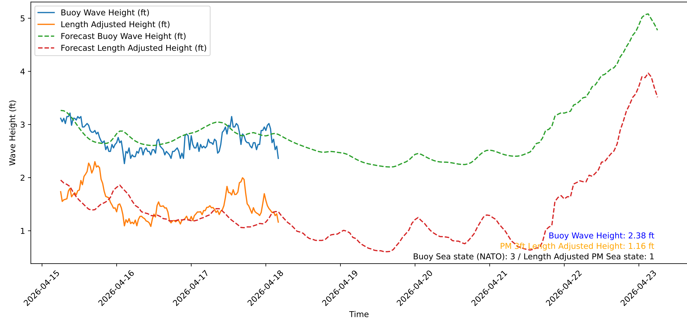
Wave Heights over Time for Red Beach at 2026-04-18 05:30:50
