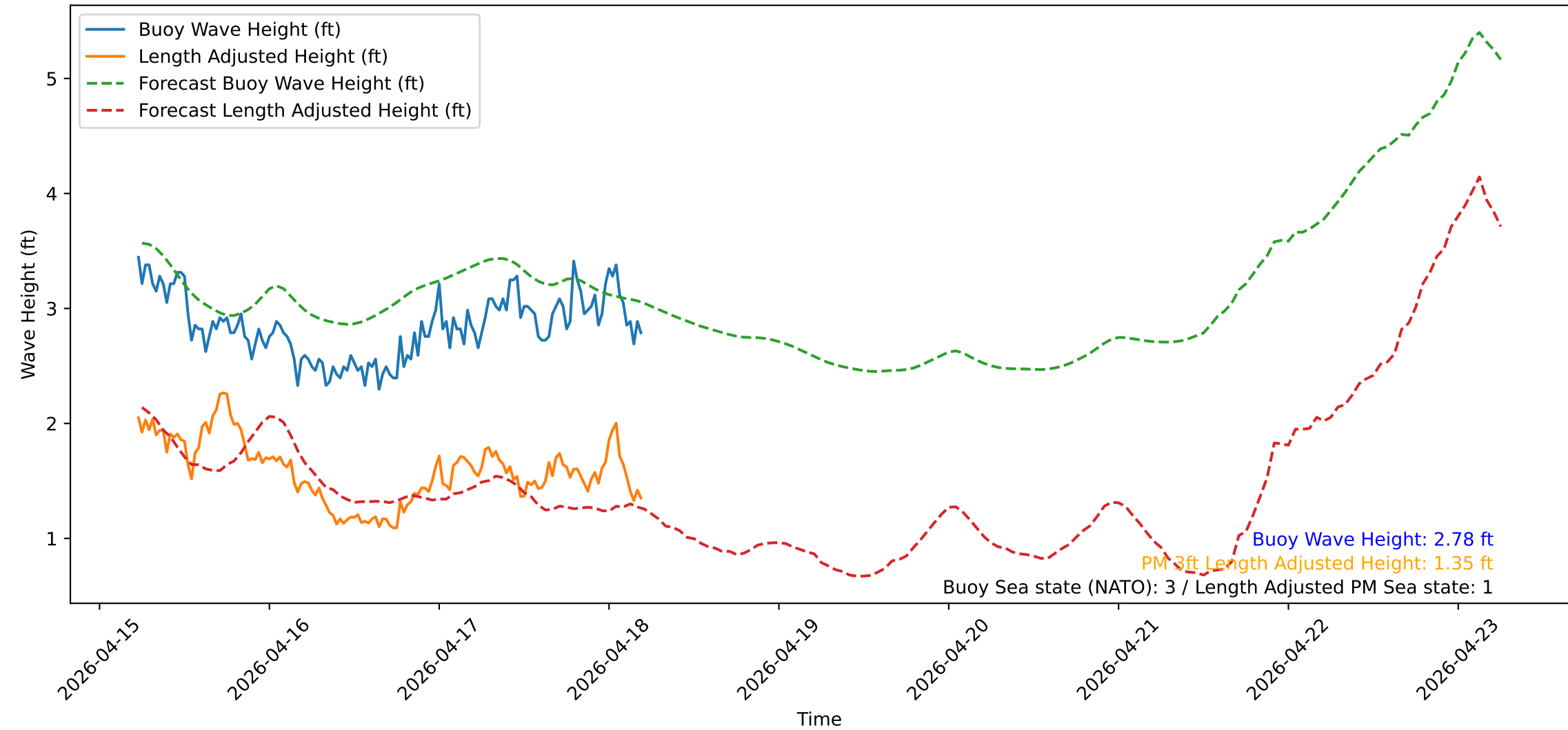
Wave Heights over Time for Oceanside Harbor at 2026-04-18 05:30:31
