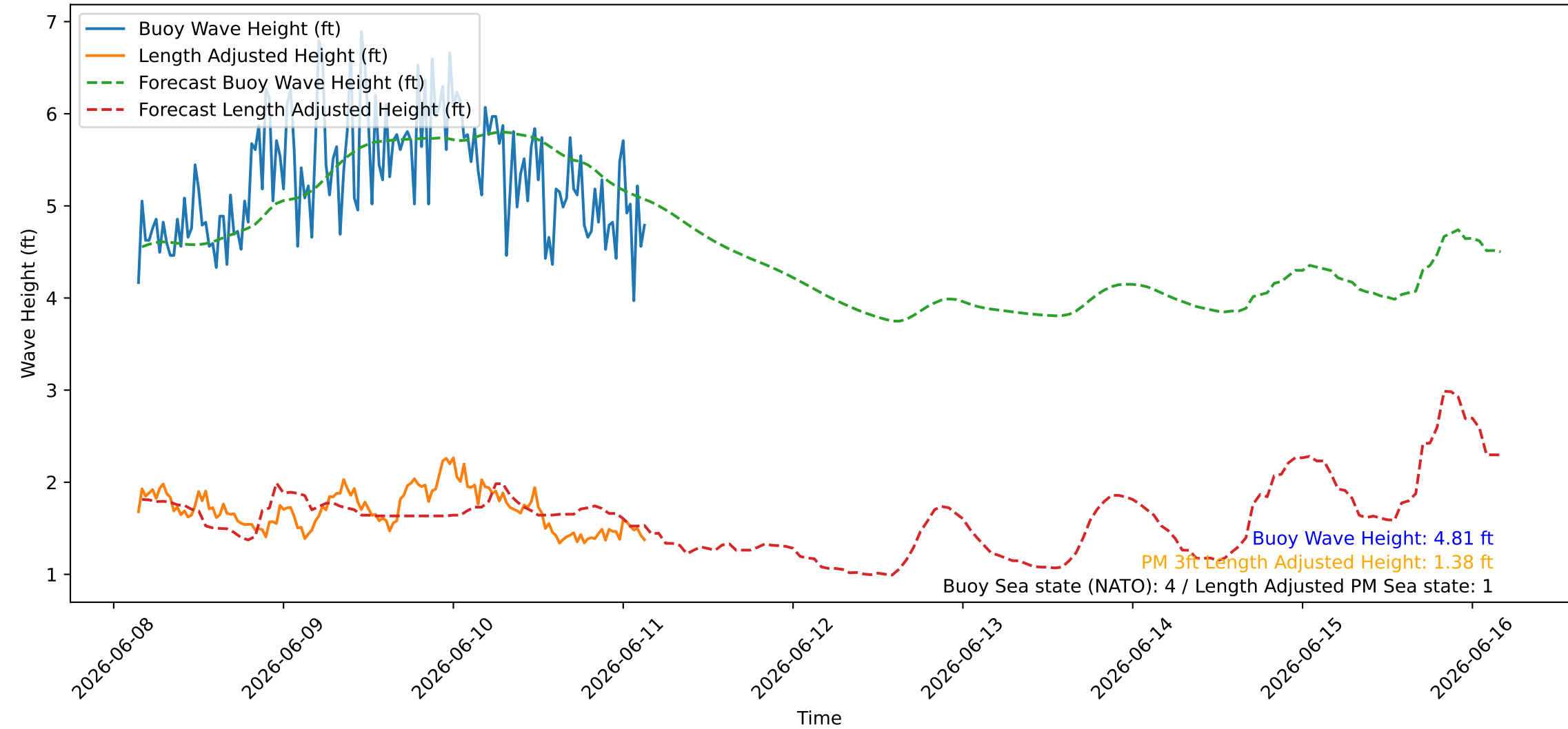
Wave Heights over Time for Green Beach at 2026-06-11 03:41:10
