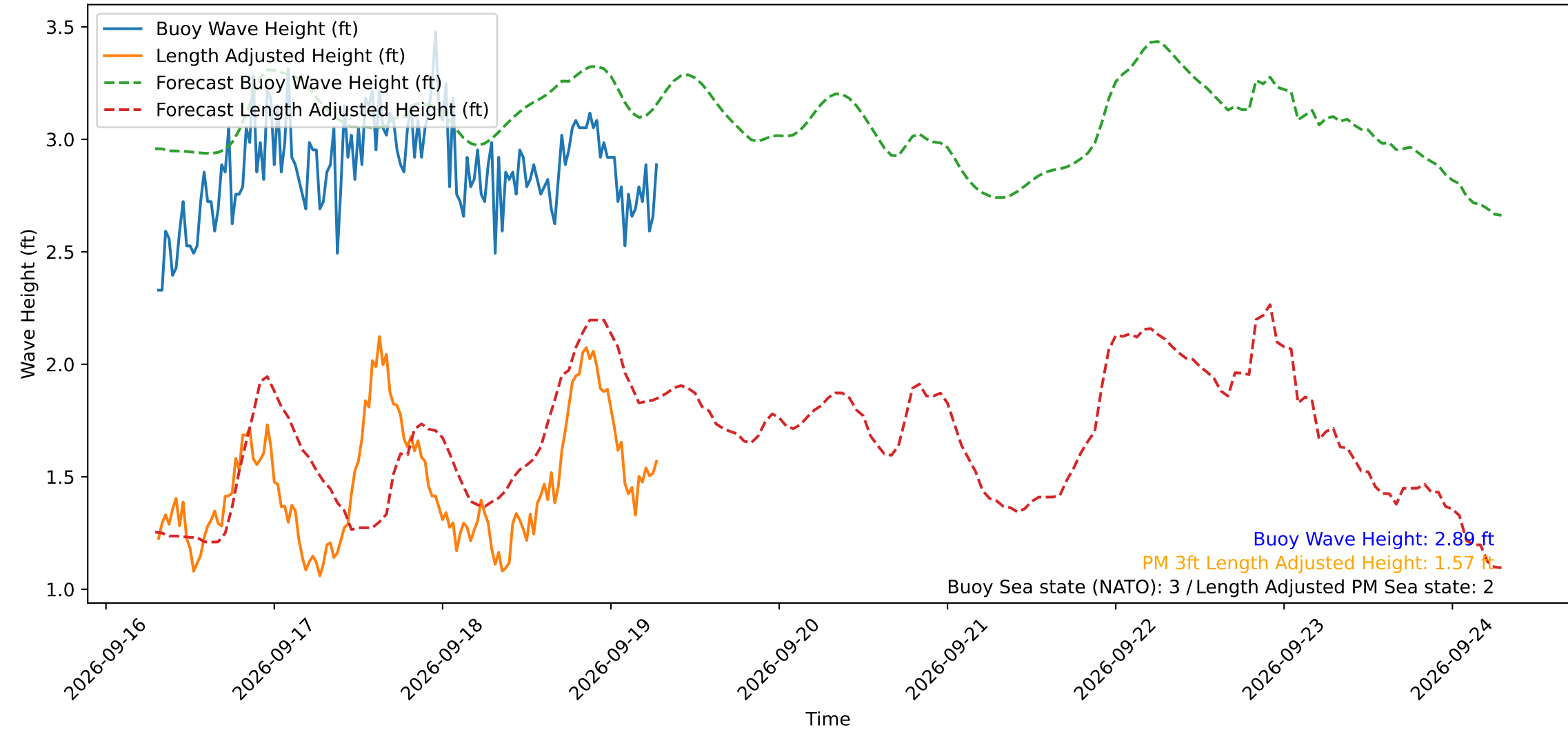
Wave Heights over Time for Green Beach at 2026-09-19 07:11:11
