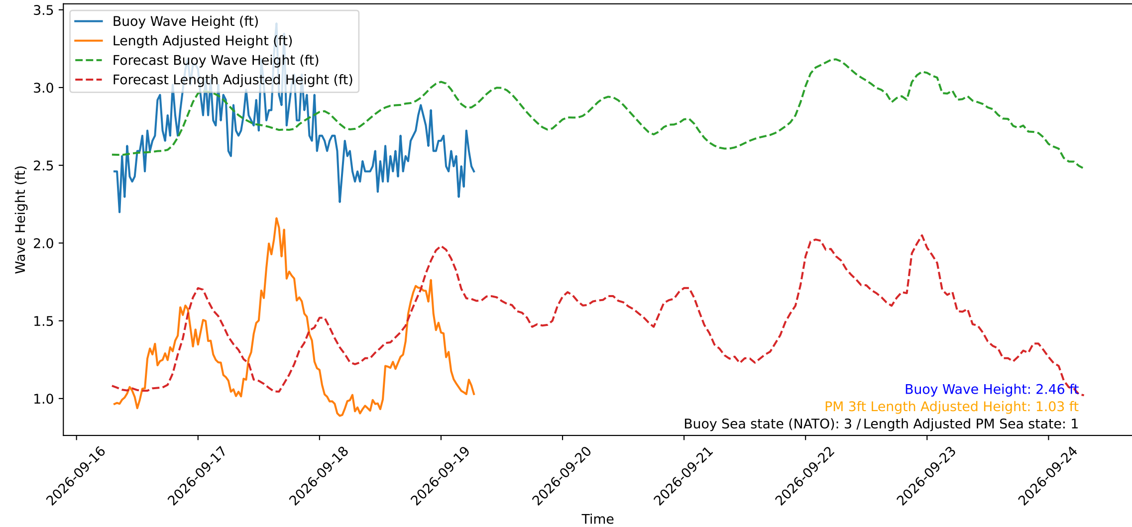
Wave Heights over Time for Red Beach at 2026-09-19 07:10:48
