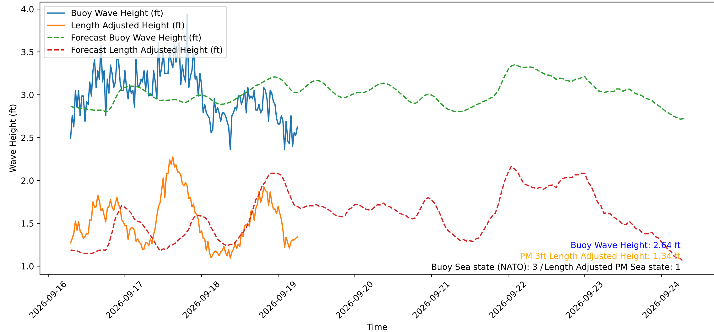
Wave Heights over Time for Oceanside Harbor at 2026-09-19 07:10:29
