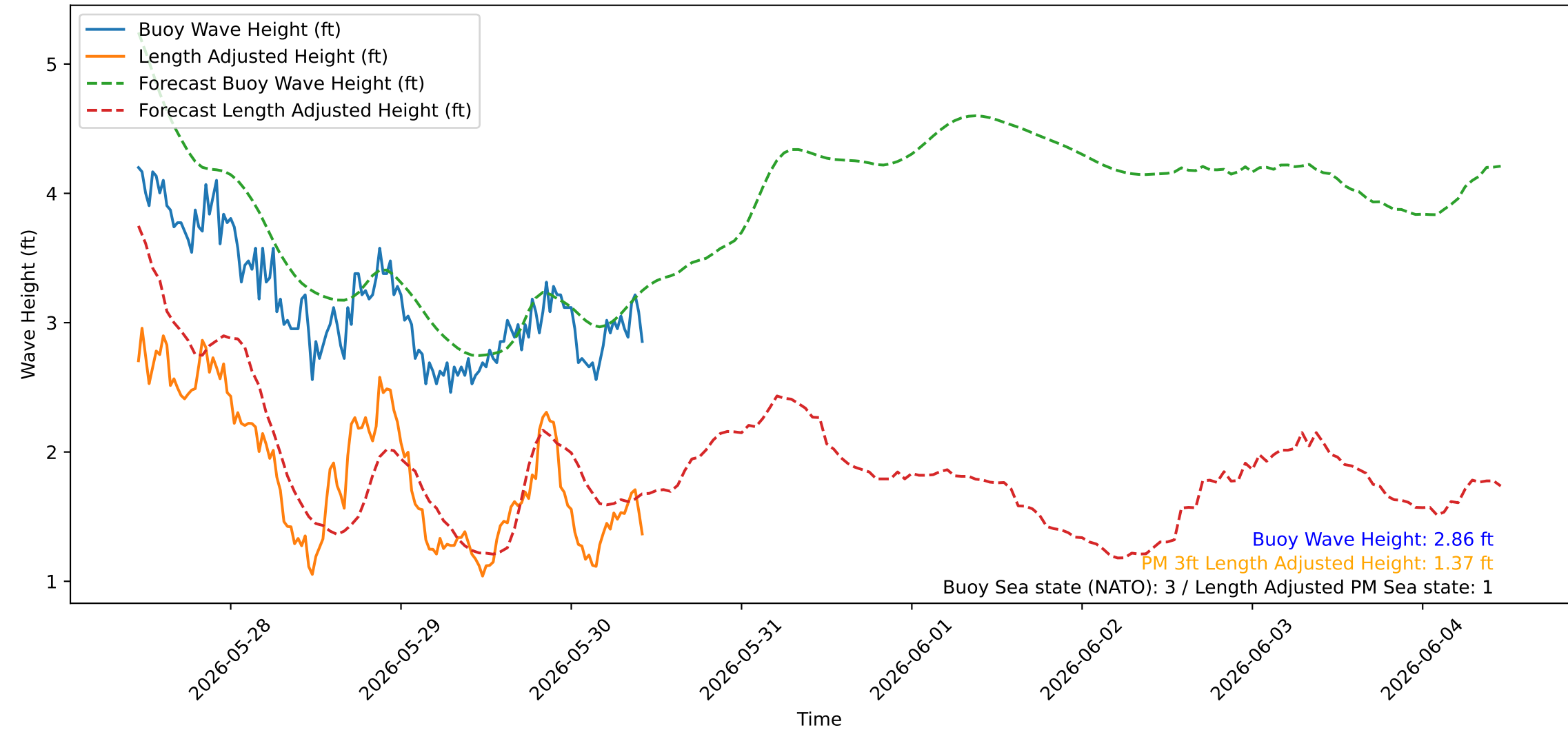
Wave Heights over Time for Green Beach at 2026-05-30 10:51:06
