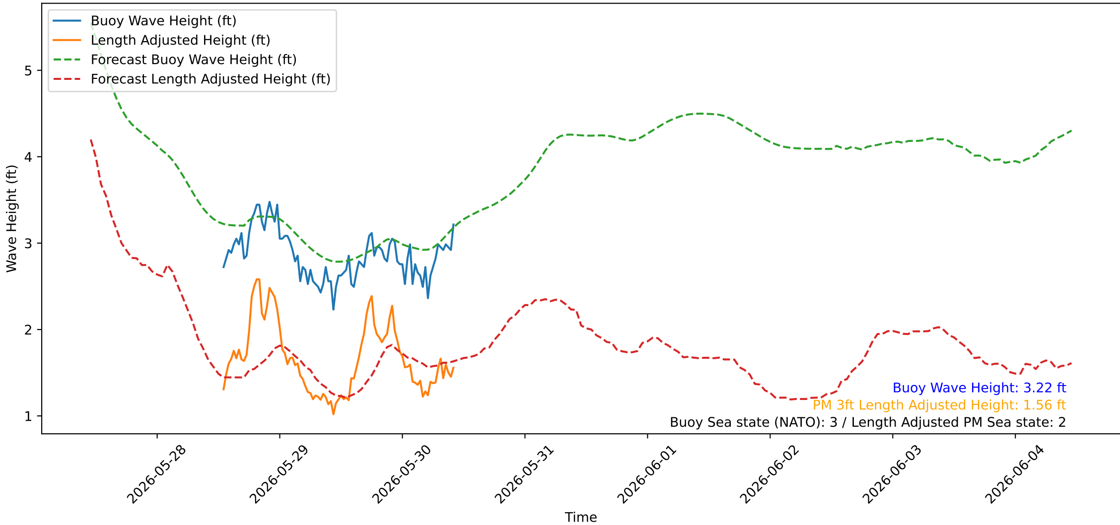
Wave Heights over Time for Oceanside Harbor at 2026-05-30 10:50:23
