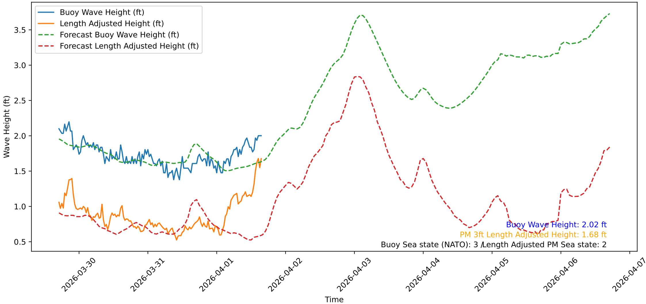
Wave Heights over Time for Red Beach at 2026-04-01 16:30:47
