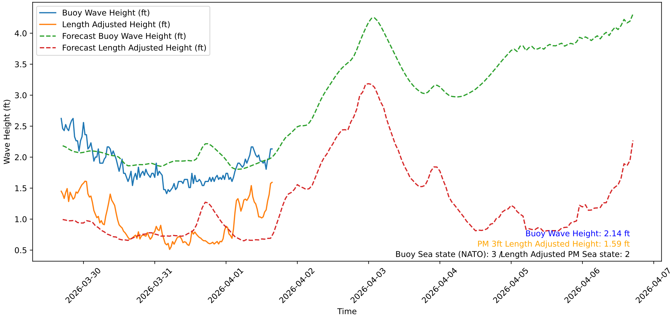
Wave Heights over Time for Green Beach at 2026-04-01 16:31:10
