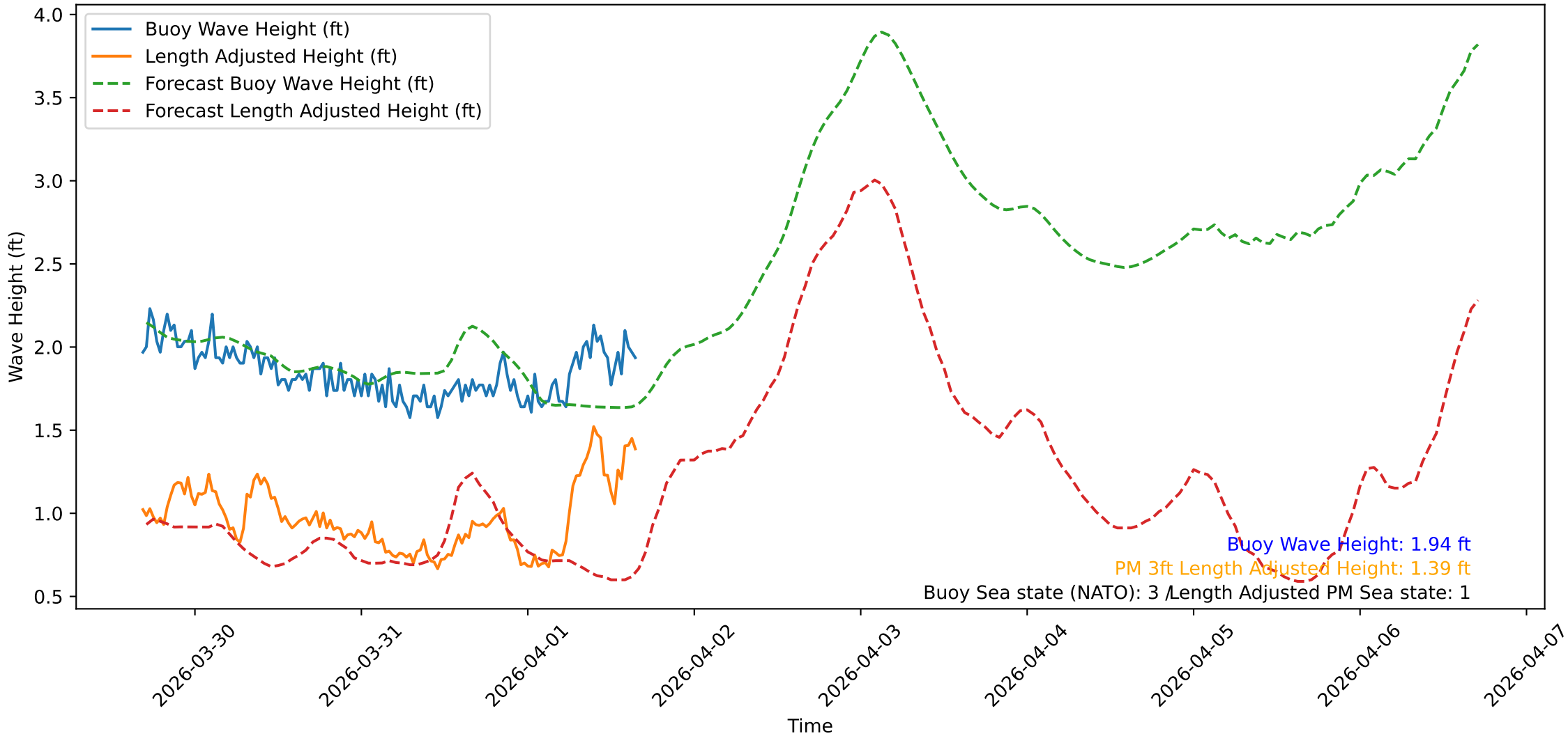
Wave Heights over Time for Oceanside Harbor at 2026-04-01 16:30:30
