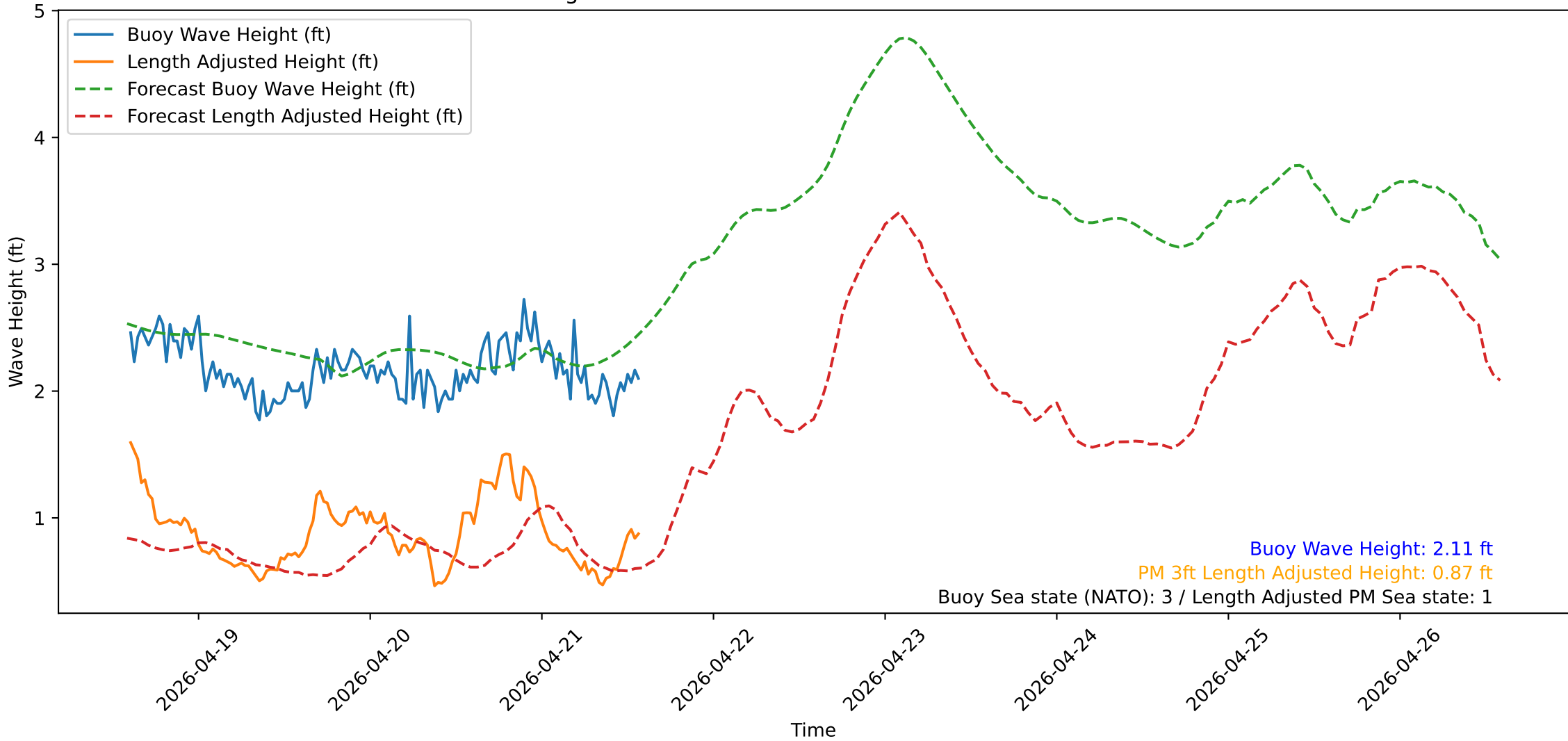
Wave Heights over Time for Red Beach at 2026-04-21 14:20:51
