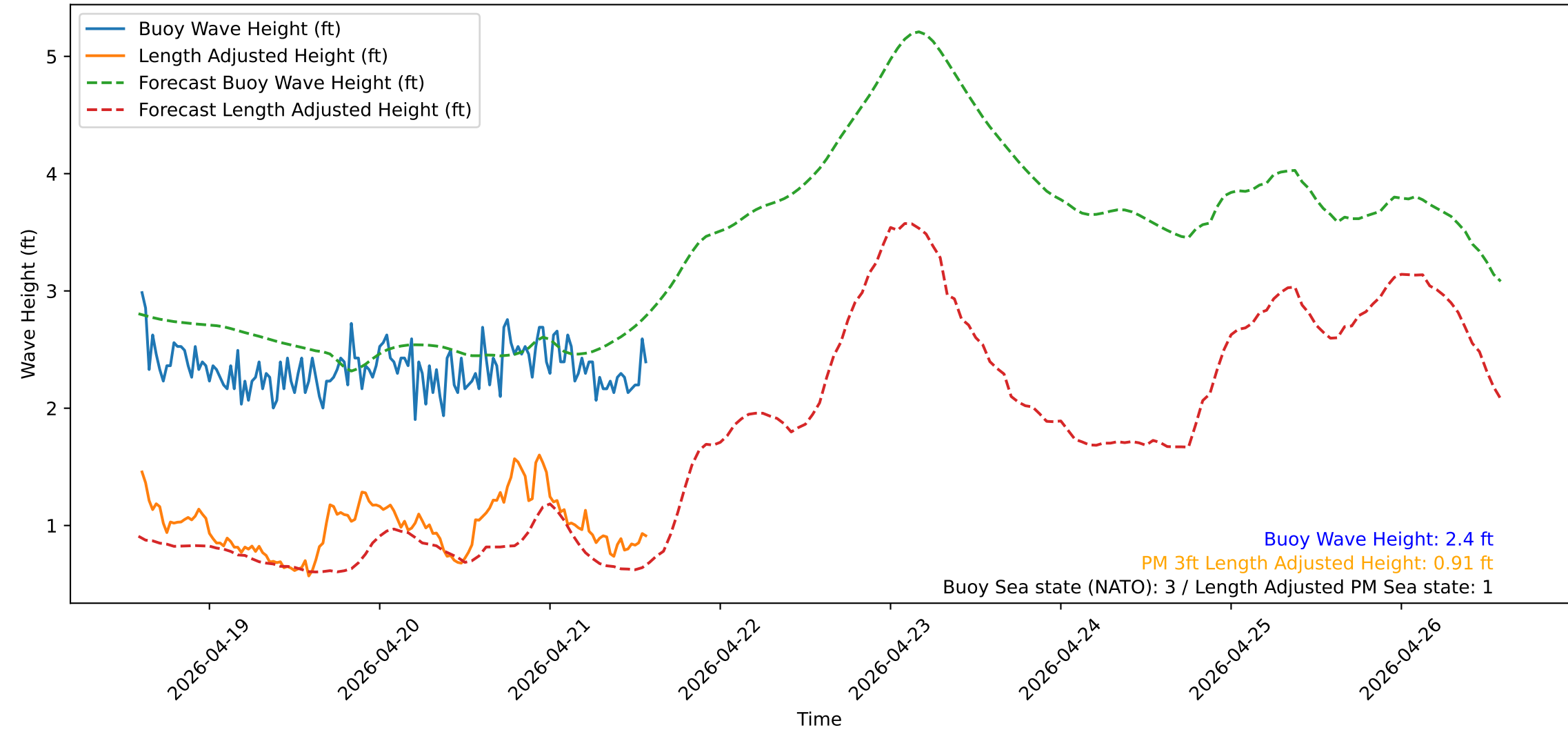
Wave Heights over Time for Oceanside Harbor at 2026-04-21 14:20:31
