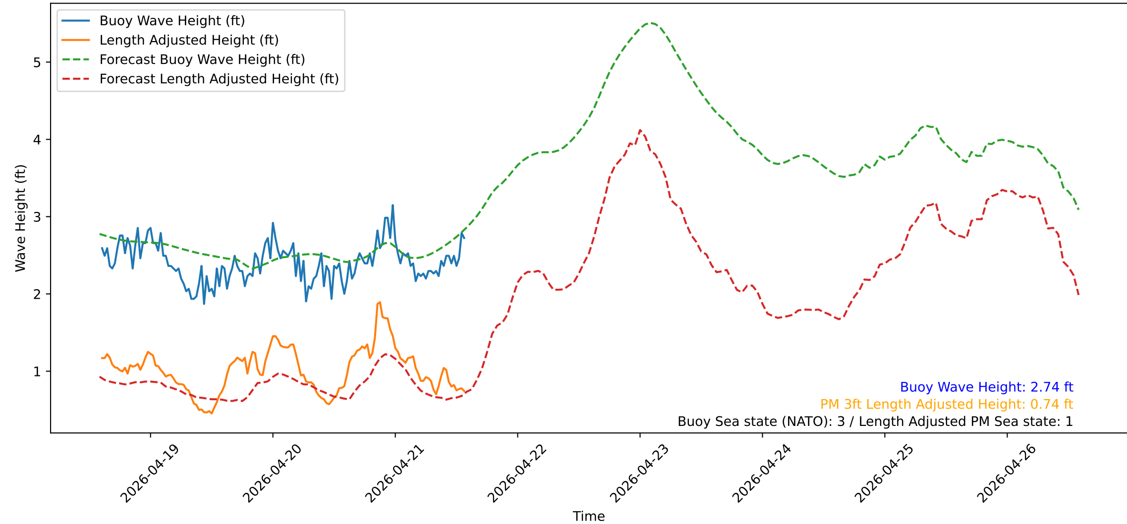
Wave Heights over Time for Green Beach at 2026-04-21 14:21:14
