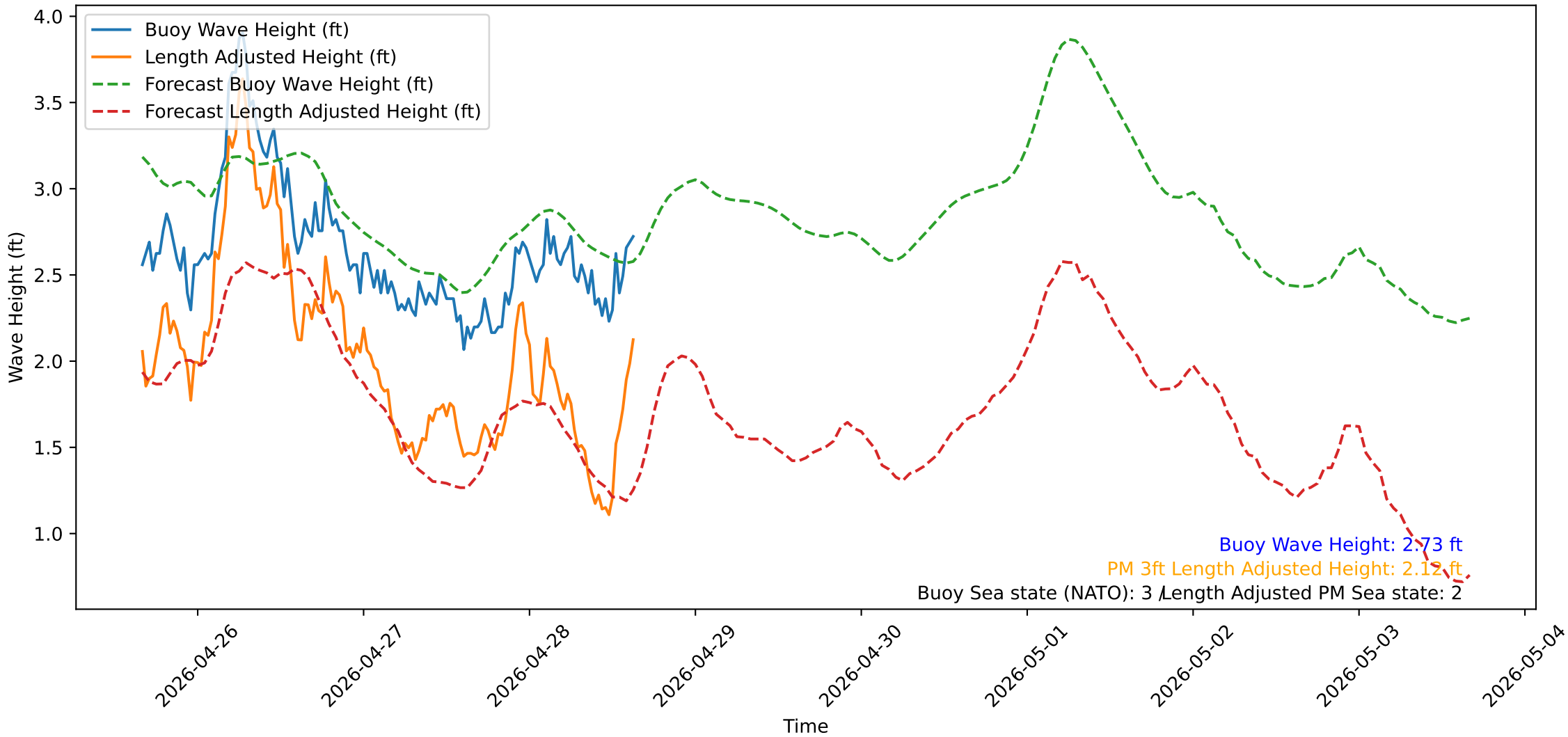
Wave Heights over Time for Oceanside Harbor at 2026-04-28 15:50:32
