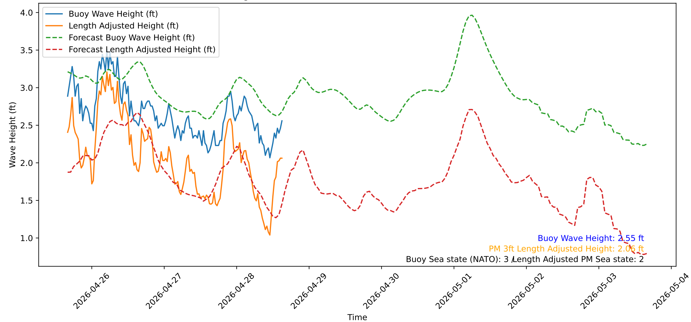
Wave Heights over Time for Green Beach at 2026-04-28 15:51:15
