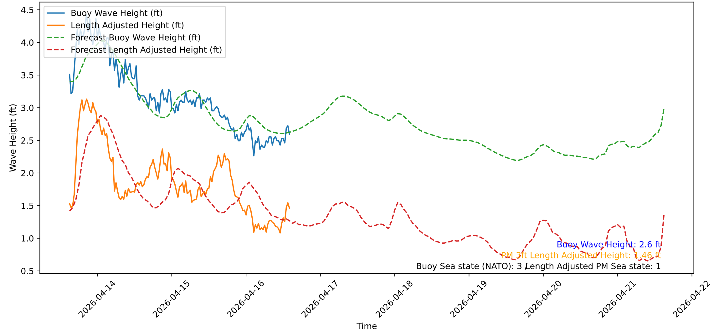
Wave Heights over Time for Red Beach at 2026-04-16 14:40:51
