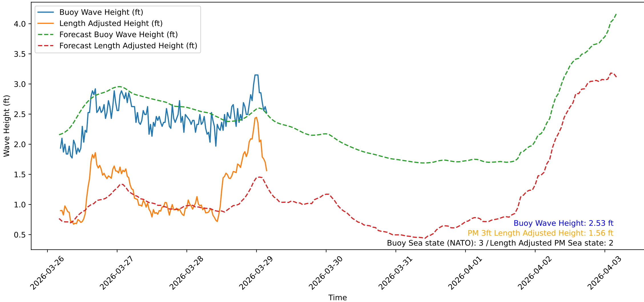
Wave Heights over Time for Oceanside Harbor at 2026-03-29 04:20:32
