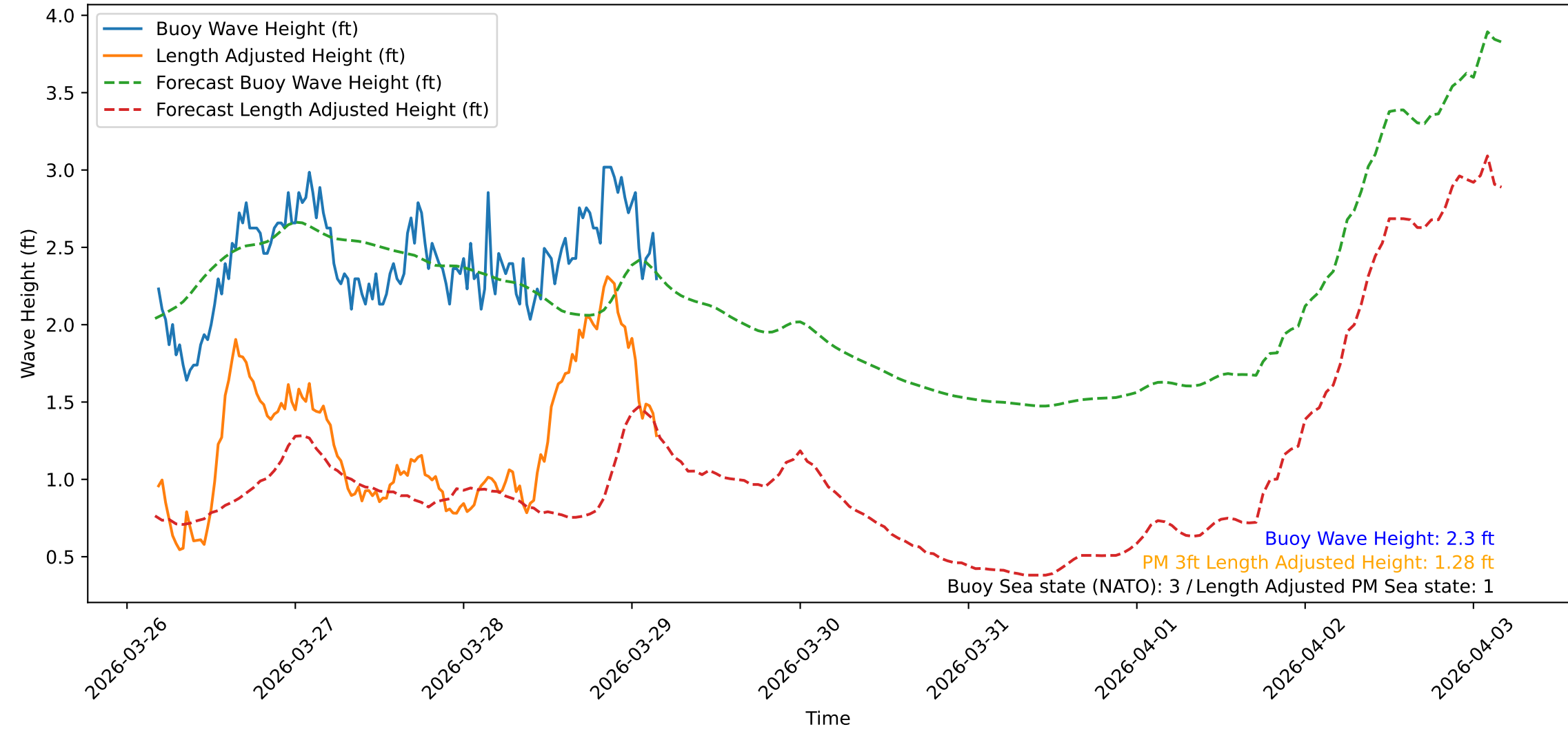
Wave Heights over Time for Red Beach at 2026-03-29 04:20:47
