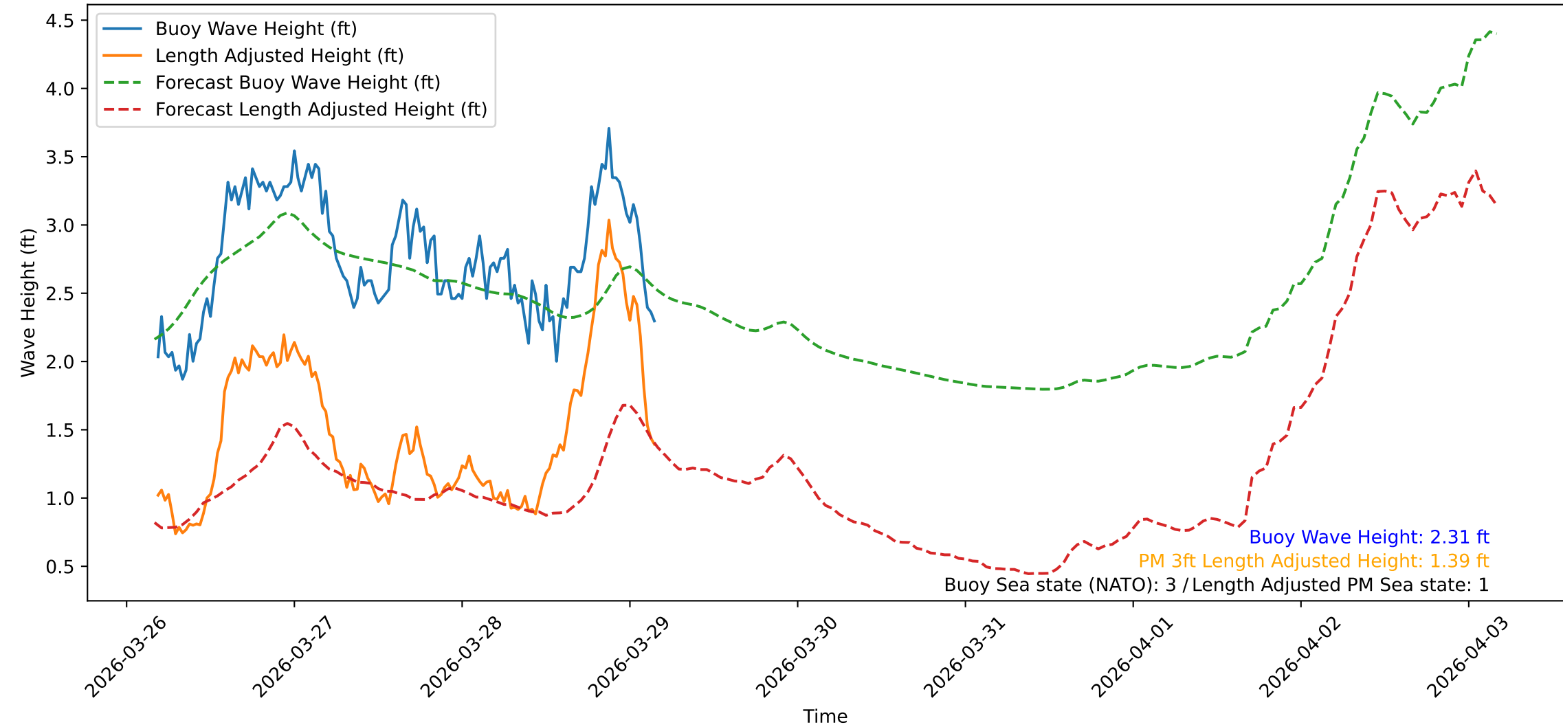
Wave Heights over Time for Green Beach at 2026-03-29 04:21:09
