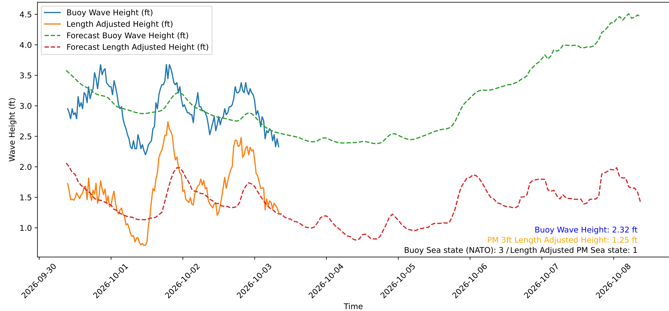
Wave Heights over Time for Green Beach at 2026-10-03 09:01:11
