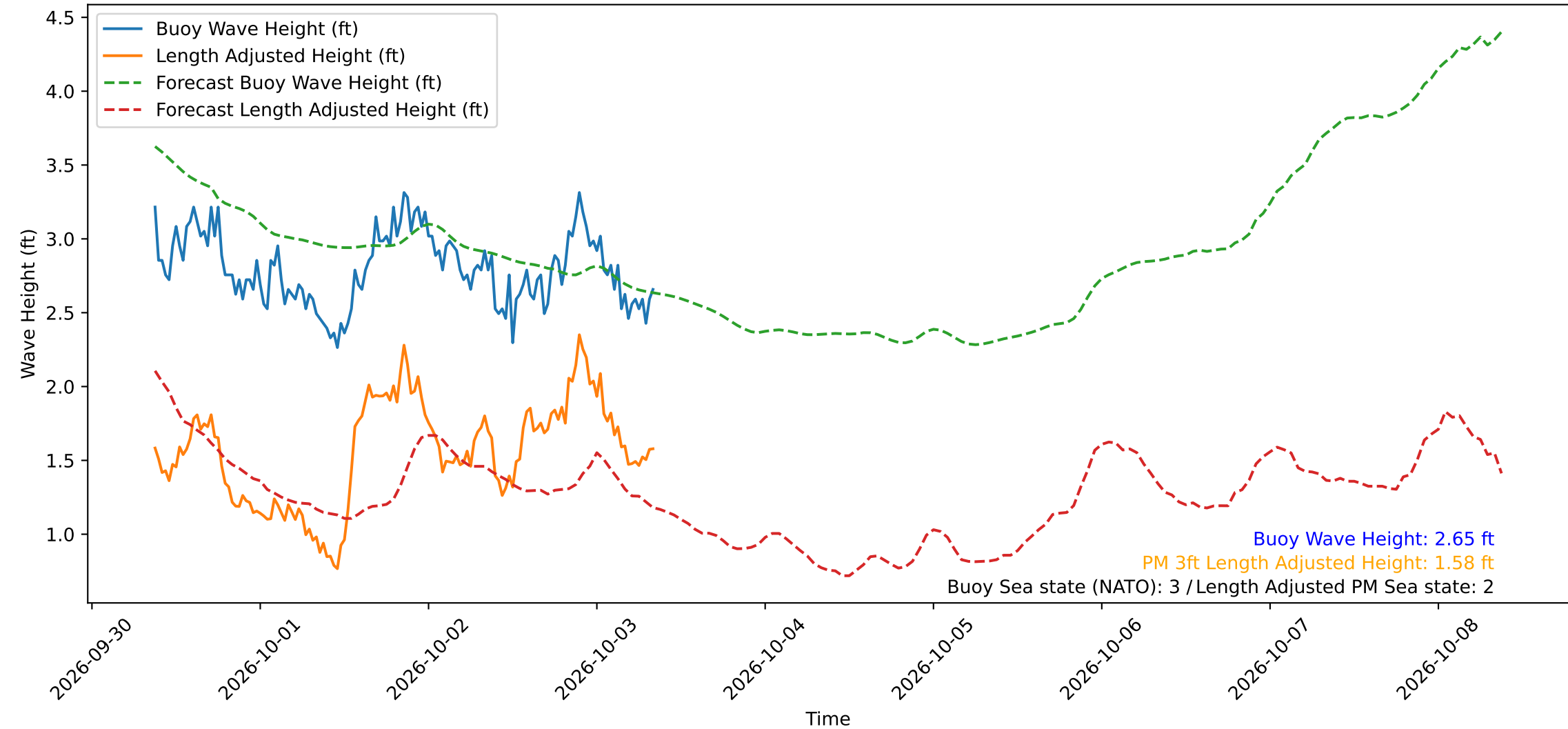
Wave Heights over Time for Oceanside Harbor at 2026-10-03 09:00:29
