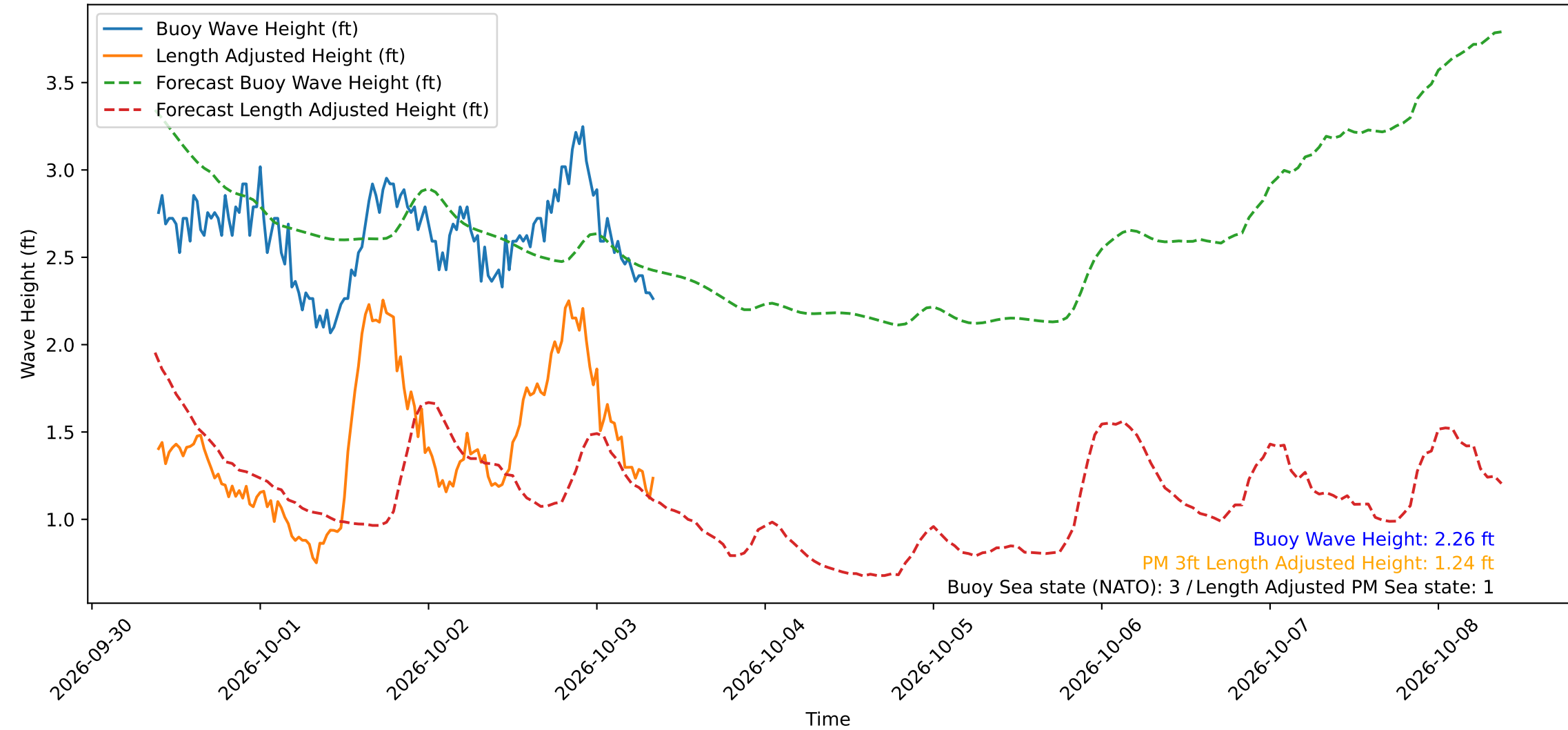
Wave Heights over Time for Red Beach at 2026-10-03 09:00:49
