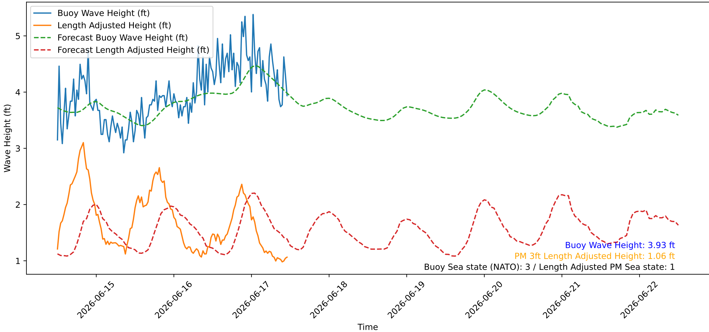
Wave Heights over Time for Red Beach at 2026-06-17 11:40:45
