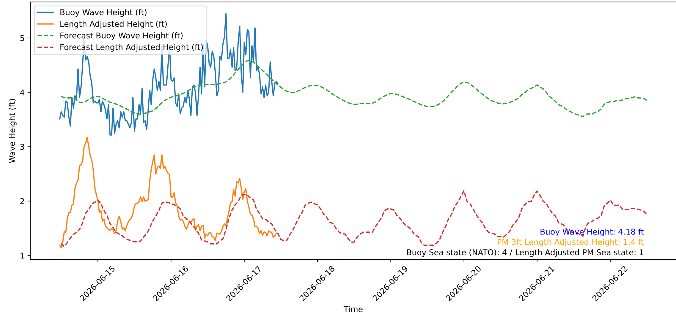
Wave Heights over Time for Oceanside Harbor at 2026-06-17 11:40:26
