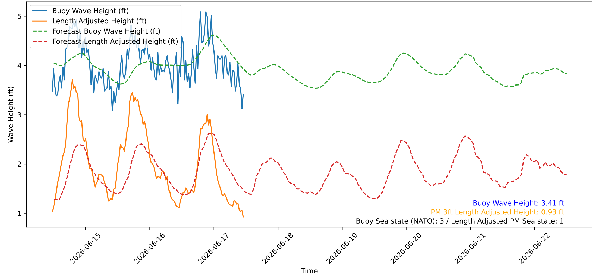
Wave Heights over Time for Green Beach at 2026-06-17 11:41:09
