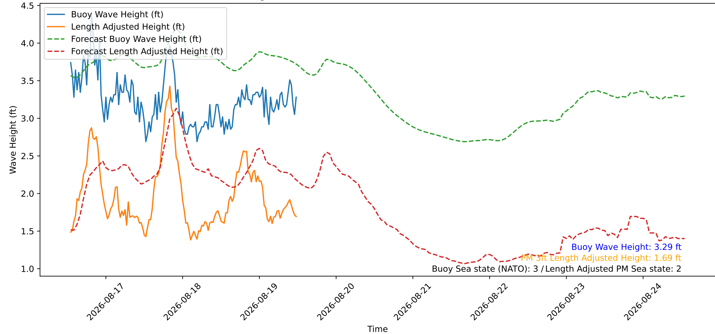
Wave Heights over Time for Green Beach at 2026-08-19 12:31:10
