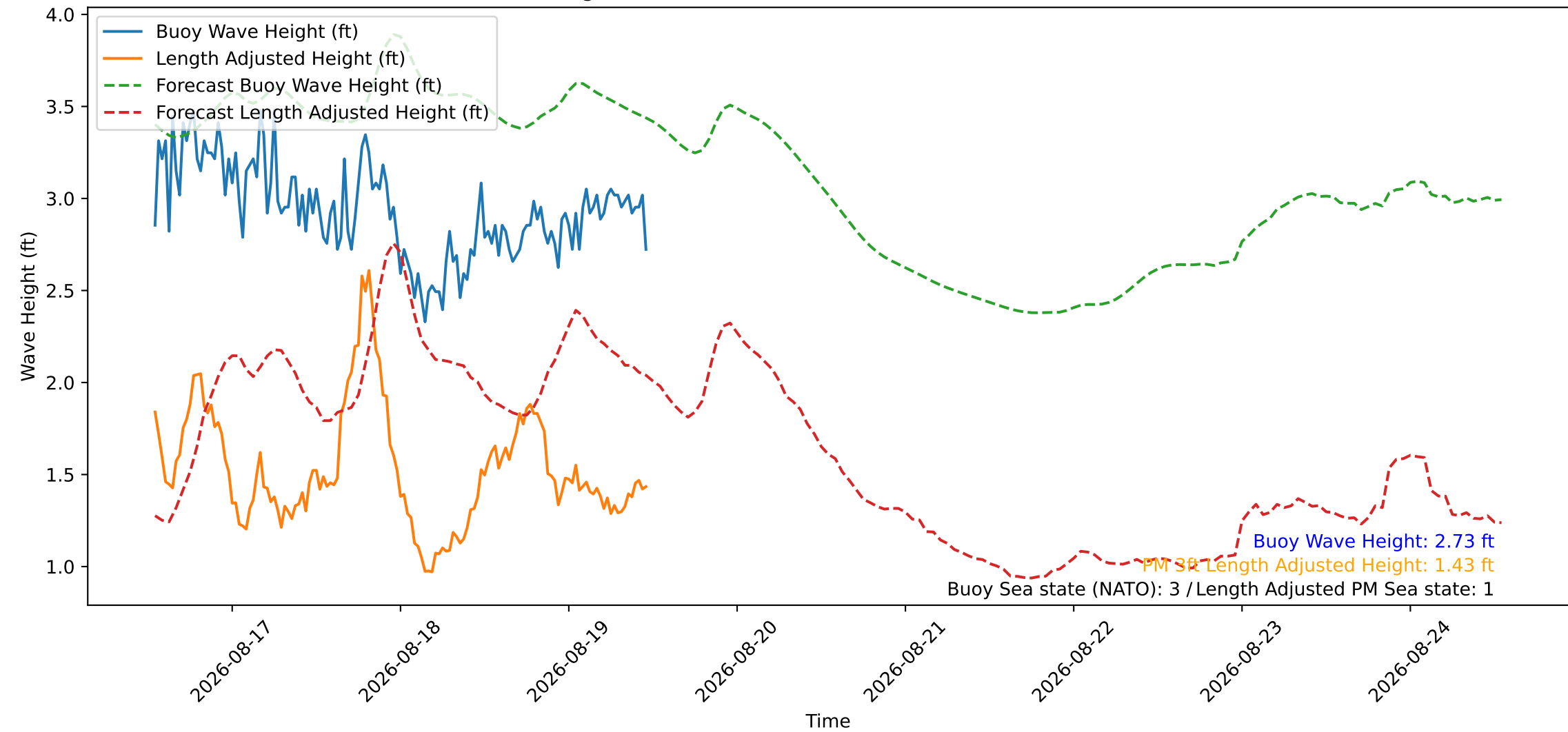
Wave Heights over Time for Red Beach at 2026-08-19 12:30:47
