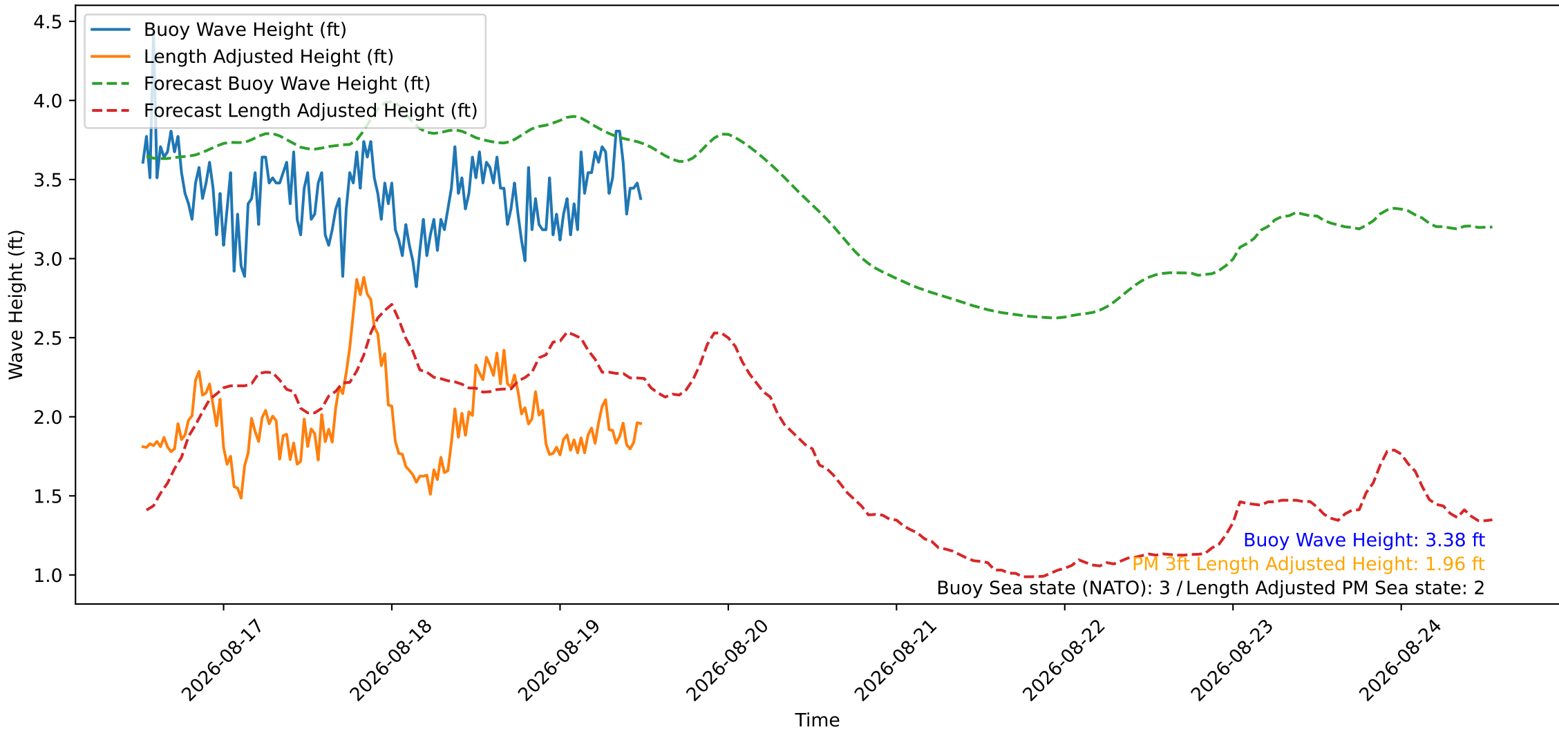
Wave Heights over Time for Oceanside Harbor at 2026-08-19 12:30:27
