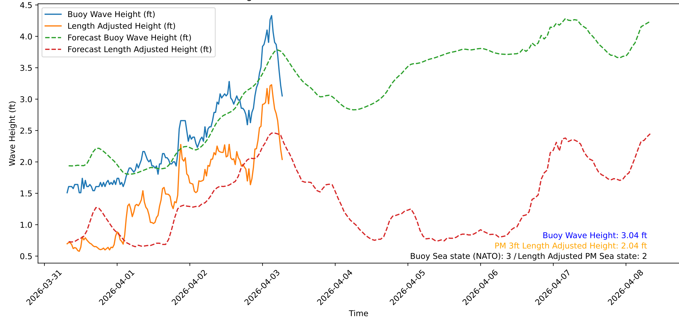
Wave Heights over Time for Green Beach at 2026-04-03 07:31:11
