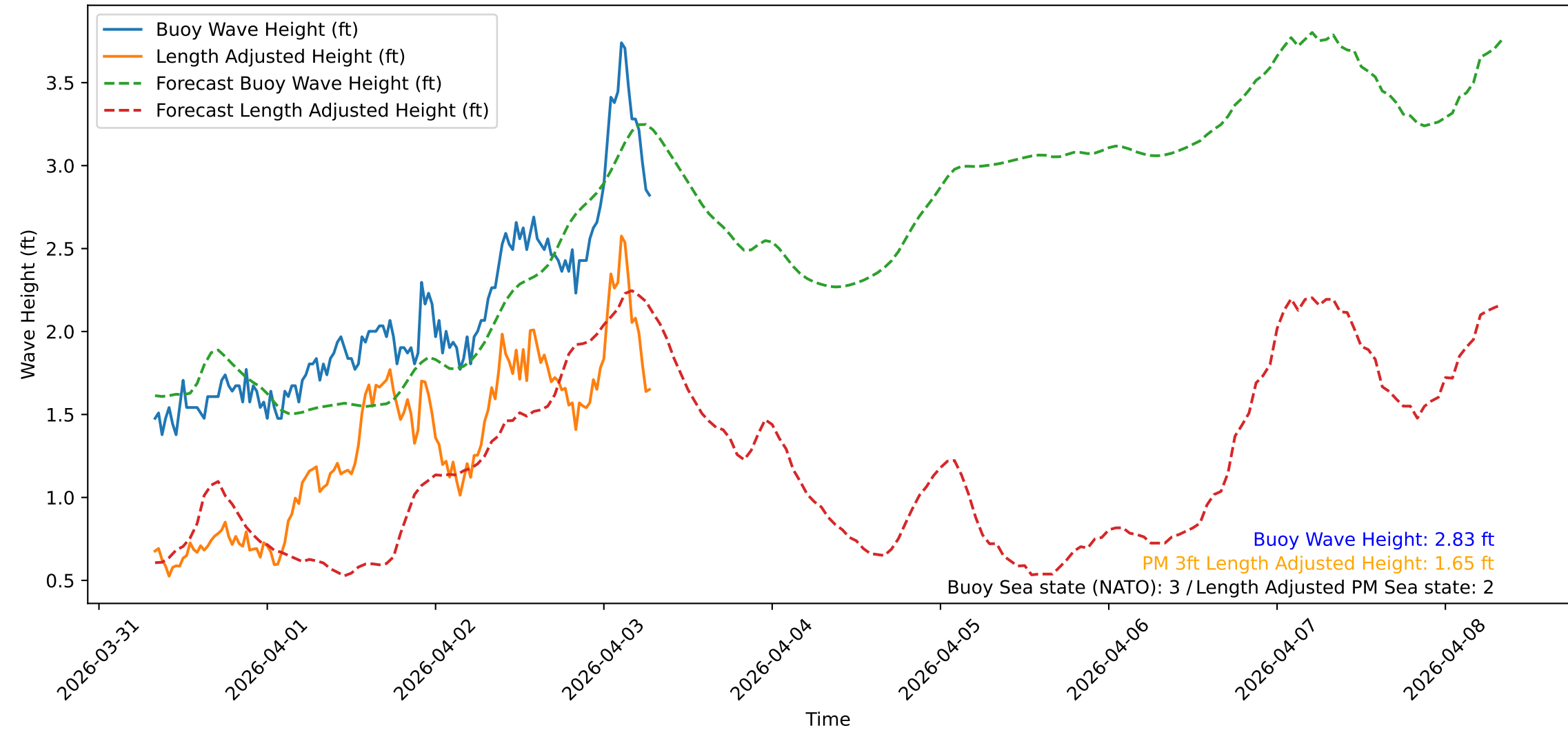
Wave Heights over Time for Red Beach at 2026-04-03 07:30:48
