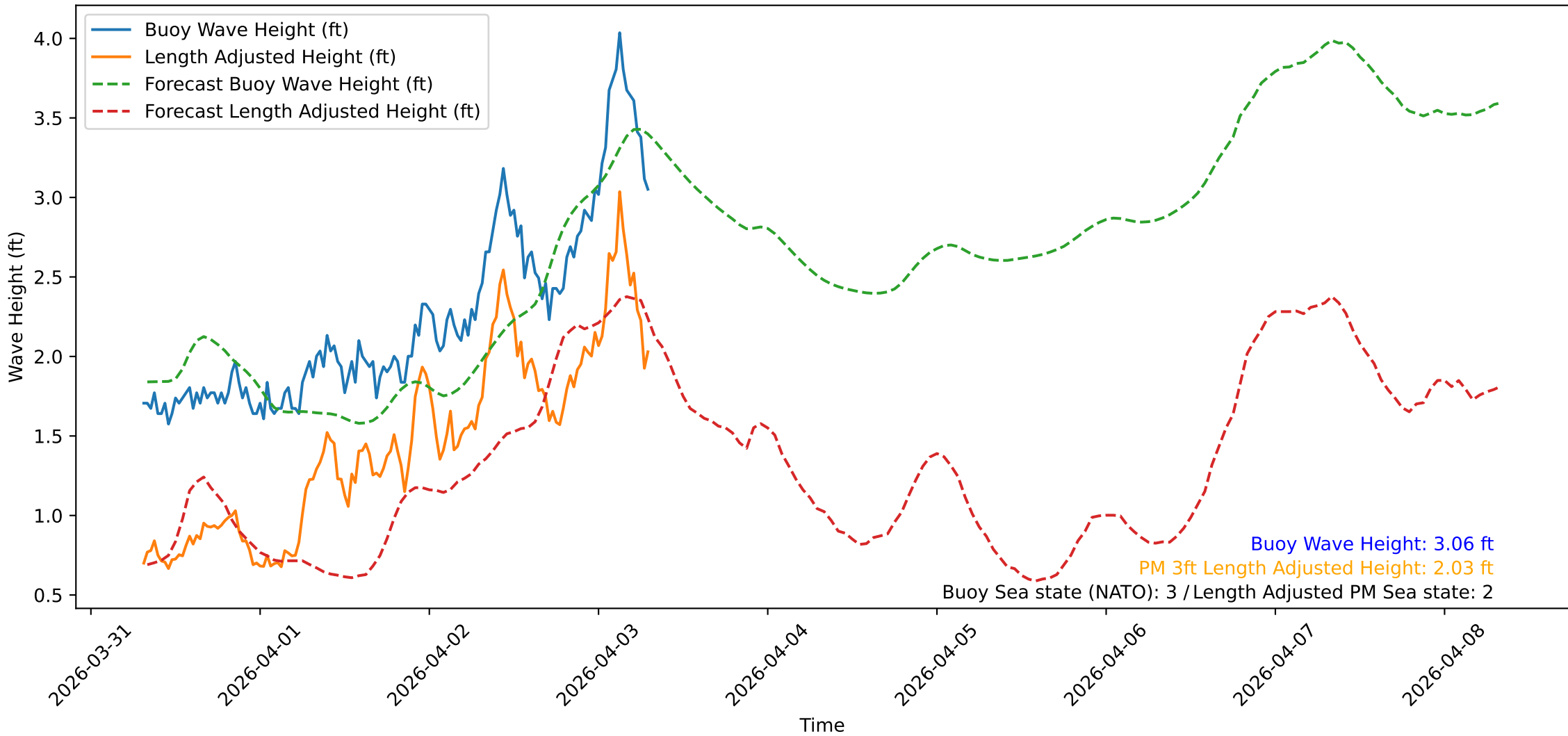
Wave Heights over Time for Oceanside Harbor at 2026-04-03 07:30:32
