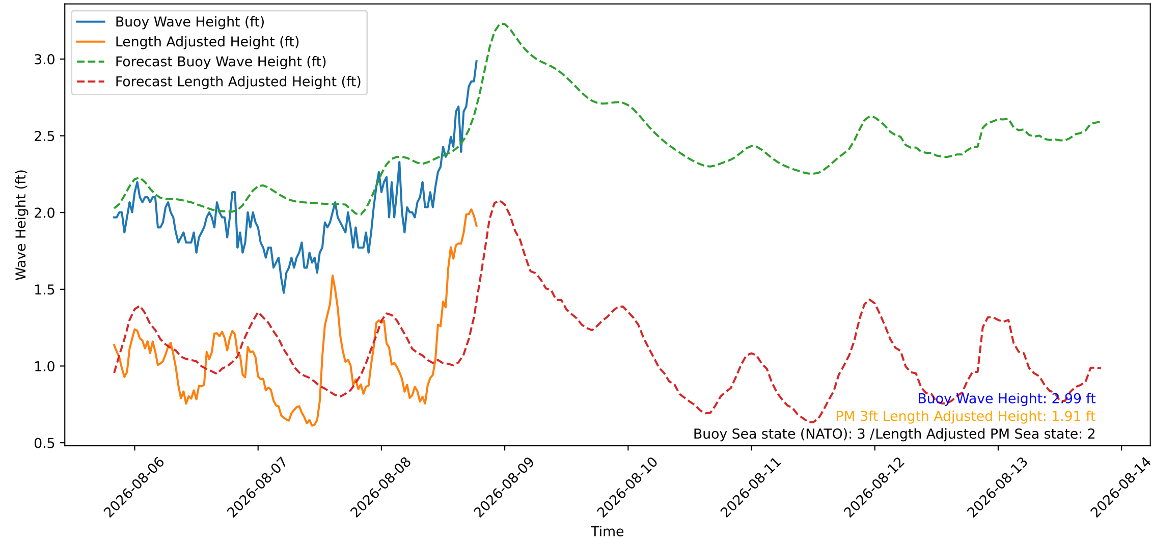
Wave Heights over Time for Red Beach at 2026-08-08 19:50:48
