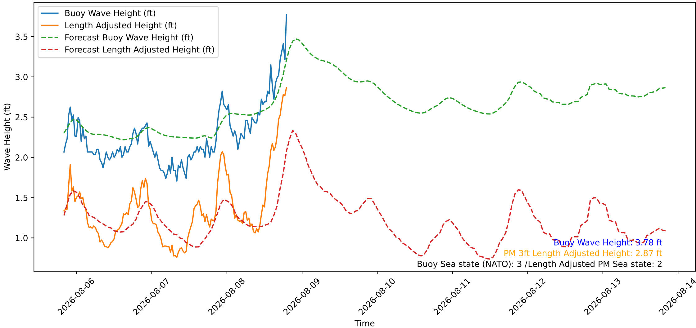
Wave Heights over Time for Green Beach at 2026-08-08 19:51:10
