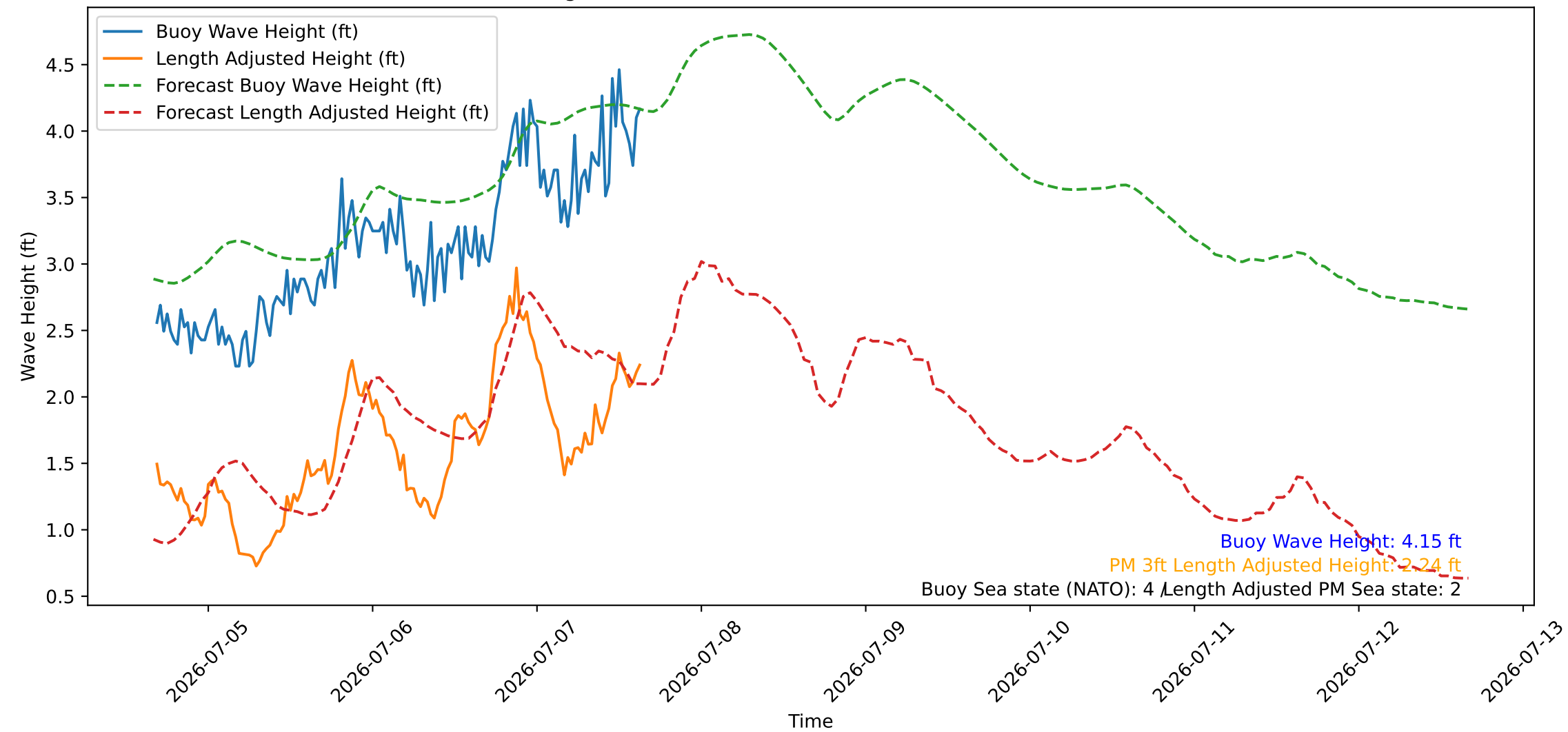
Wave Heights over Time for Red Beach at 2026-07-07 16:00:46
