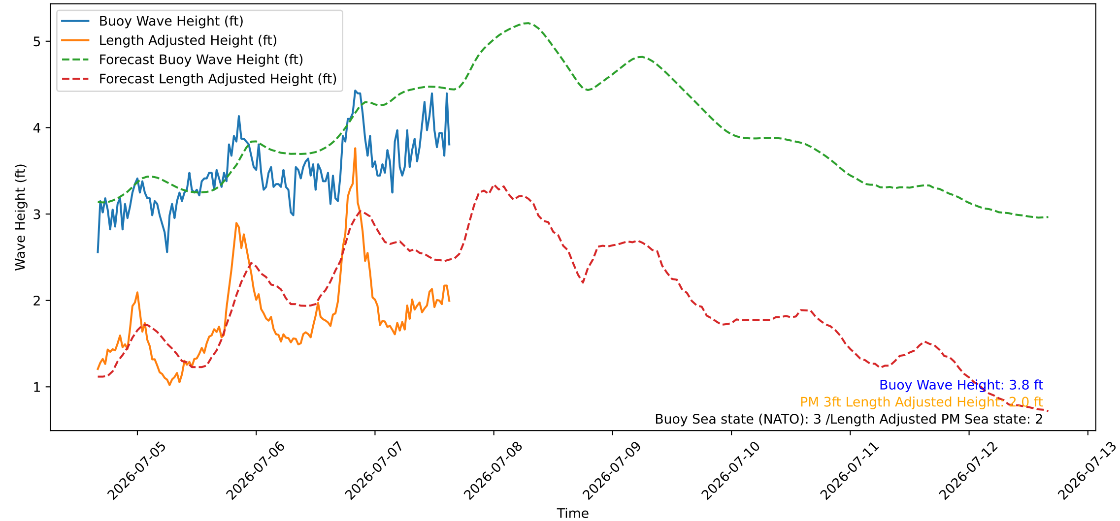
Wave Heights over Time for Green Beach at 2026-07-07 16:01:08
