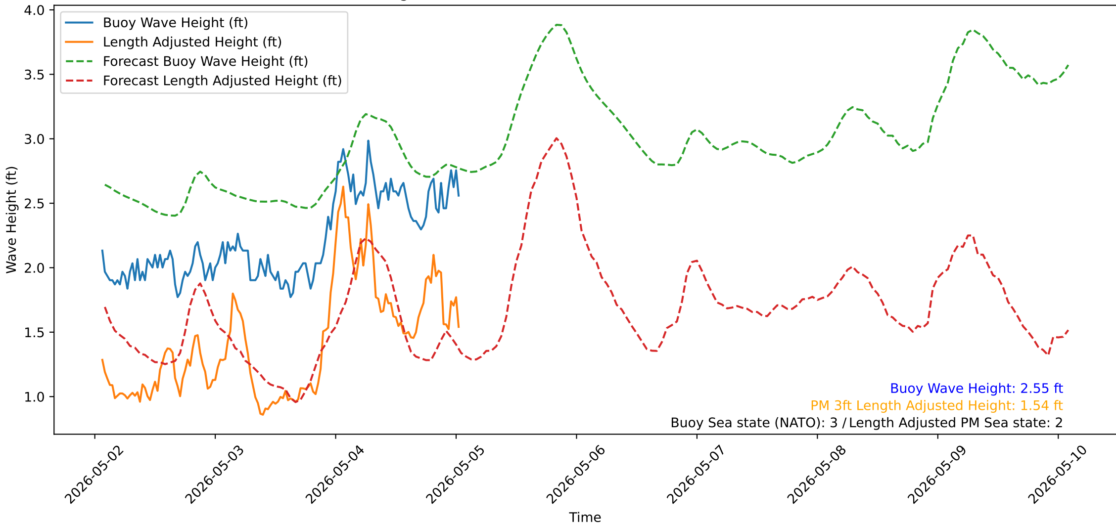
Wave Heights over Time for Green Beach at 2026-05-05 01:31:13
