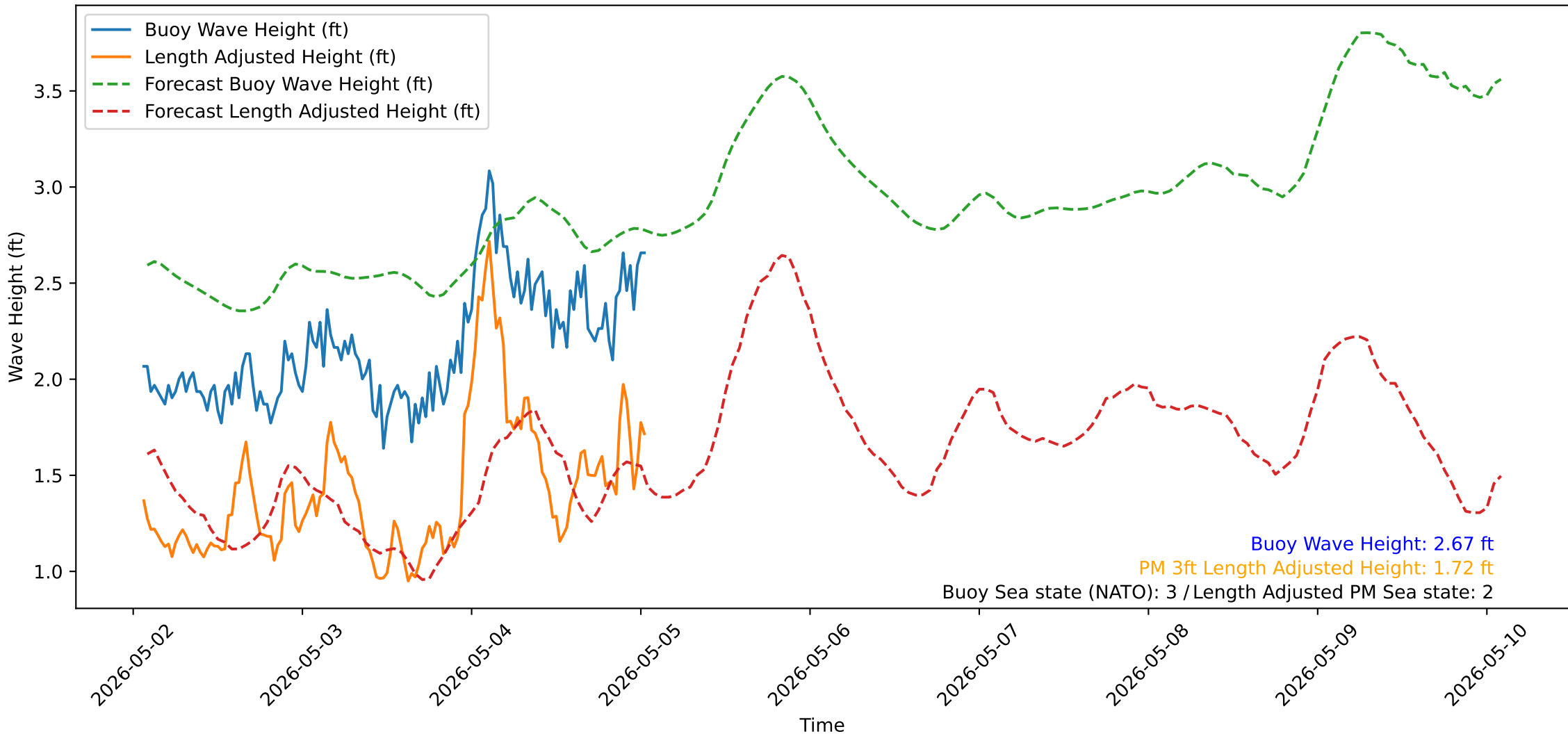
Wave Heights over Time for Oceanside Harbor at 2026-05-05 01:30:32
