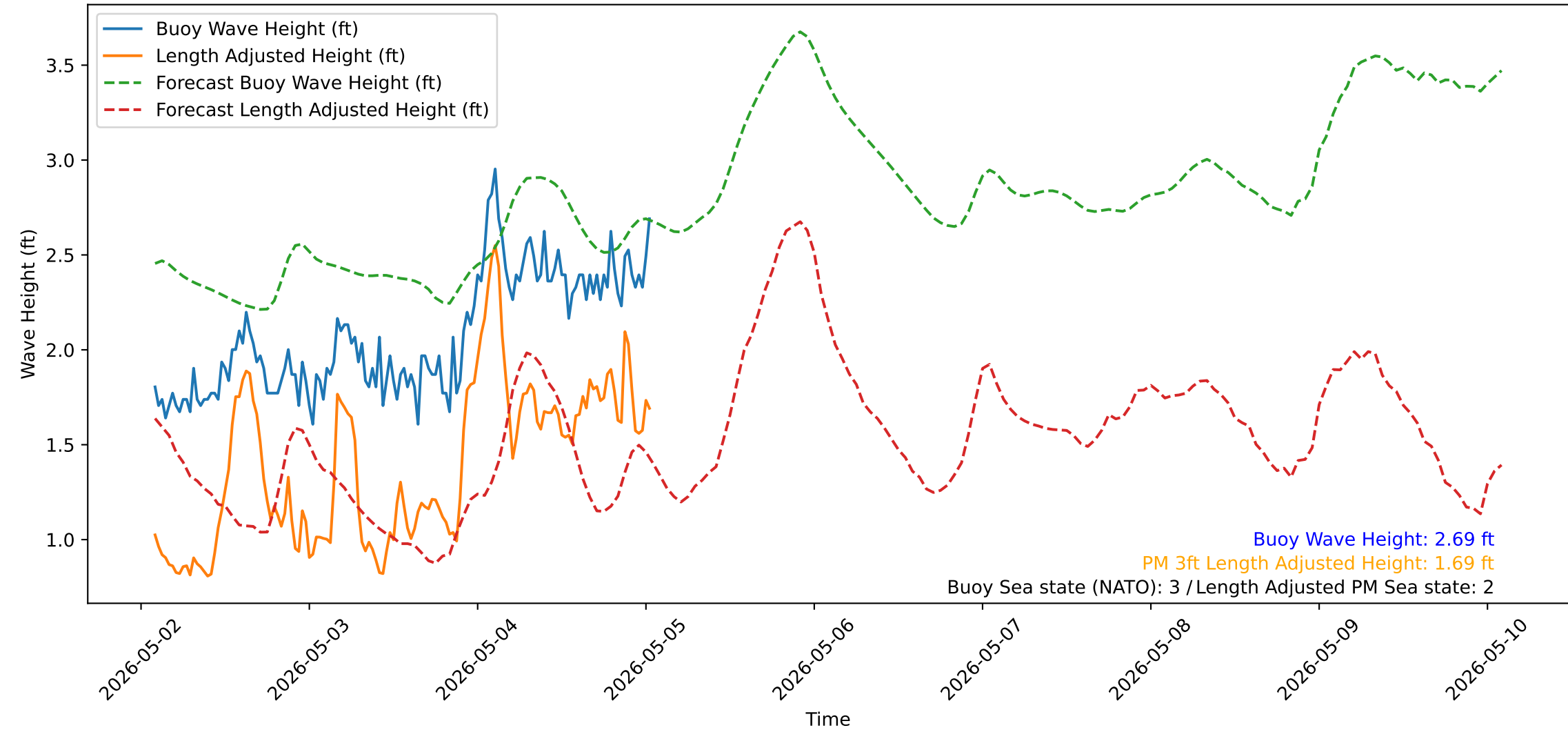
Wave Heights over Time for Red Beach at 2026-05-05 01:30:51
