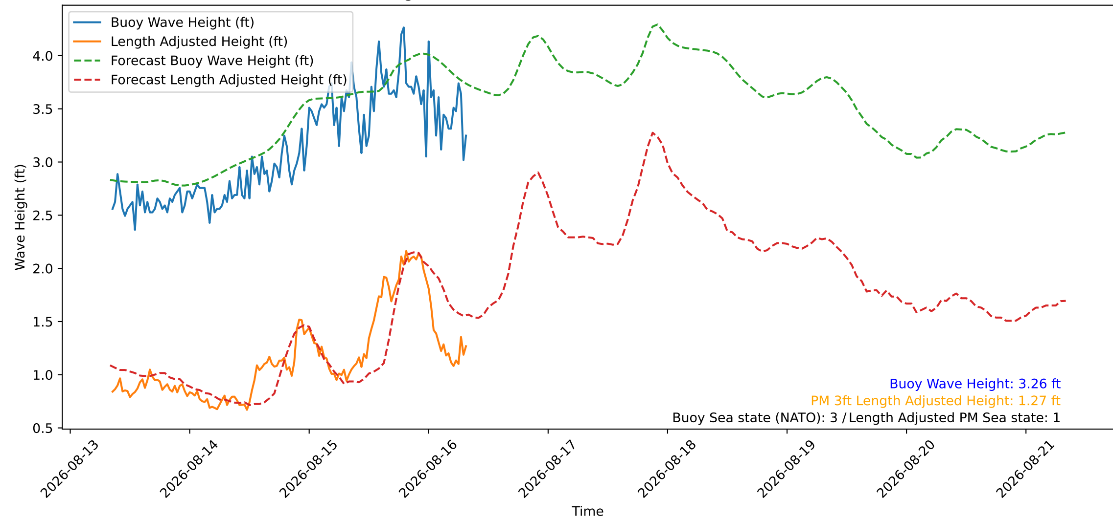
Wave Heights over Time for Green Beach at 2026-08-16 08:11:08
