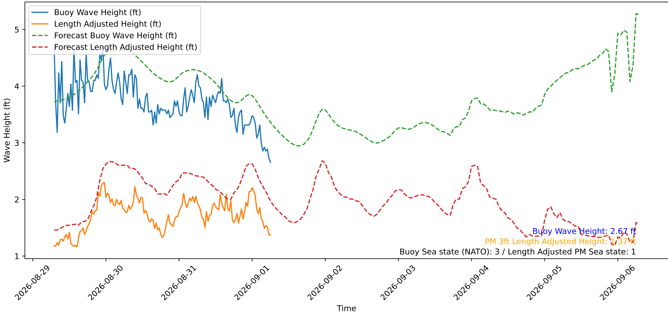
Wave Heights over Time for Red Beach at 2026-09-01 06:50:50
