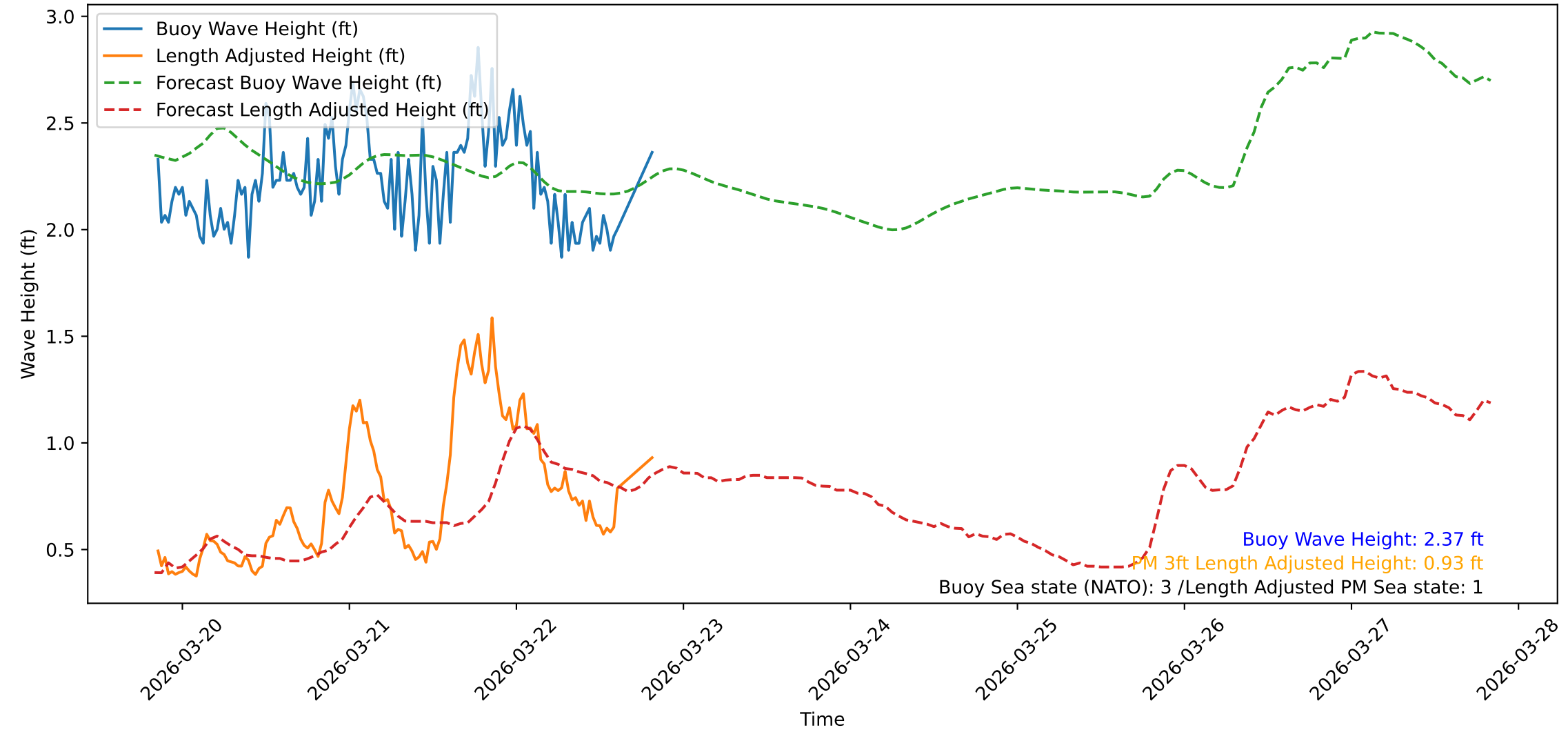
Wave Heights over Time for Red Beach at 2026-03-22 20:10:46
