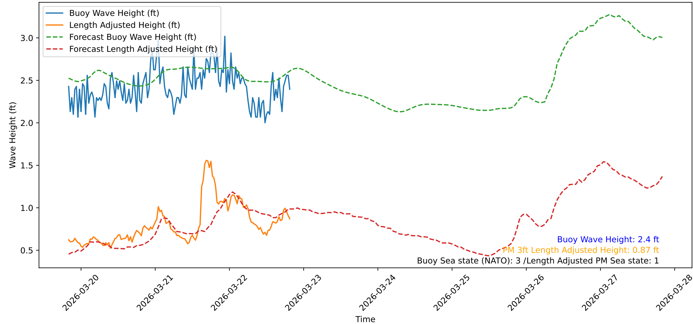
Wave Heights over Time for Oceanside Harbor at 2026-03-22 20:10:31
