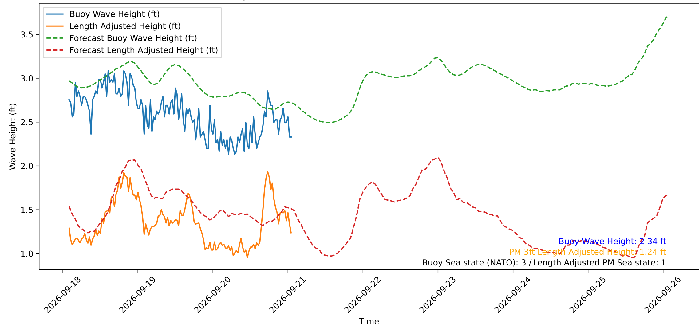
Wave Heights over Time for Oceanside Harbor at 2026-09-21 02:00:29
