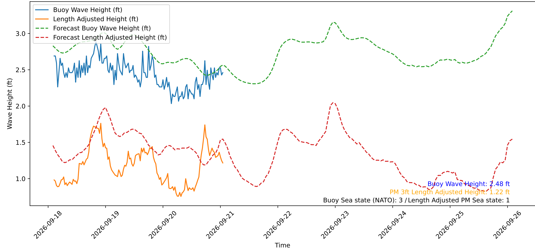
Wave Heights over Time for Red Beach at 2026-09-21 02:00:48
