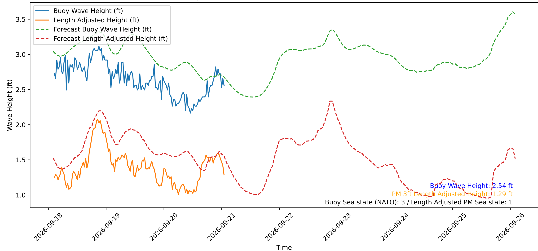
Wave Heights over Time for Green Beach at 2026-09-21 02:01:10
