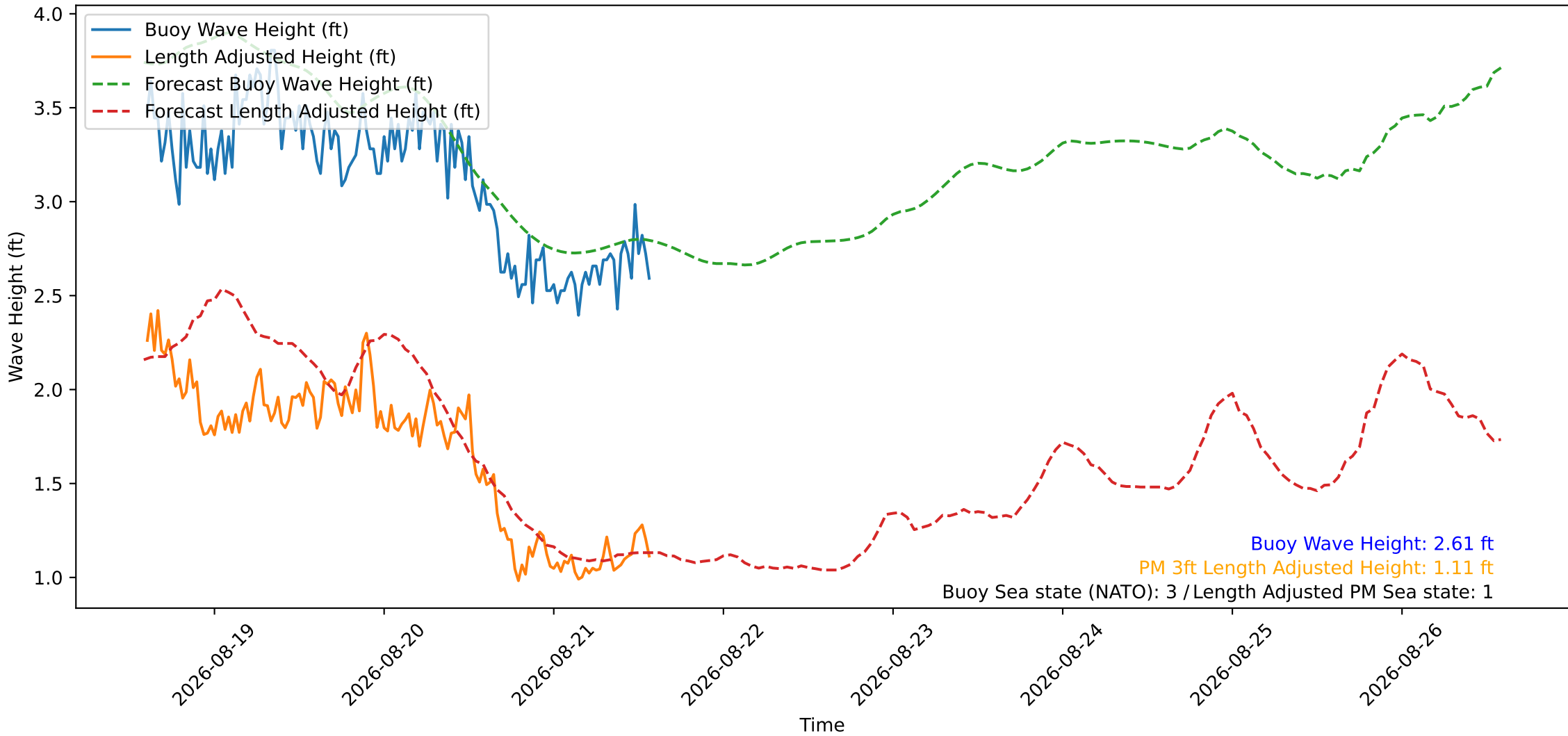
Wave Heights over Time for Oceanside Harbor at 2026-08-21 14:20:27
