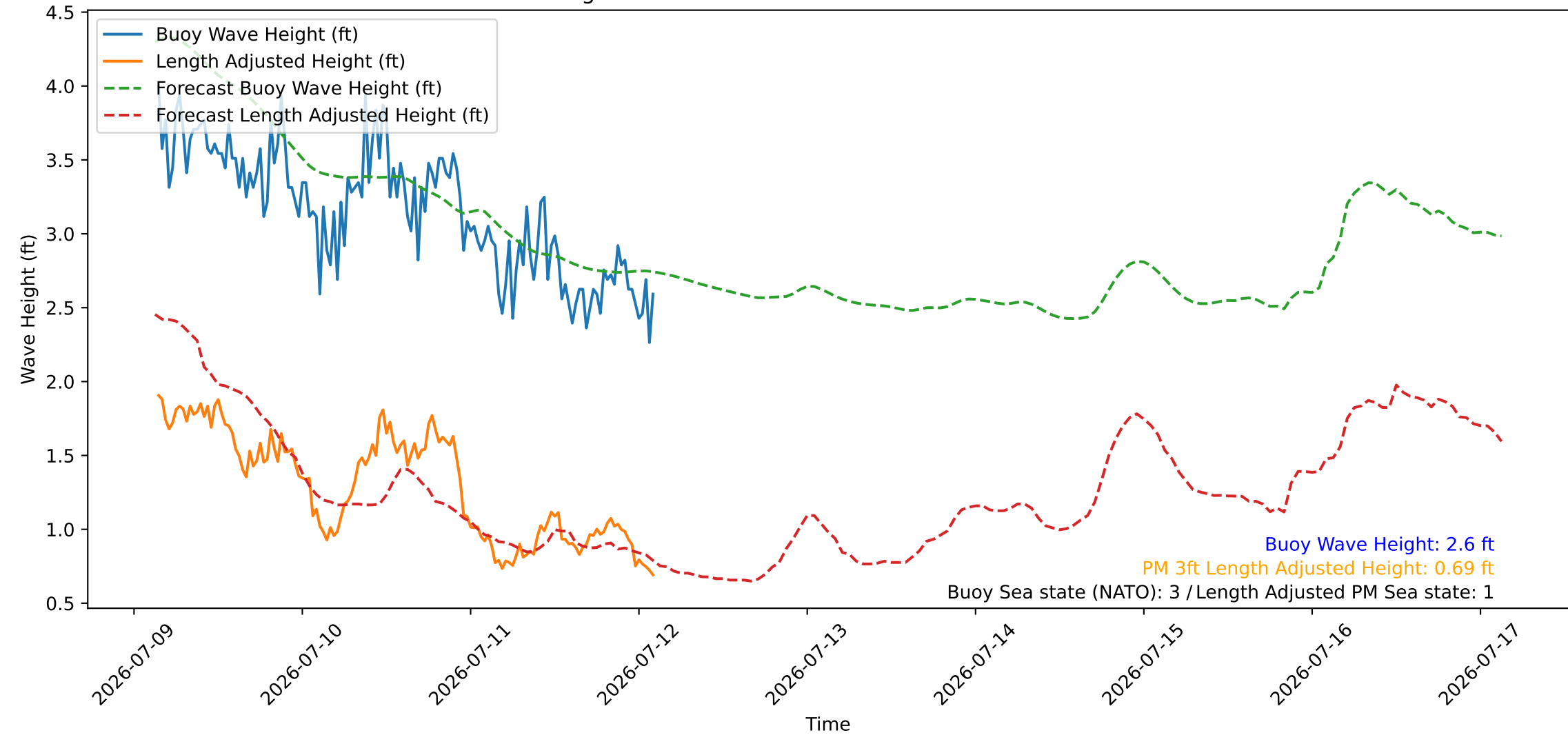
Wave Heights over Time for Red Beach at 2026-07-12 03:00:45
