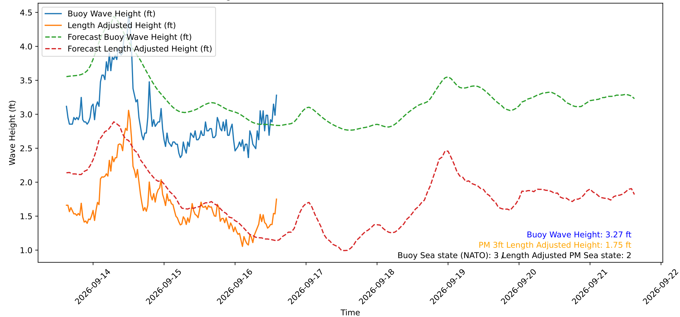
Wave Heights over Time for Oceanside Harbor at 2026-09-16 14:50:29
