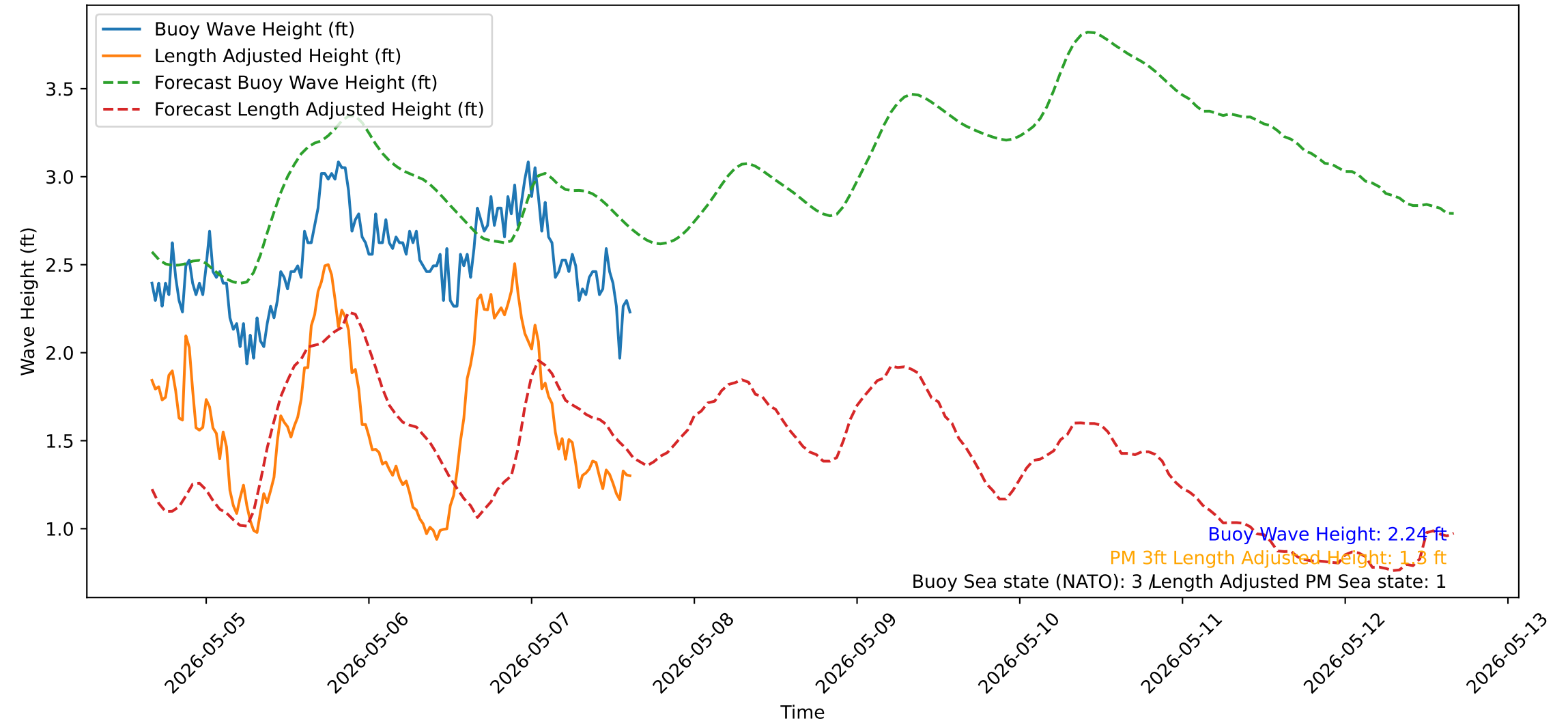
Wave Heights over Time for Red Beach at 2026-05-07 15:30:50
