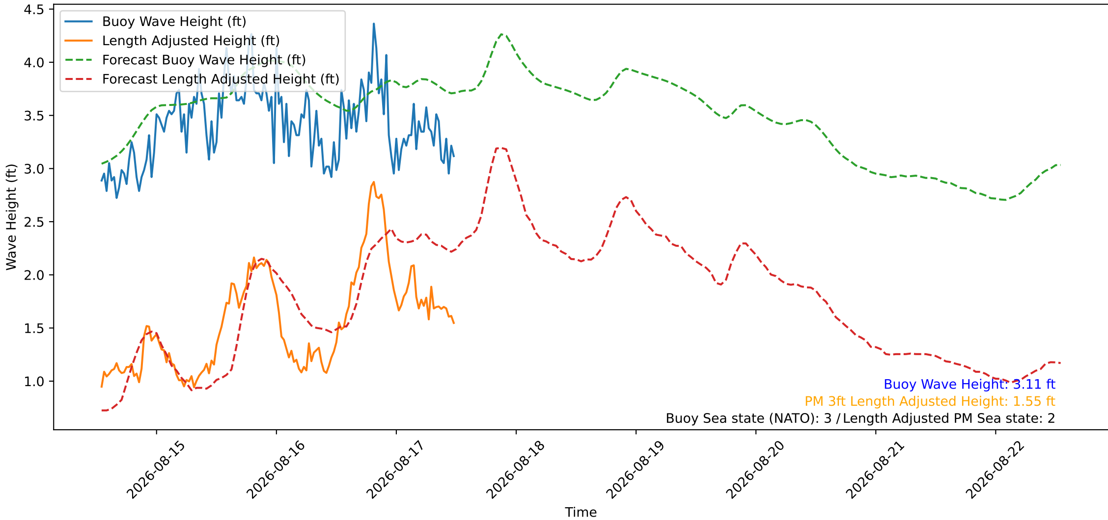
Wave Heights over Time for Green Beach at 2026-08-17 12:31:08
