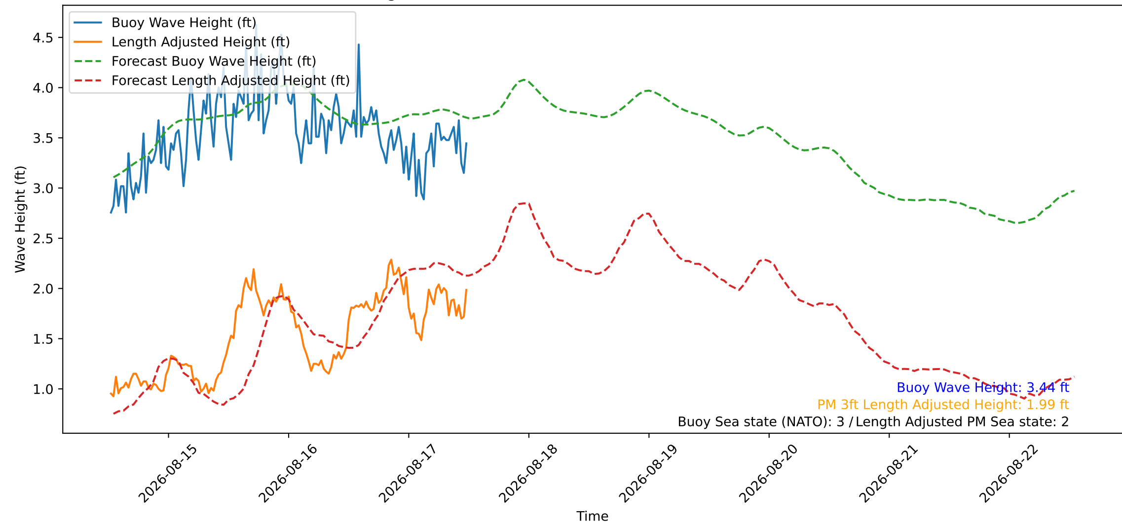
Wave Heights over Time for Oceanside Harbor at 2026-08-17 12:30:26
