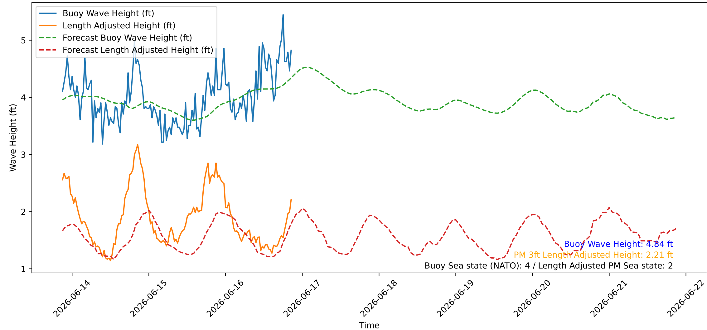
Wave Heights over Time for Oceanside Harbor at 2026-06-16 21:10:25
