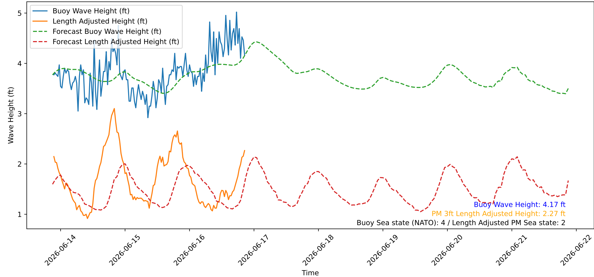
Wave Heights over Time for Red Beach at 2026-06-16 21:10:45
