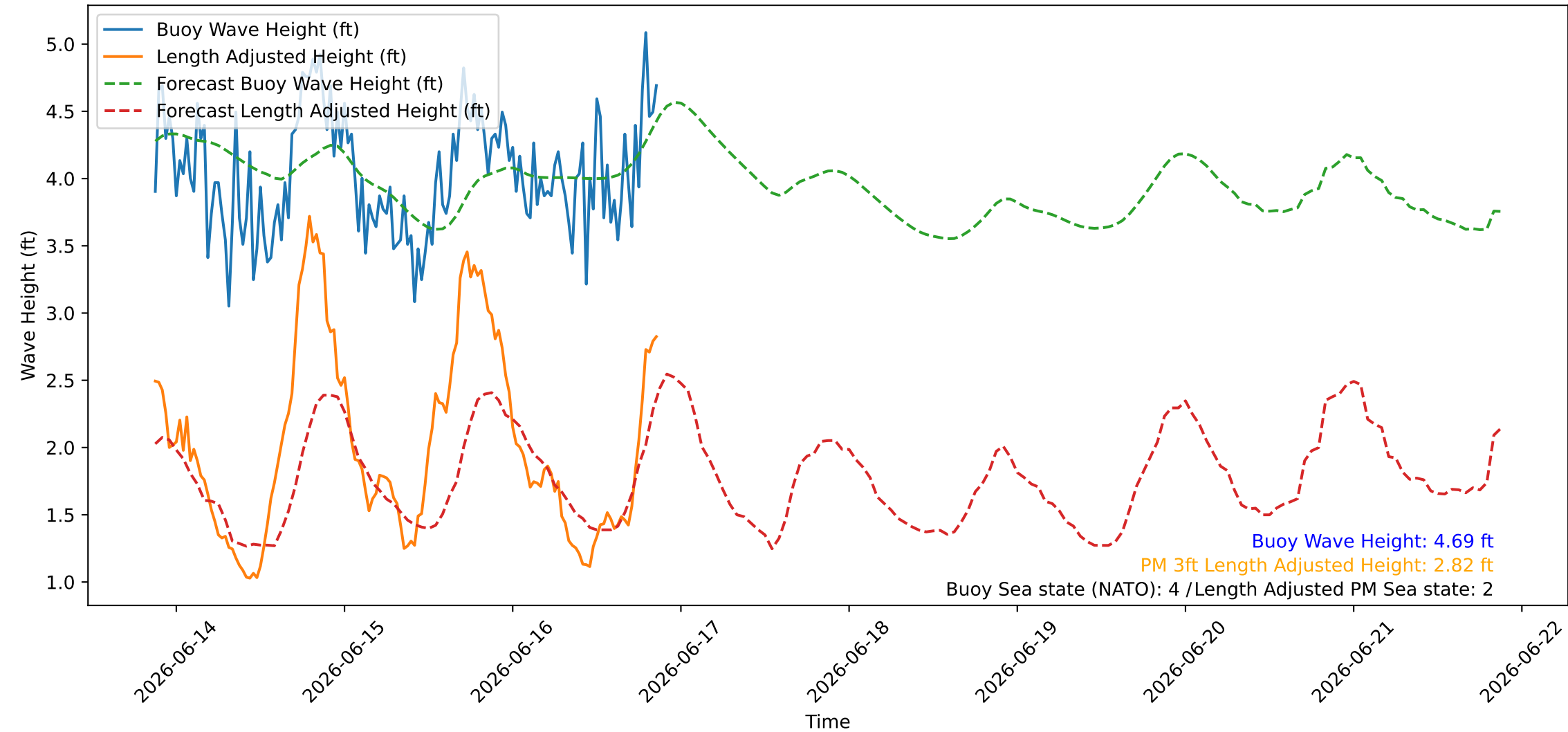
Wave Heights over Time for Green Beach at 2026-06-16 21:11:08
