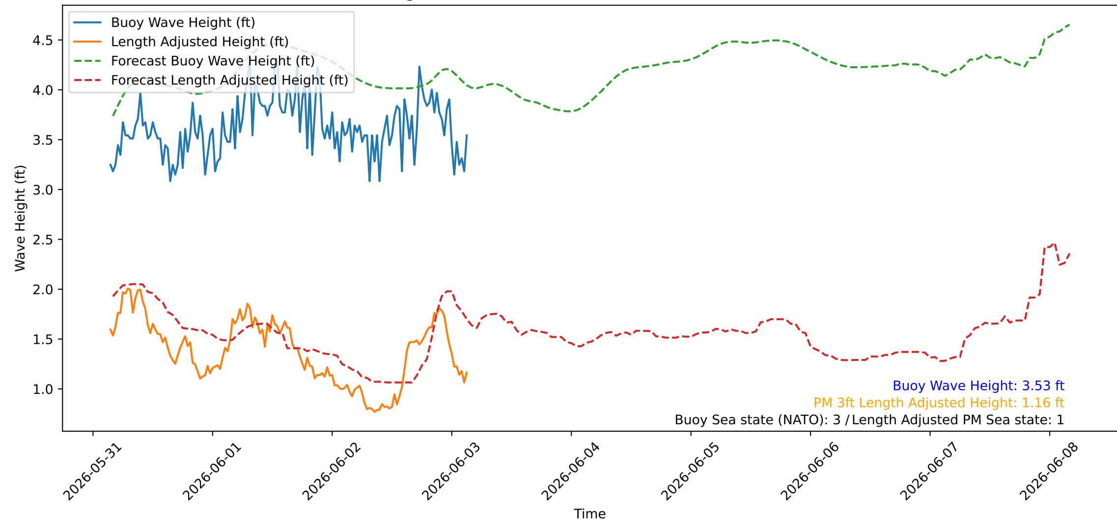
Wave Heights over Time for Green Beach at 2026-06-03 03:41:07
