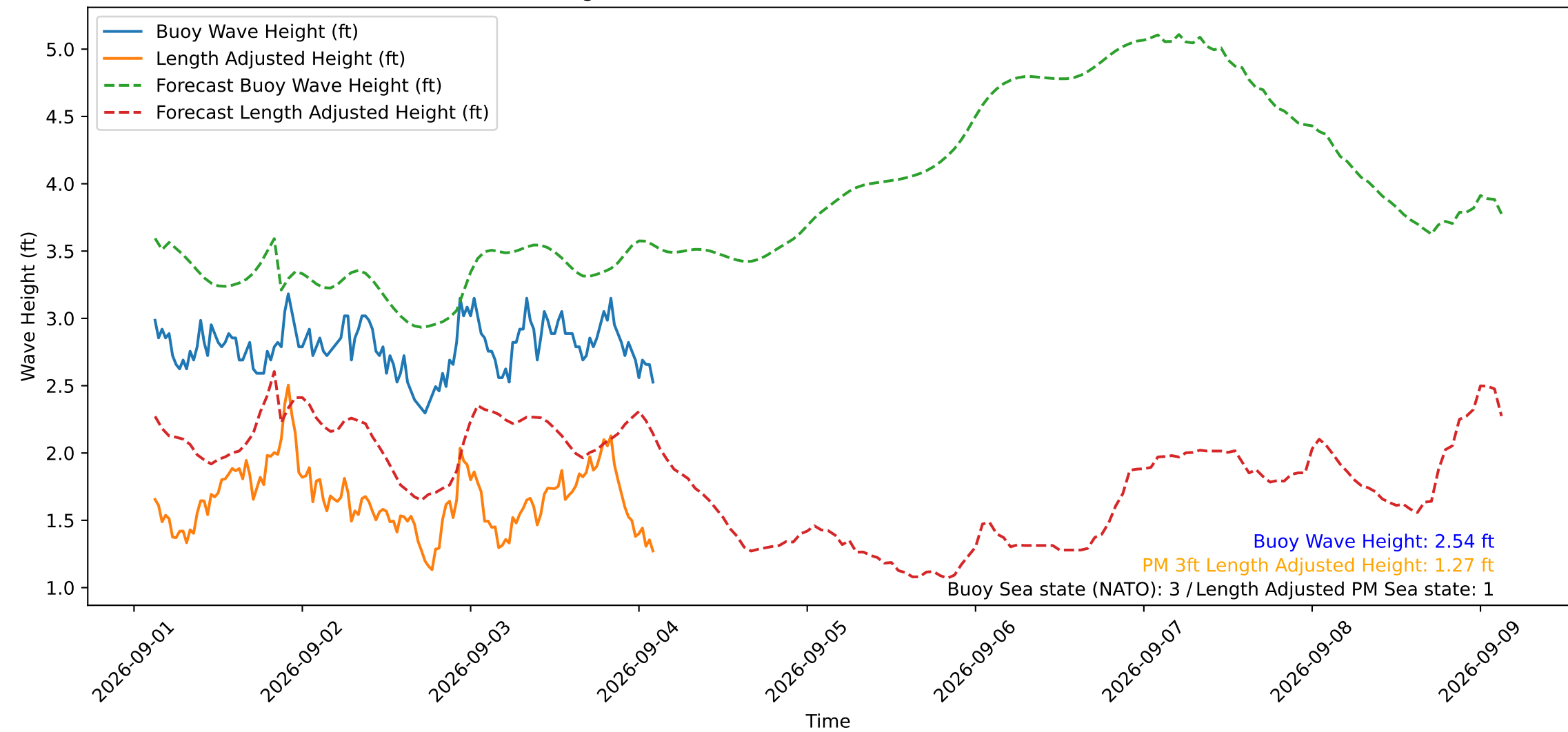
Wave Heights over Time for Red Beach at 2026-09-04 02:50:51
