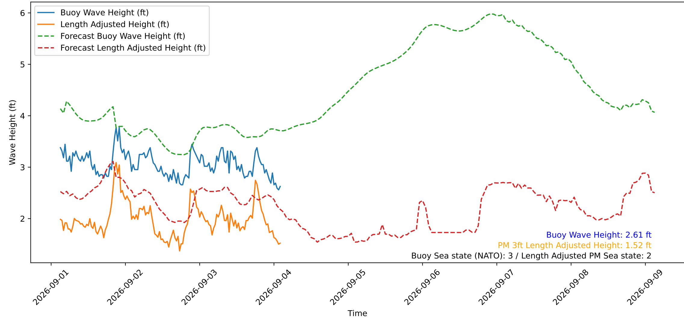
Wave Heights over Time for Green Beach at 2026-09-04 02:51:15
