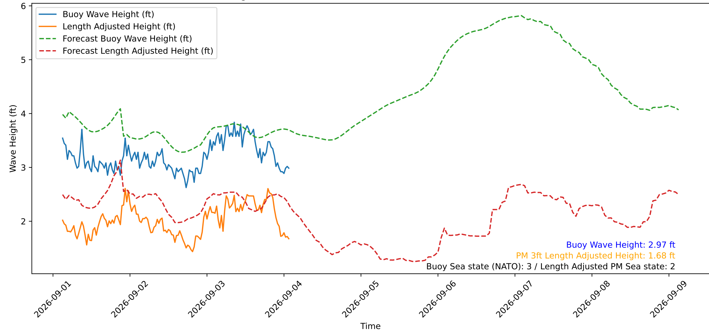
Wave Heights over Time for Oceanside Harbor at 2026-09-04 02:50:30
