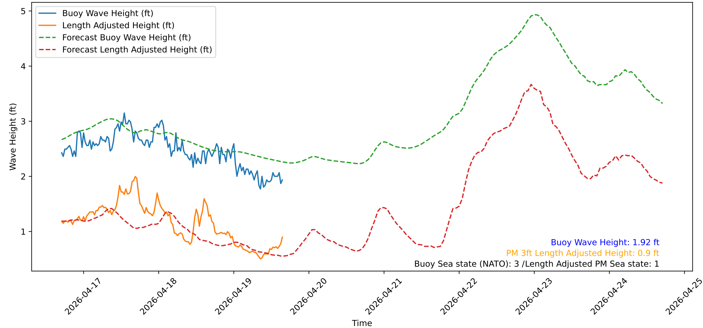
Wave Heights over Time for Red Beach at 2026-04-19 16:40:50
