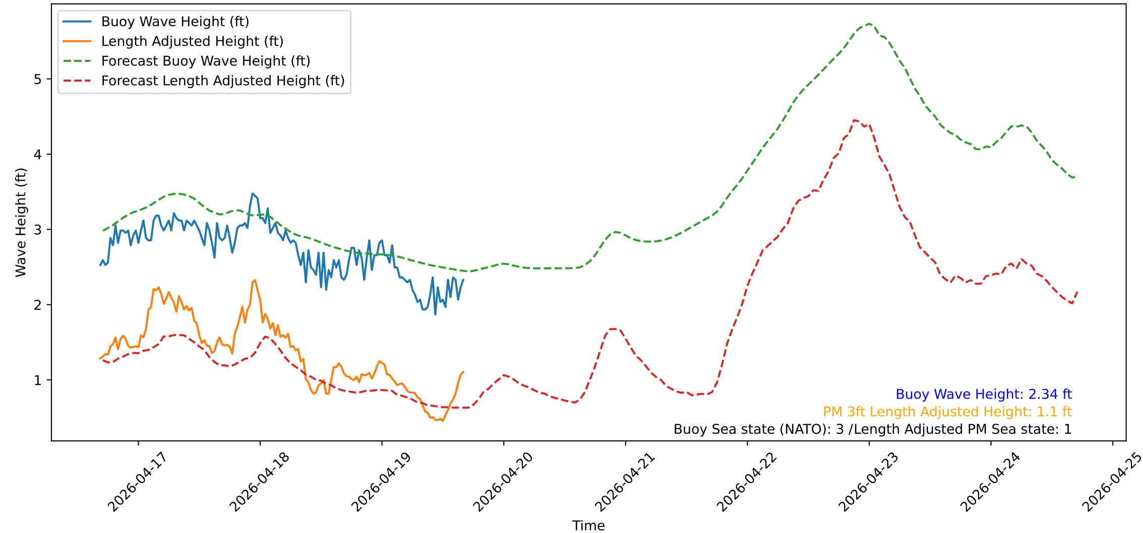
Wave Heights over Time for Green Beach at 2026-04-19 16:41:13
