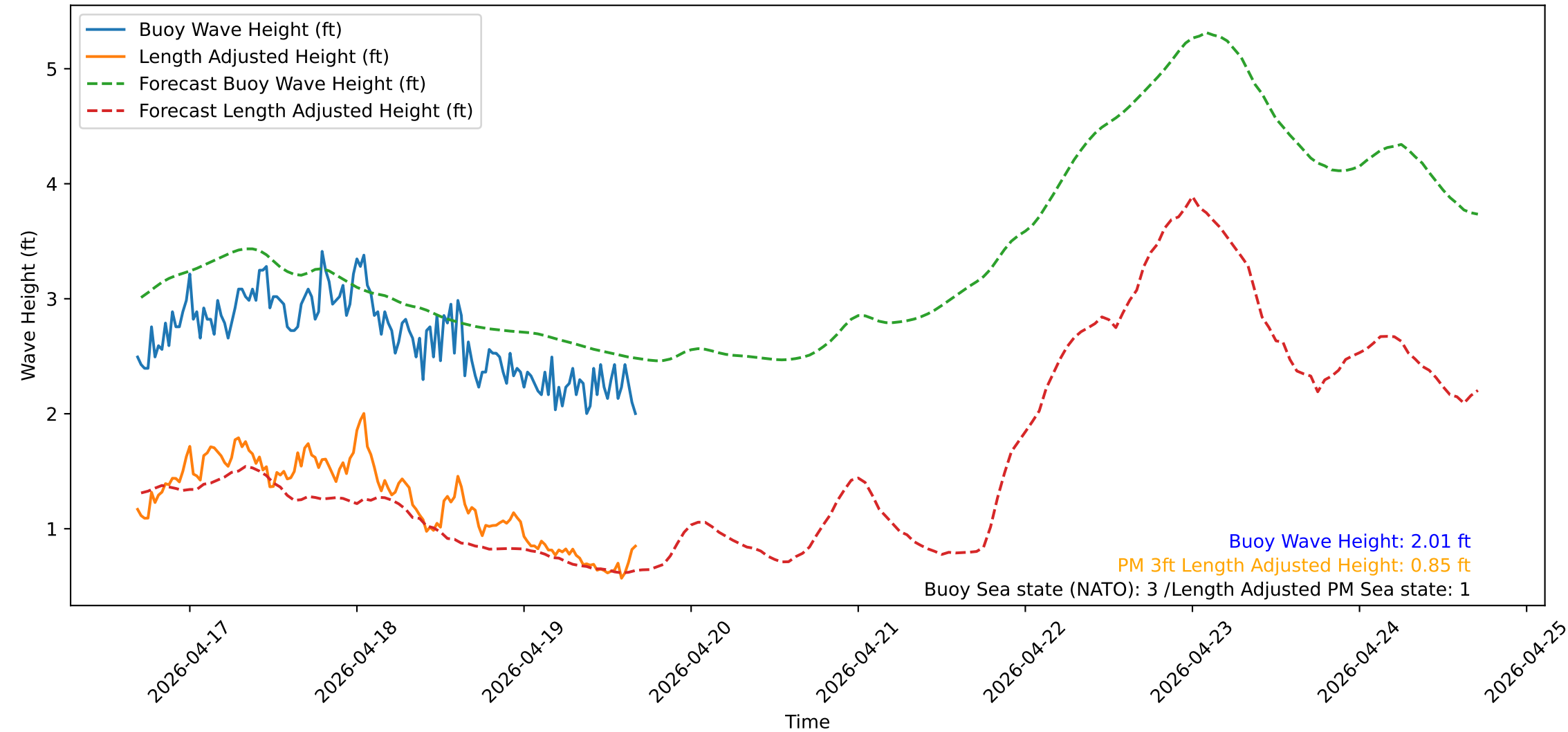
Wave Heights over Time for Oceanside Harbor at 2026-04-19 16:40:31
