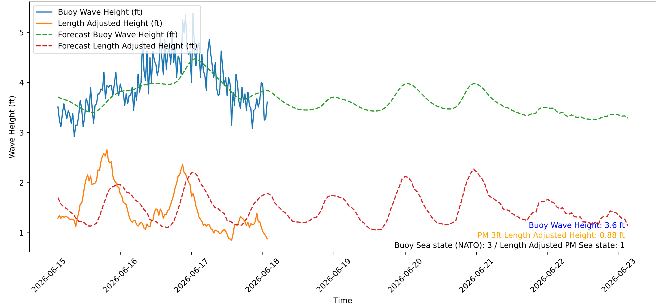
Wave Heights over Time for Red Beach at 2026-06-18 02:30:45
