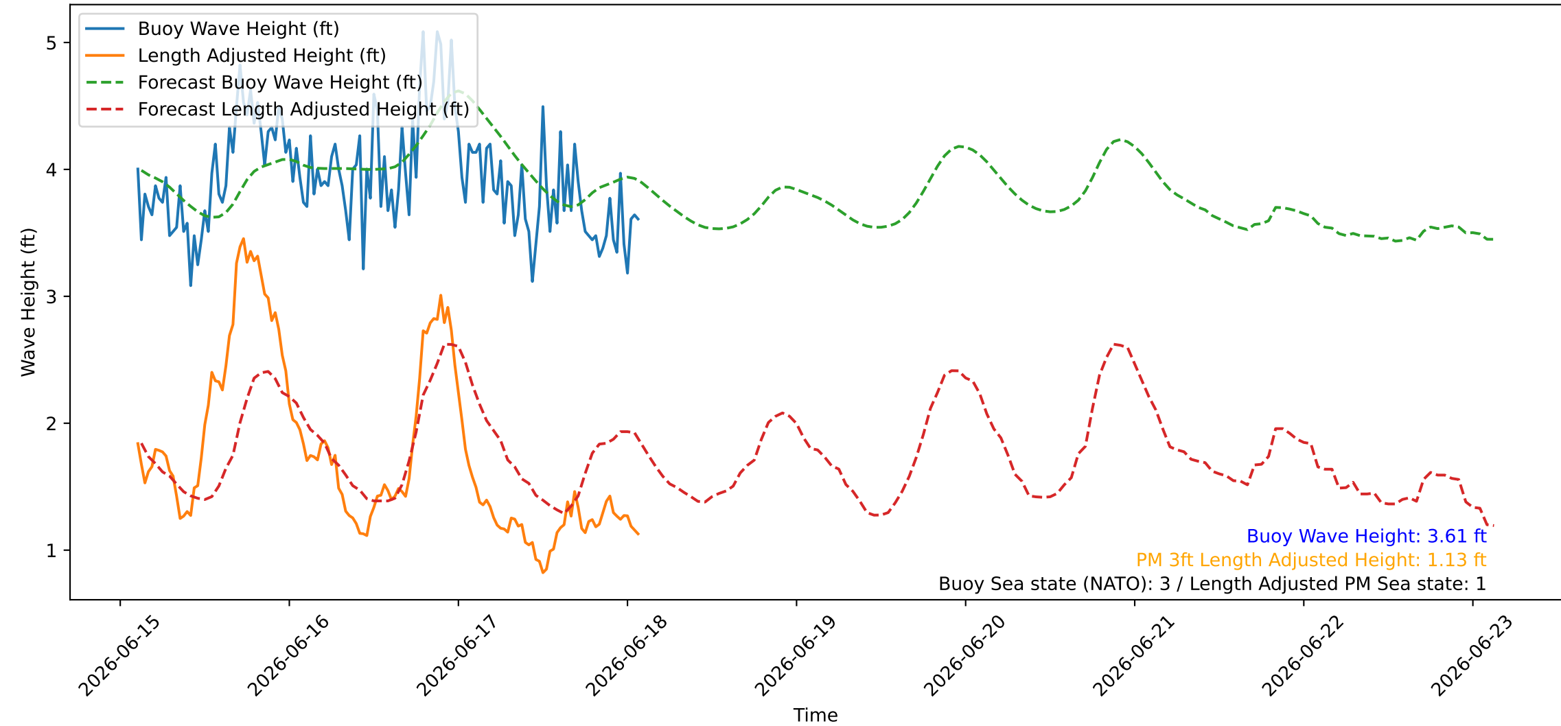
Wave Heights over Time for Green Beach at 2026-06-18 02:31:08
