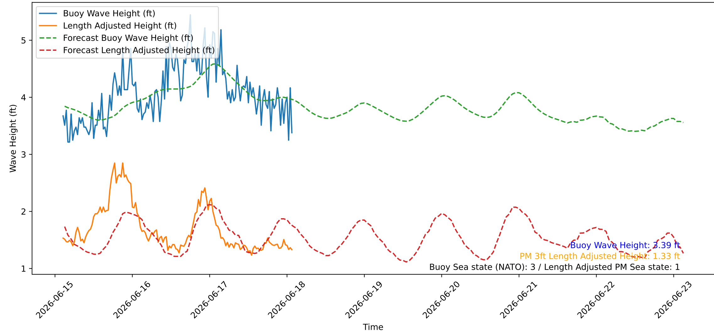
Wave Heights over Time for Oceanside Harbor at 2026-06-18 02:30:26
