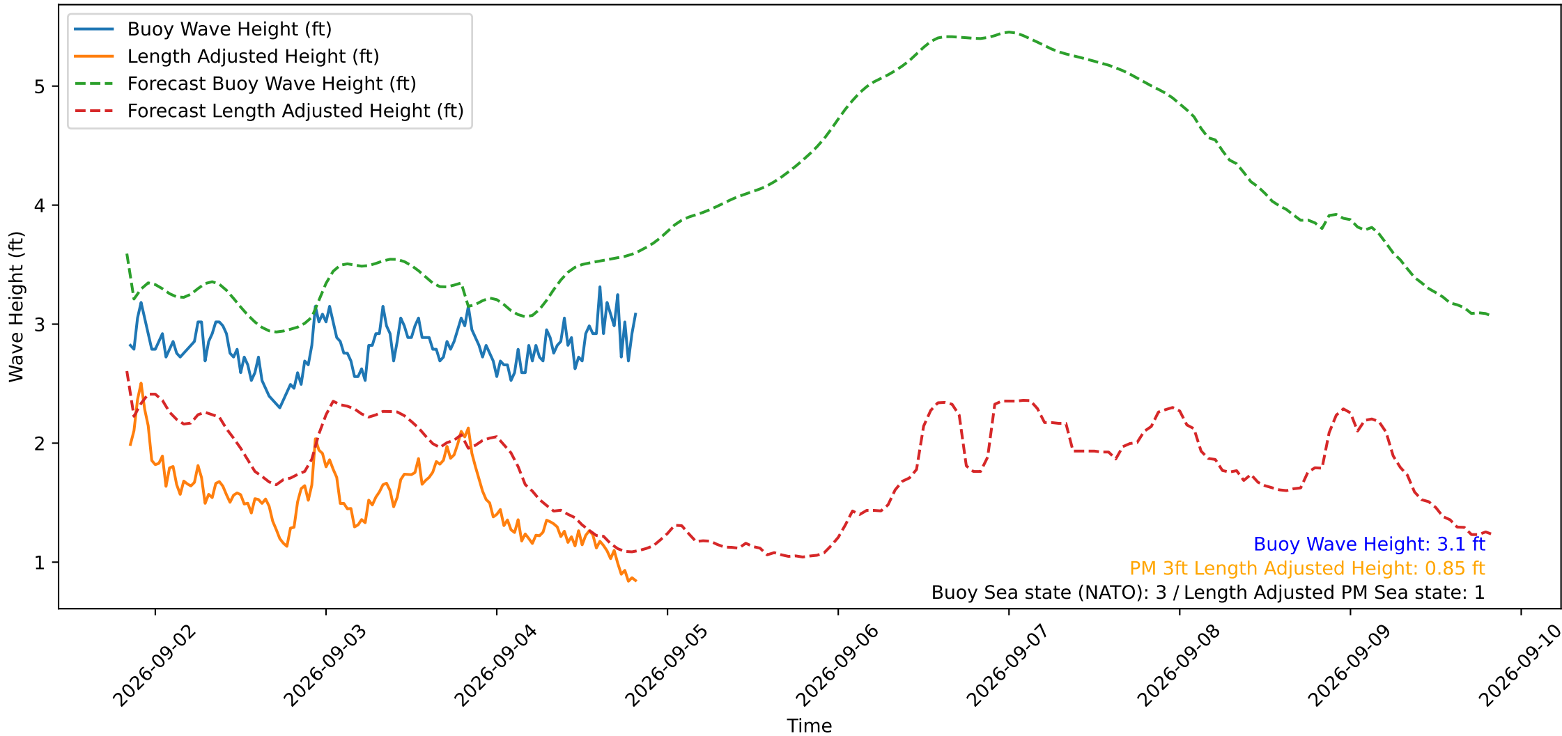
Wave Heights over Time for Red Beach at 2026-09-04 20:10:49
