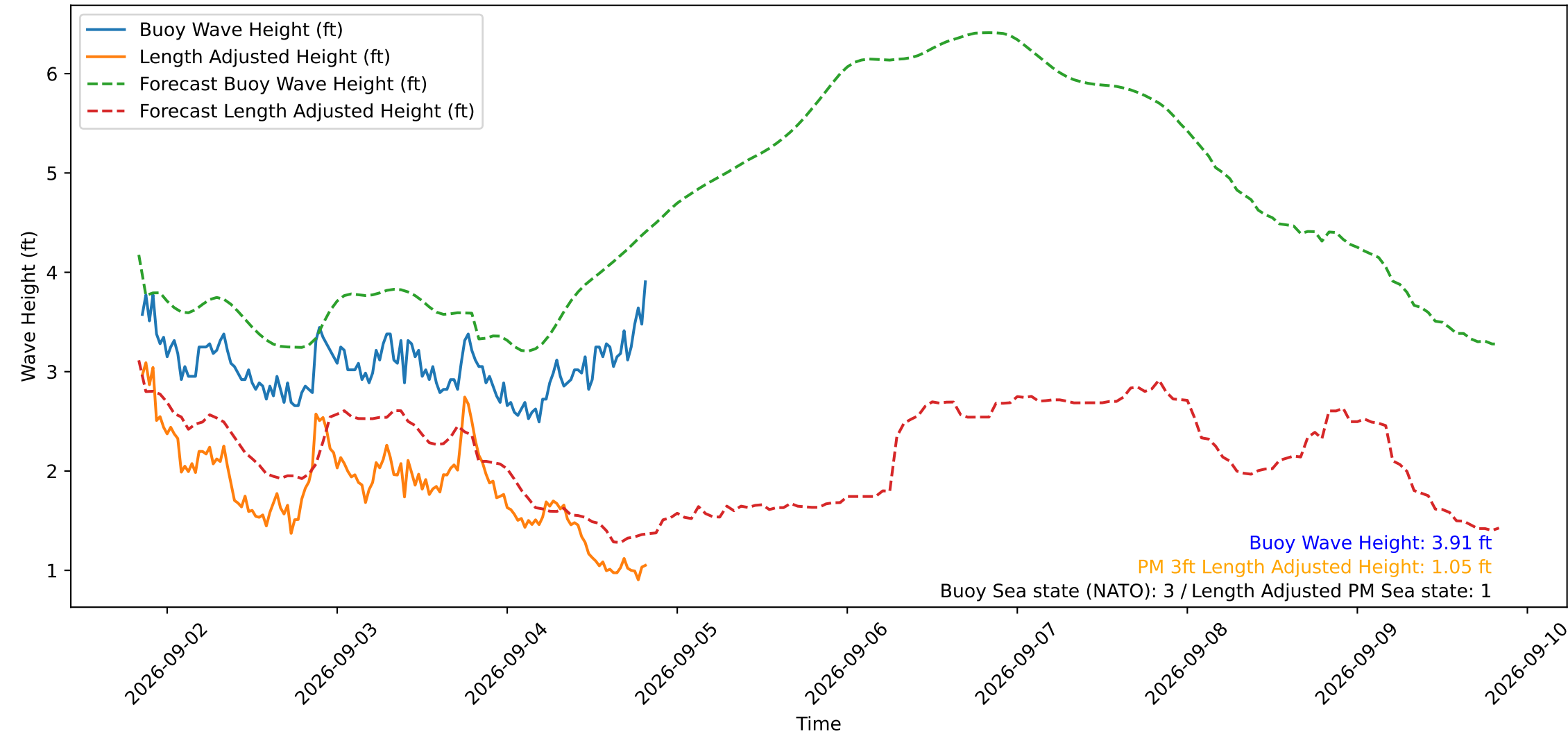
Wave Heights over Time for Green Beach at 2026-09-04 20:11:13
