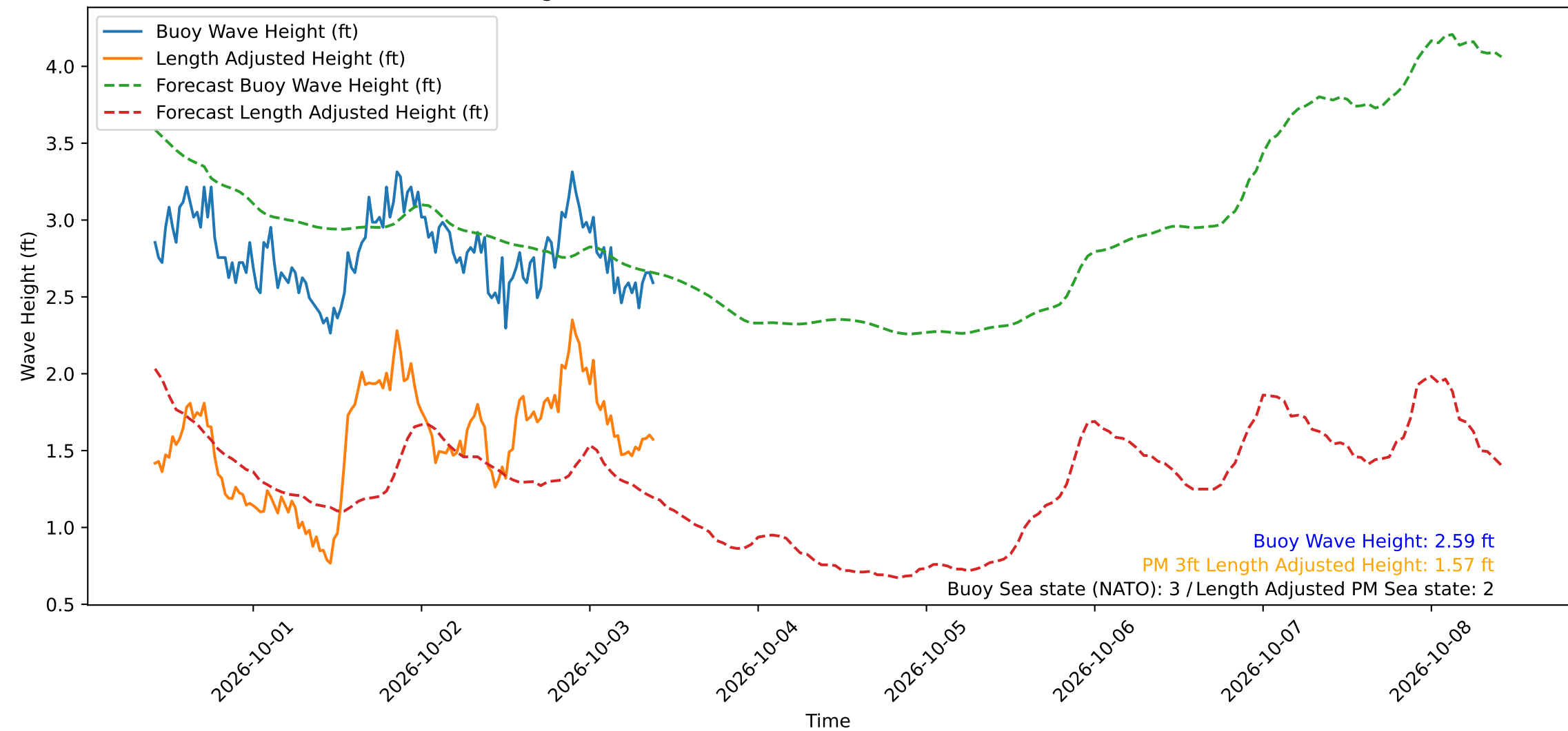
Wave Heights over Time for Oceanside Harbor at 2026-10-03 10:00:29
