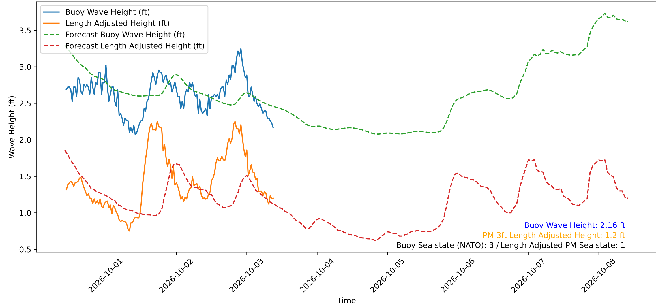
Wave Heights over Time for Red Beach at 2026-10-03 10:00:49
