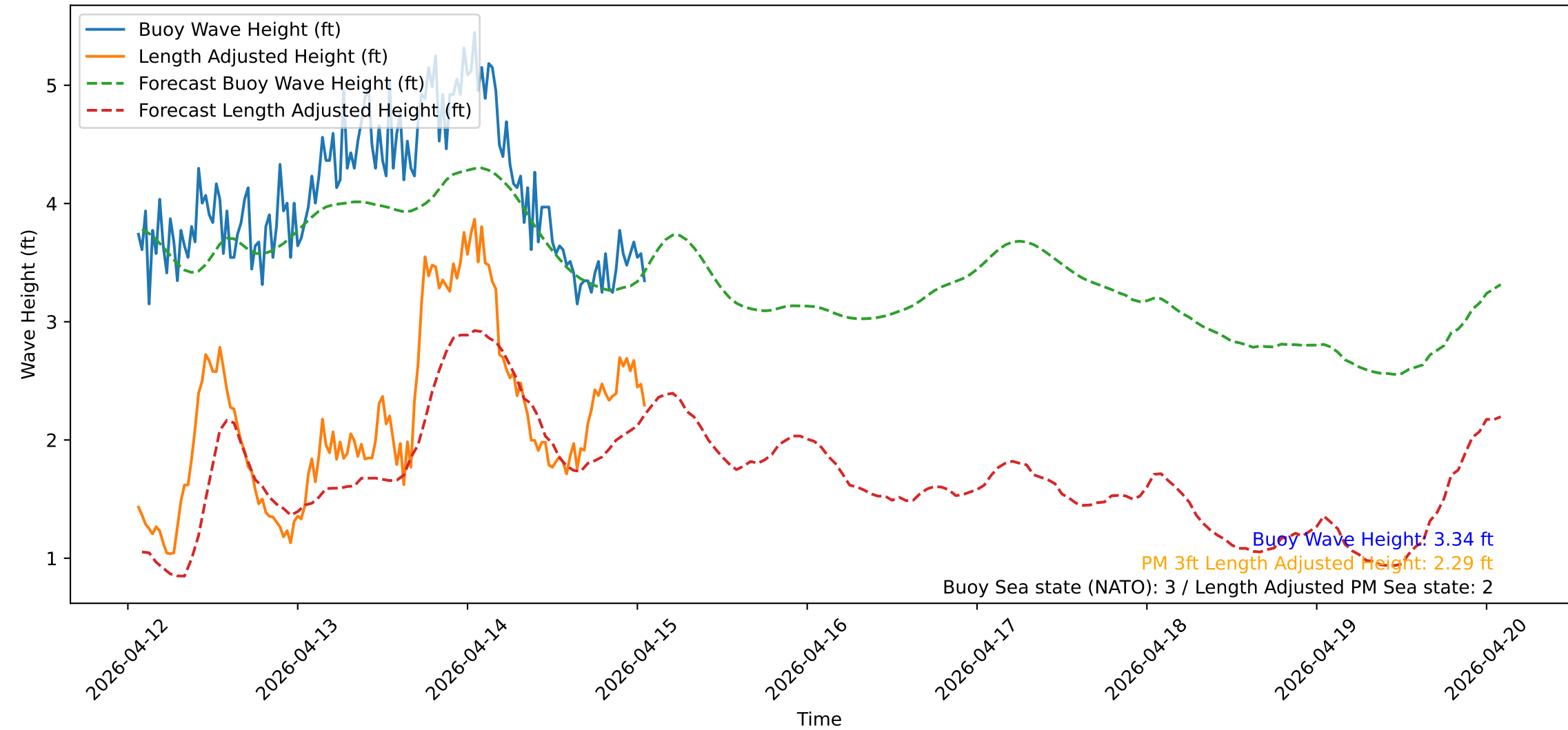
Wave Heights over Time for Oceanside Harbor at 2026-04-15 01:30:31
