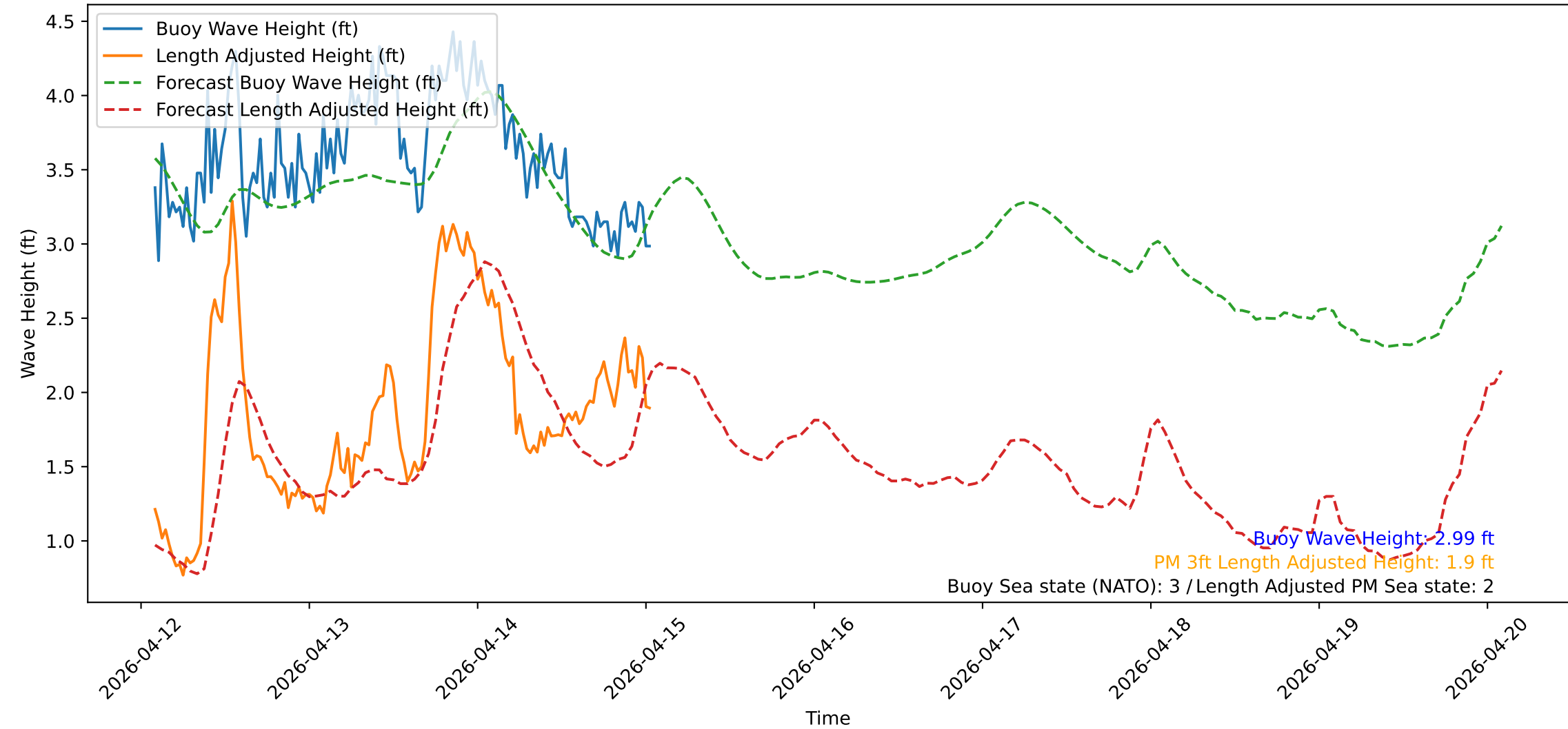
Wave Heights over Time for Red Beach at 2026-04-15 01:30:50
