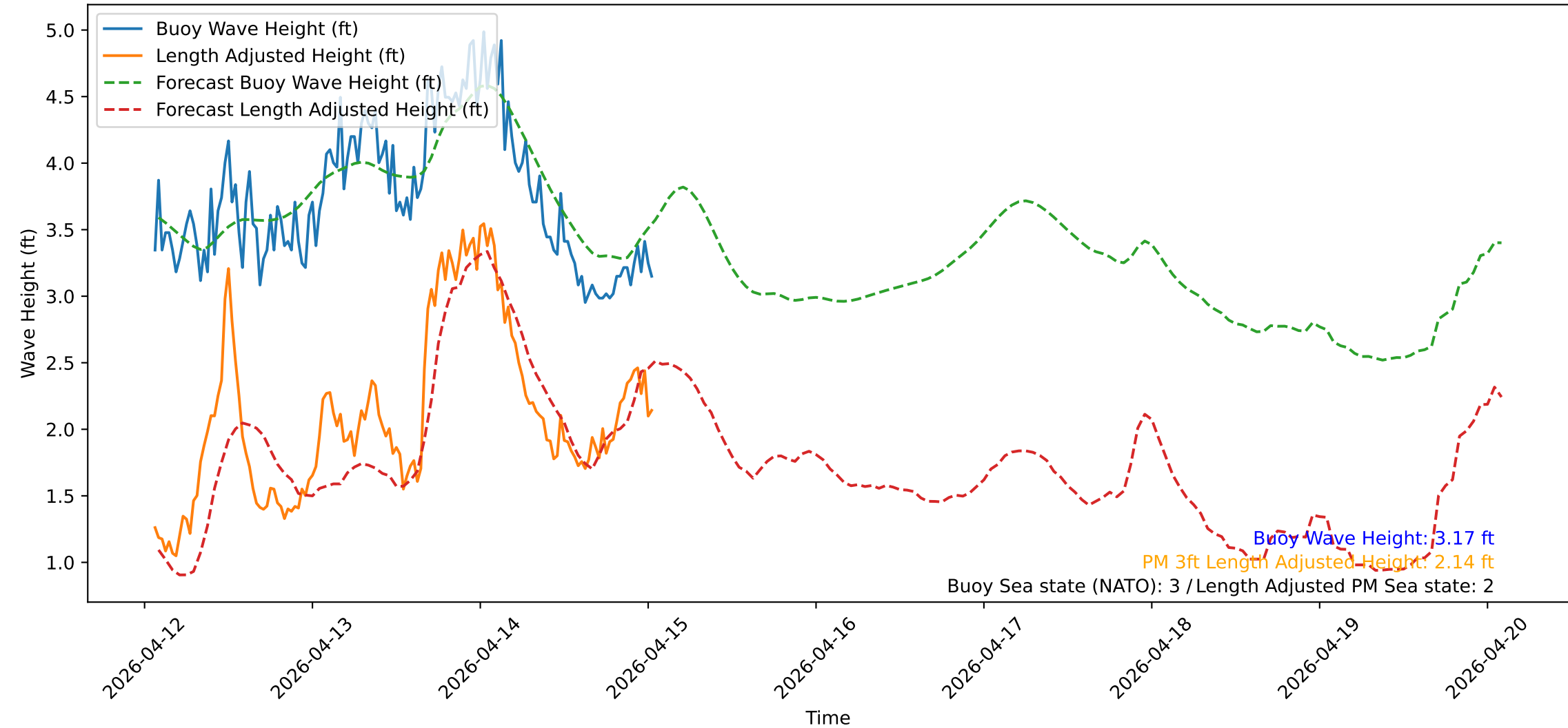
Wave Heights over Time for Green Beach at 2026-04-15 01:31:12
