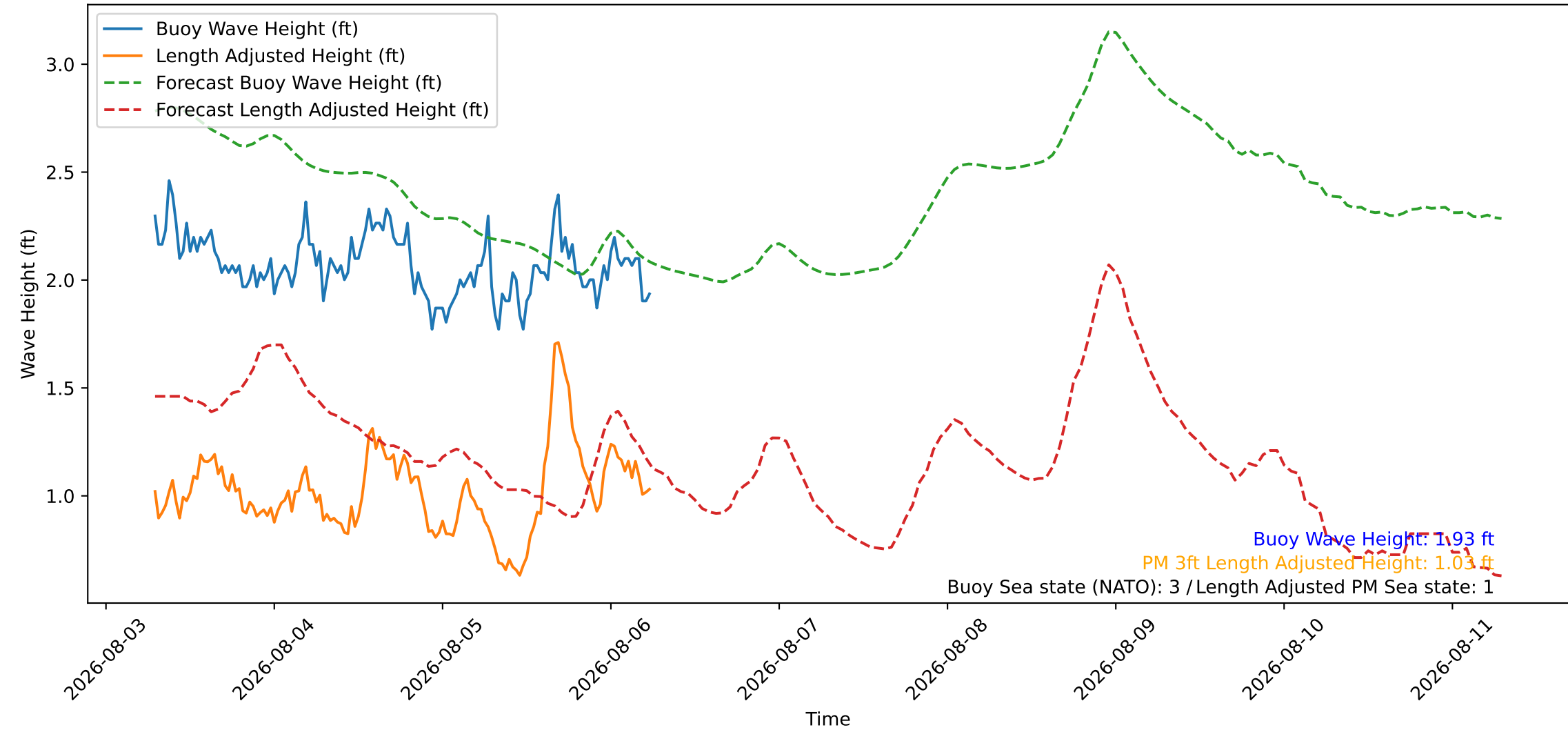
Wave Heights over Time for Red Beach at 2026-08-06 06:30:45
