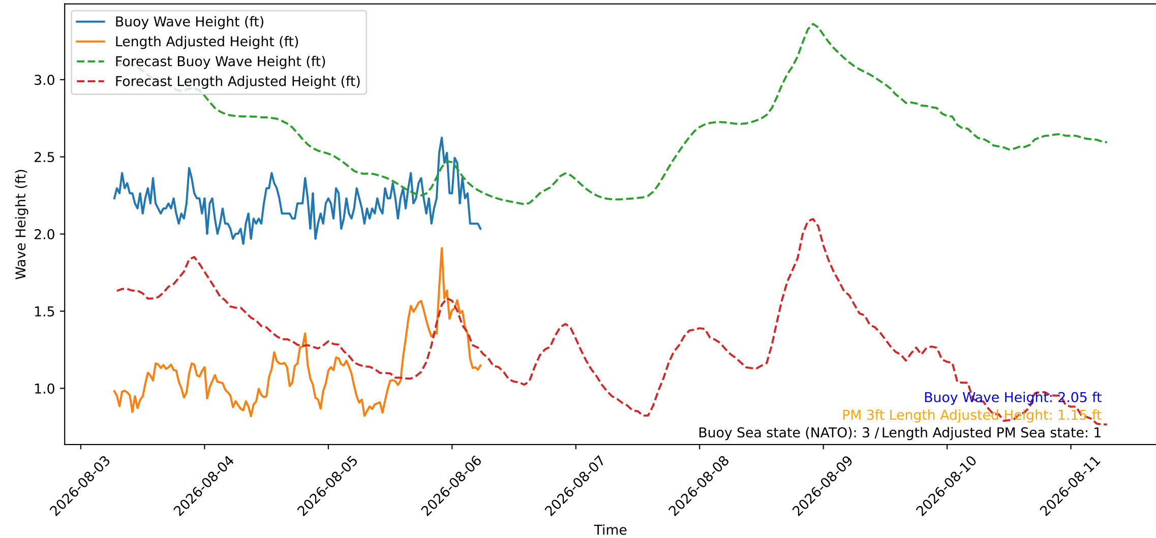
Wave Heights over Time for Green Beach at 2026-08-06 06:31:08
