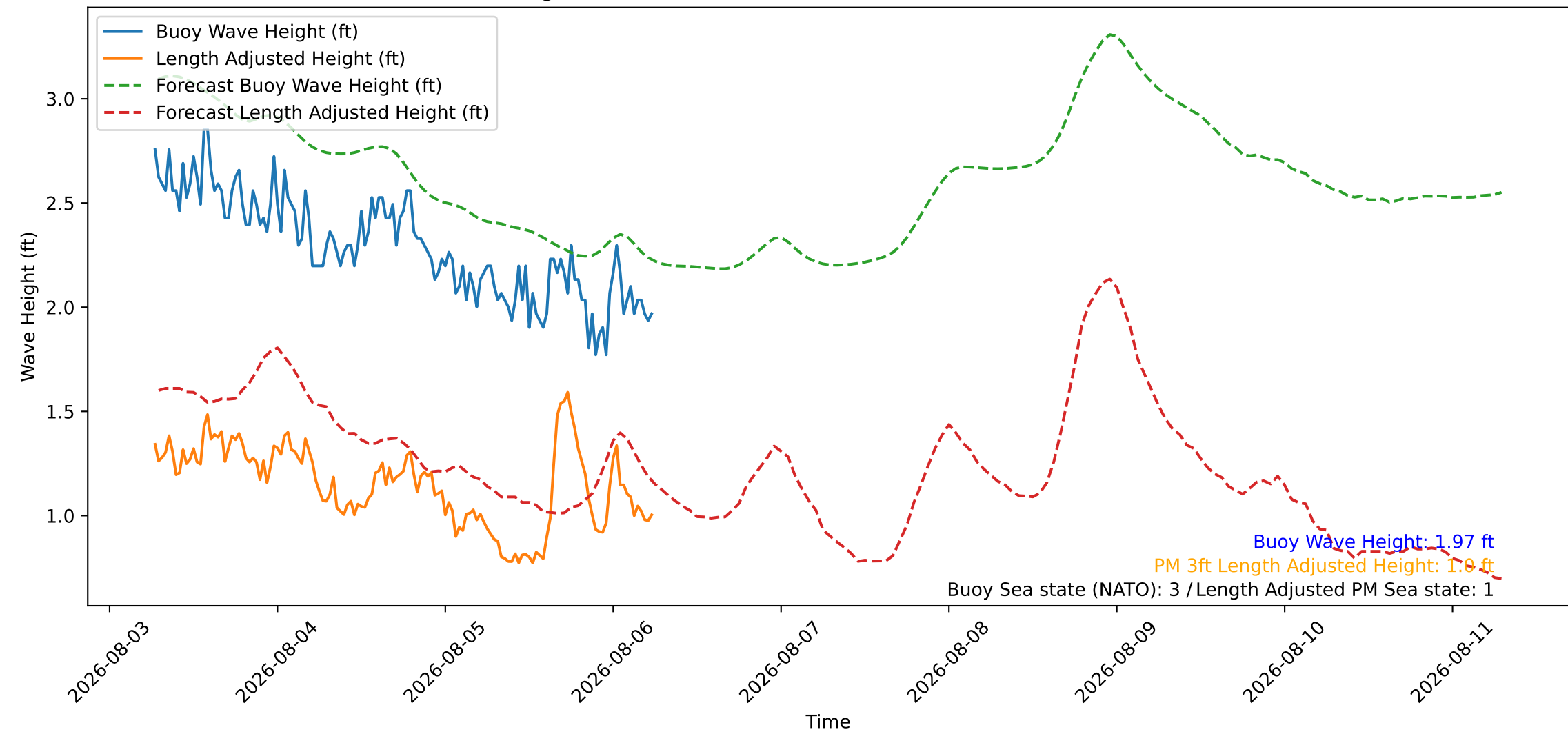
Wave Heights over Time for Oceanside Harbor at 2026-08-06 06:30:26
