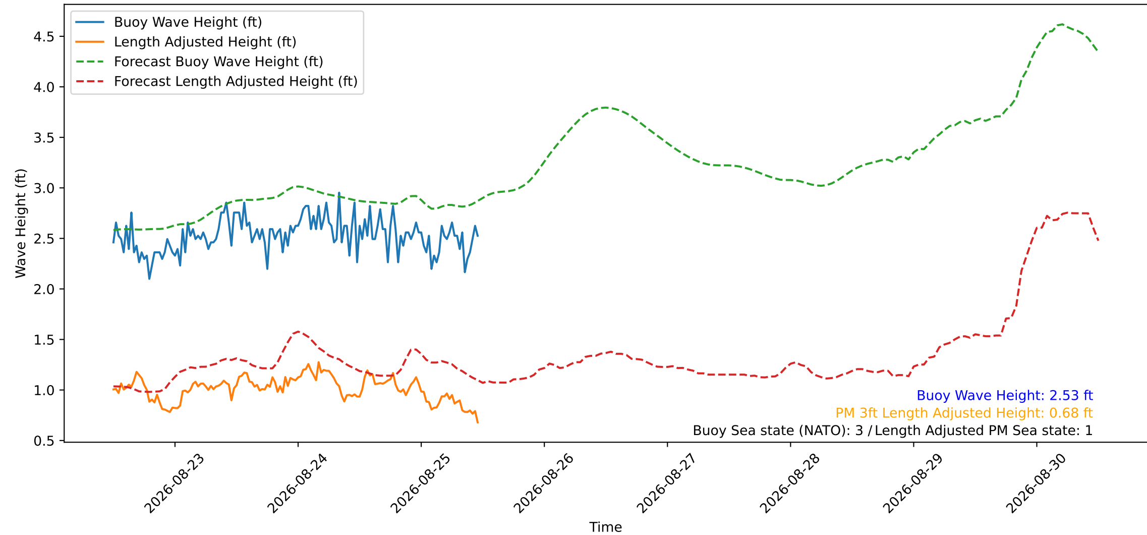
Wave Heights over Time for Red Beach at 2026-08-25 11:50:51
