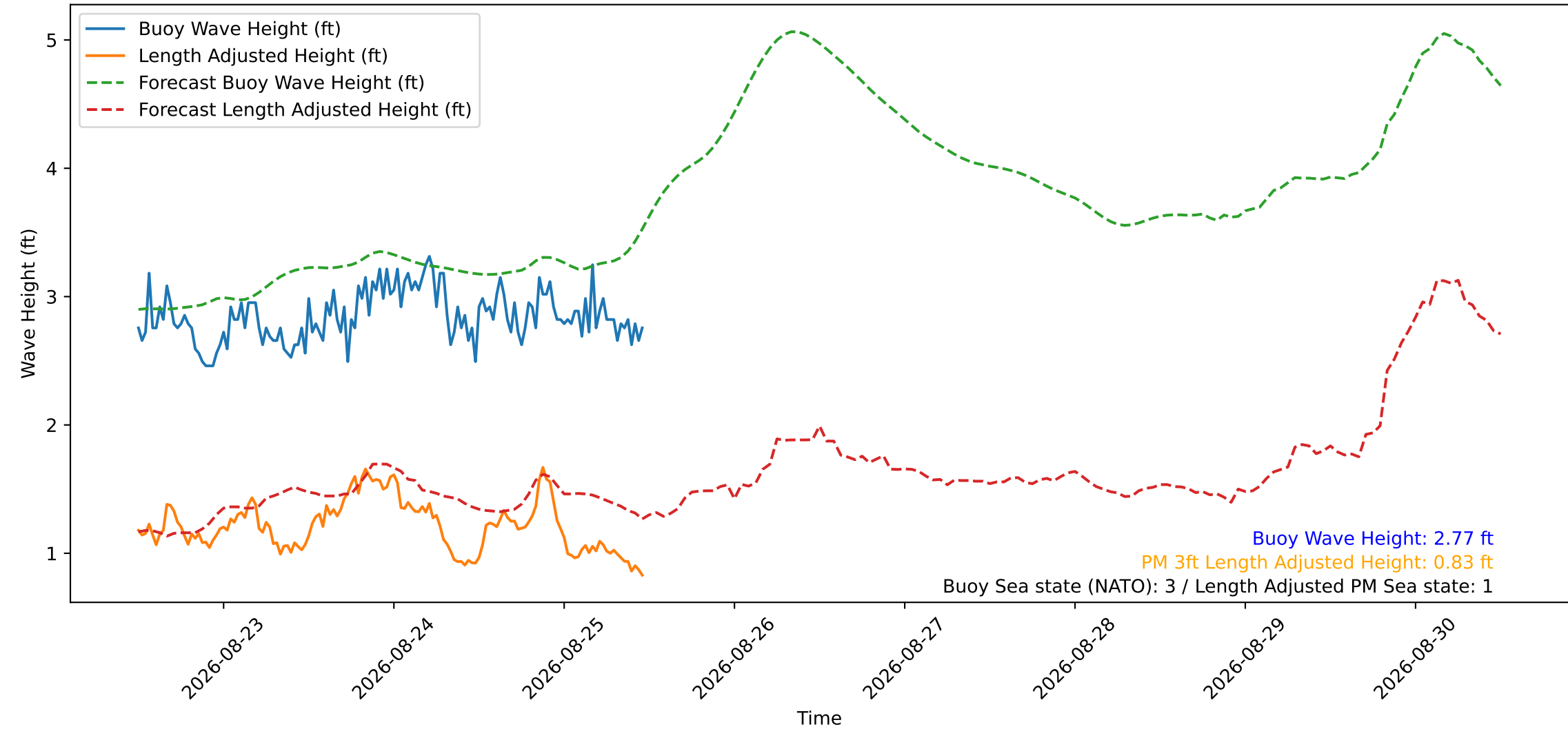
Wave Heights over Time for Green Beach at 2026-08-25 11:51:15
