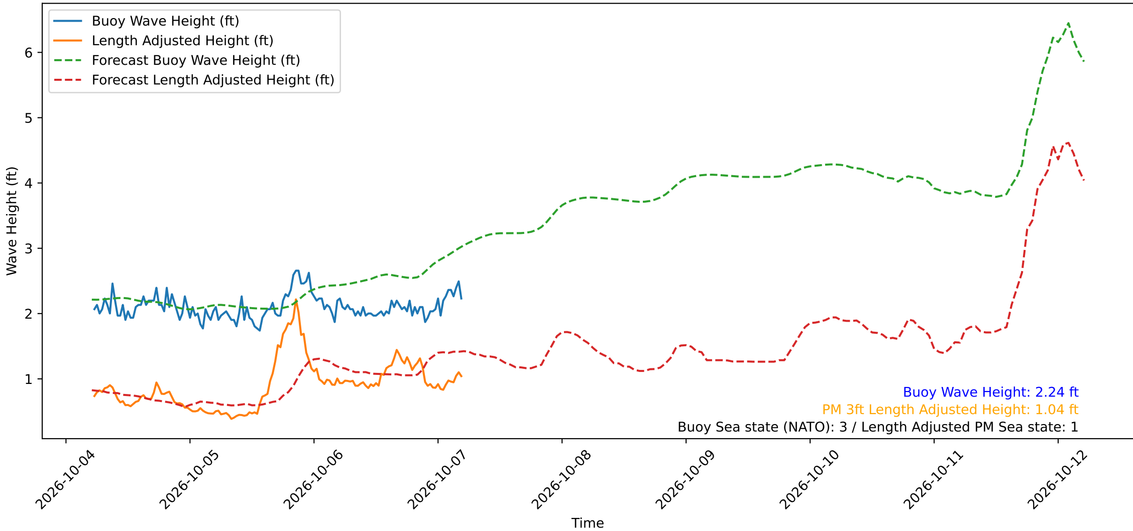
Wave Heights over Time for Red Beach at 2026-10-07 05:20:50
