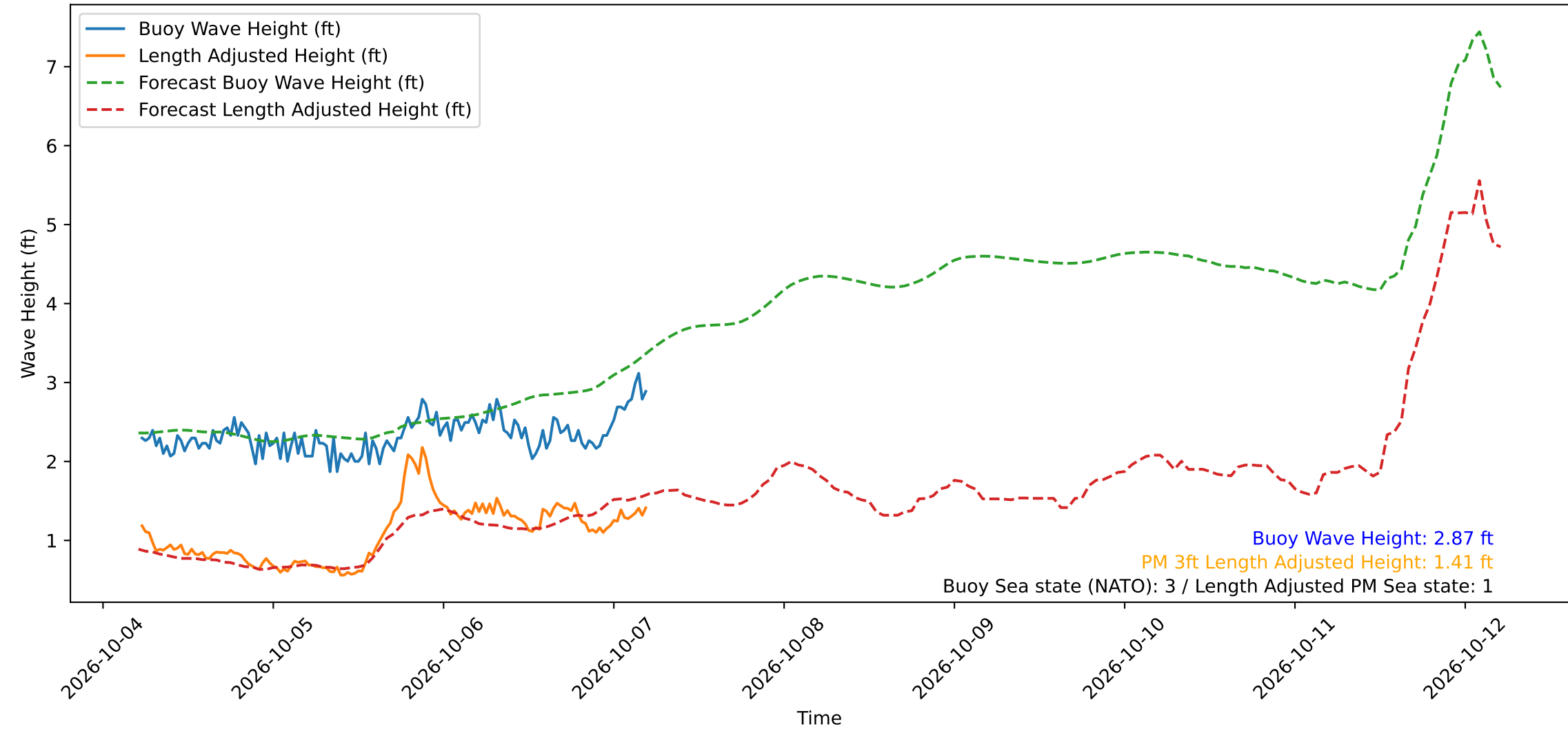
Wave Heights over Time for Oceanside Harbor at 2026-10-07 05:20:29
