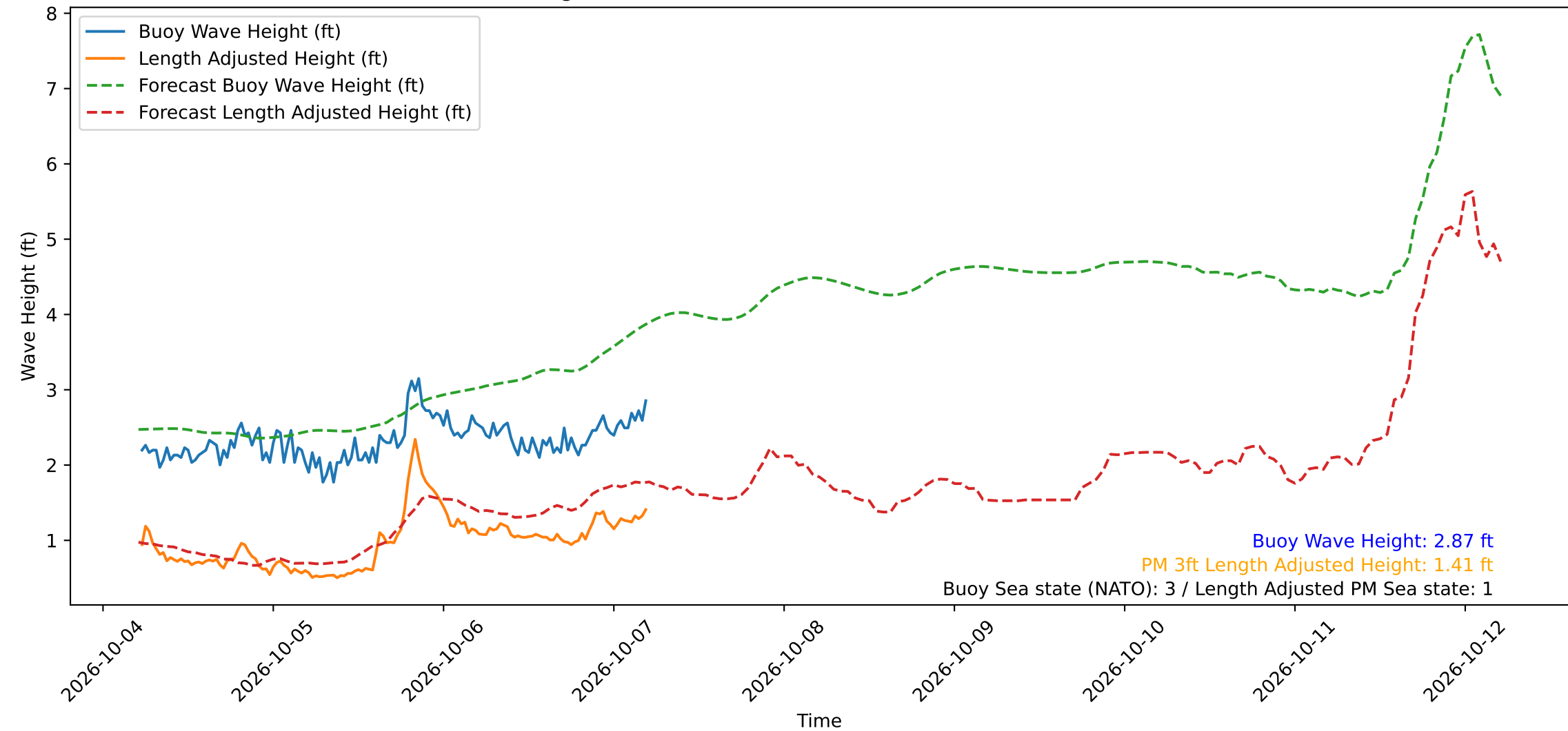
Wave Heights over Time for Green Beach at 2026-10-07 05:21:15
