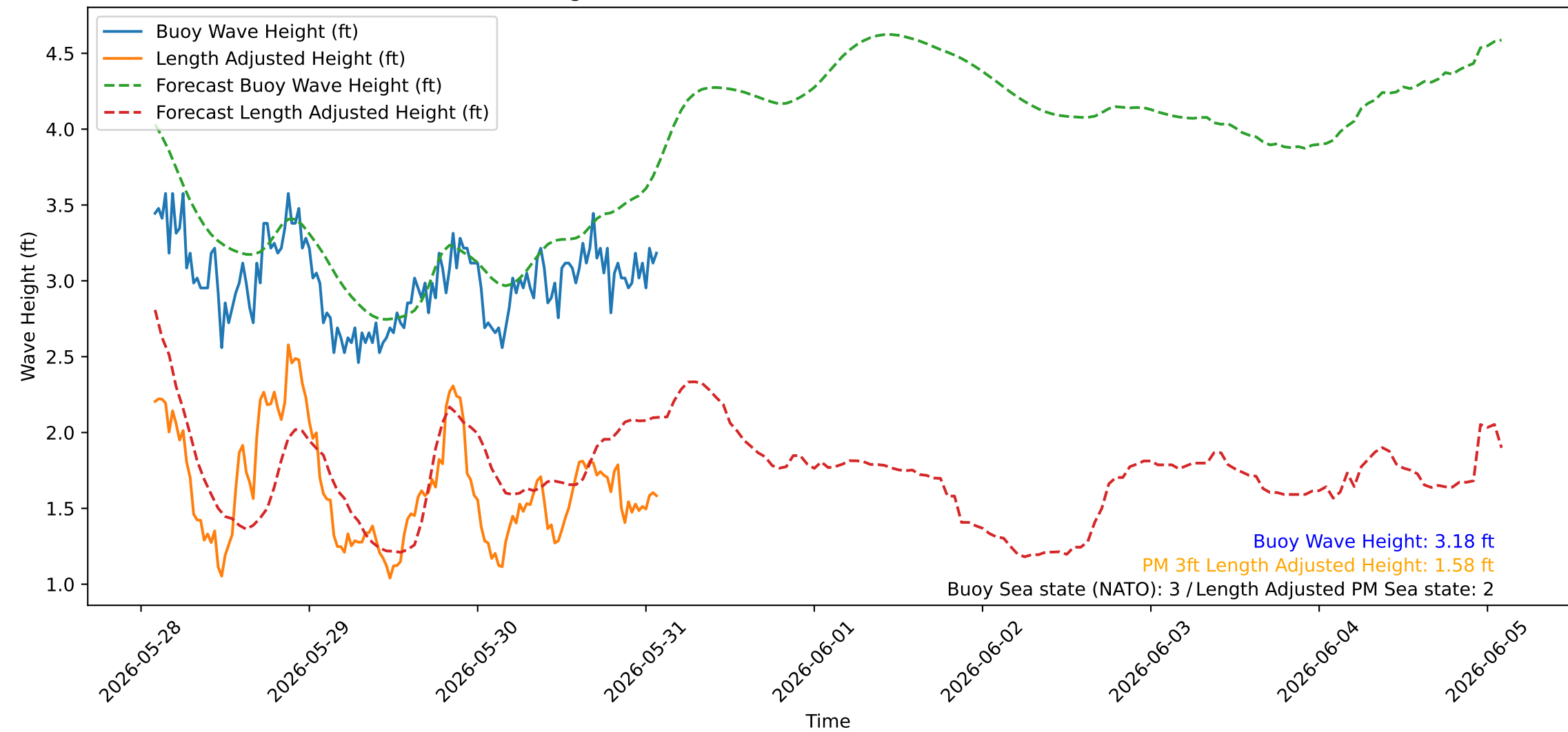
Wave Heights over Time for Green Beach at 2026-05-31 02:11:07
