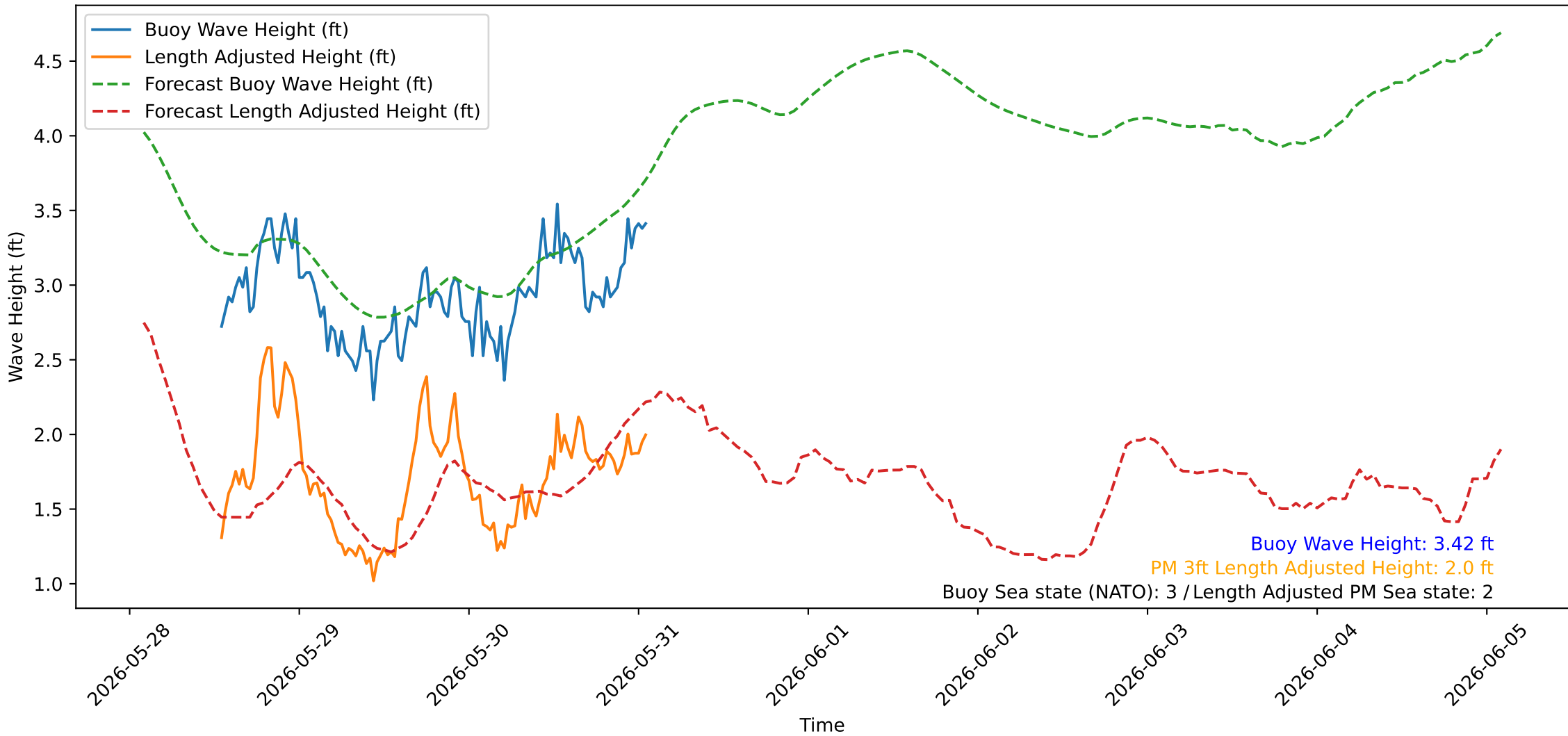
Wave Heights over Time for Oceanside Harbor at 2026-05-31 02:10:25
