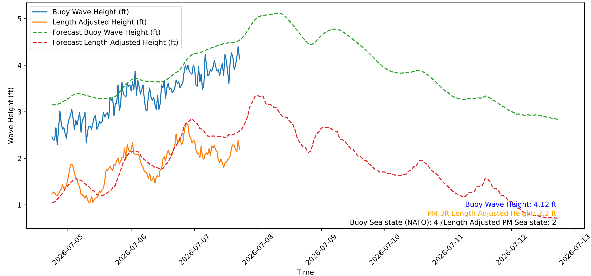
Wave Heights over Time for Oceanside Harbor at 2026-07-07 18:00:27
