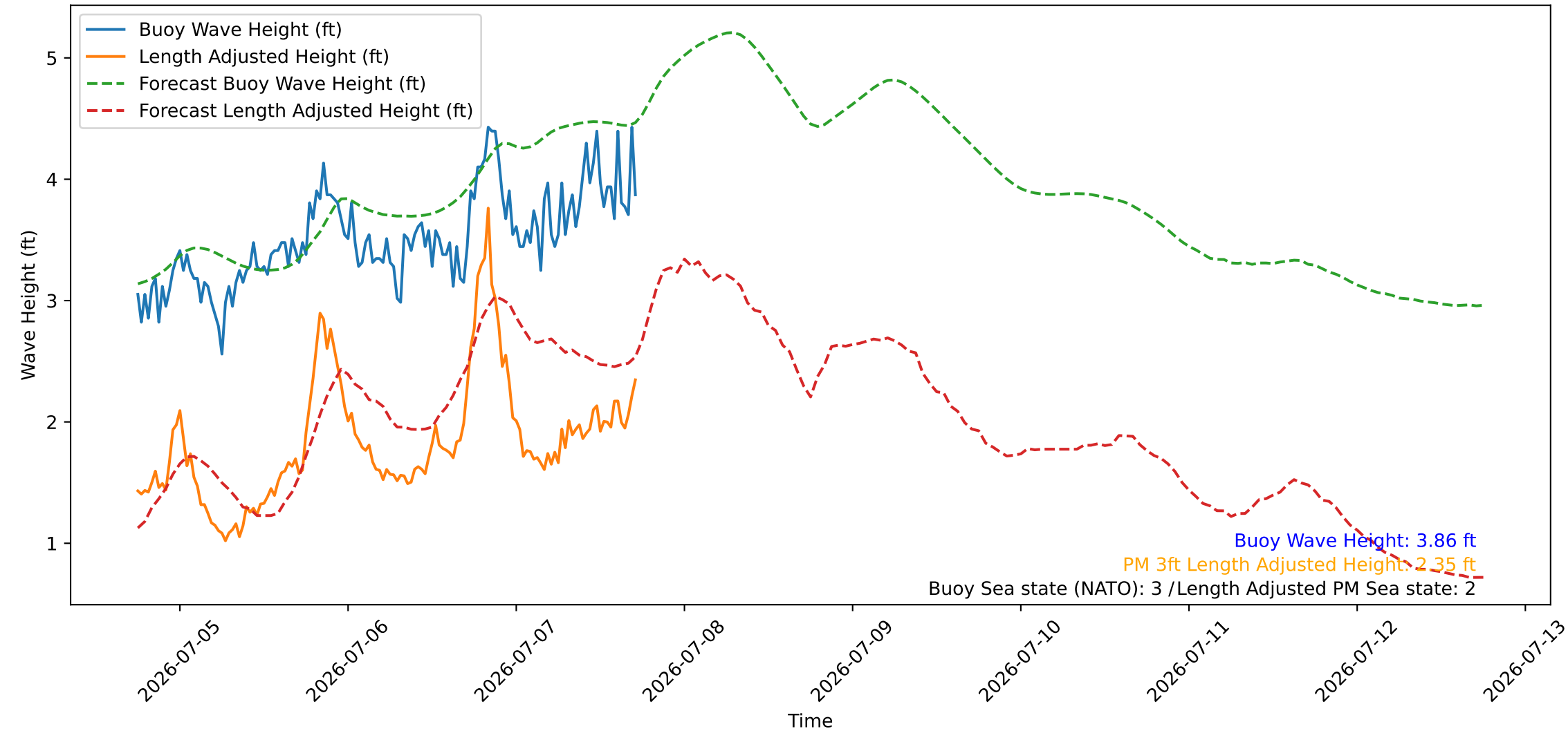
Wave Heights over Time for Green Beach at 2026-07-07 18:01:08
