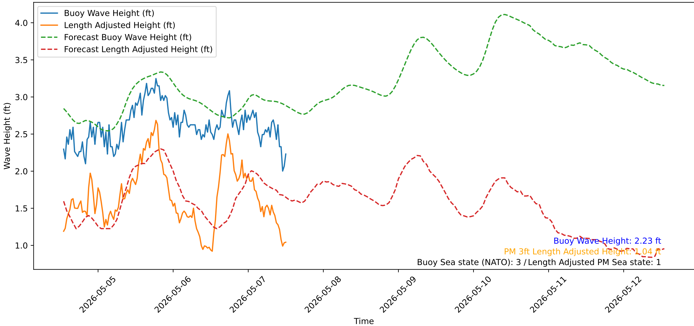
Wave Heights over Time for Oceanside Harbor at 2026-05-07 12:50:31
