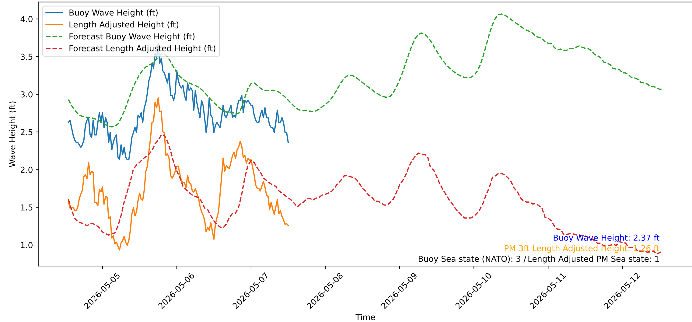
Wave Heights over Time for Green Beach at 2026-05-07 12:51:14
