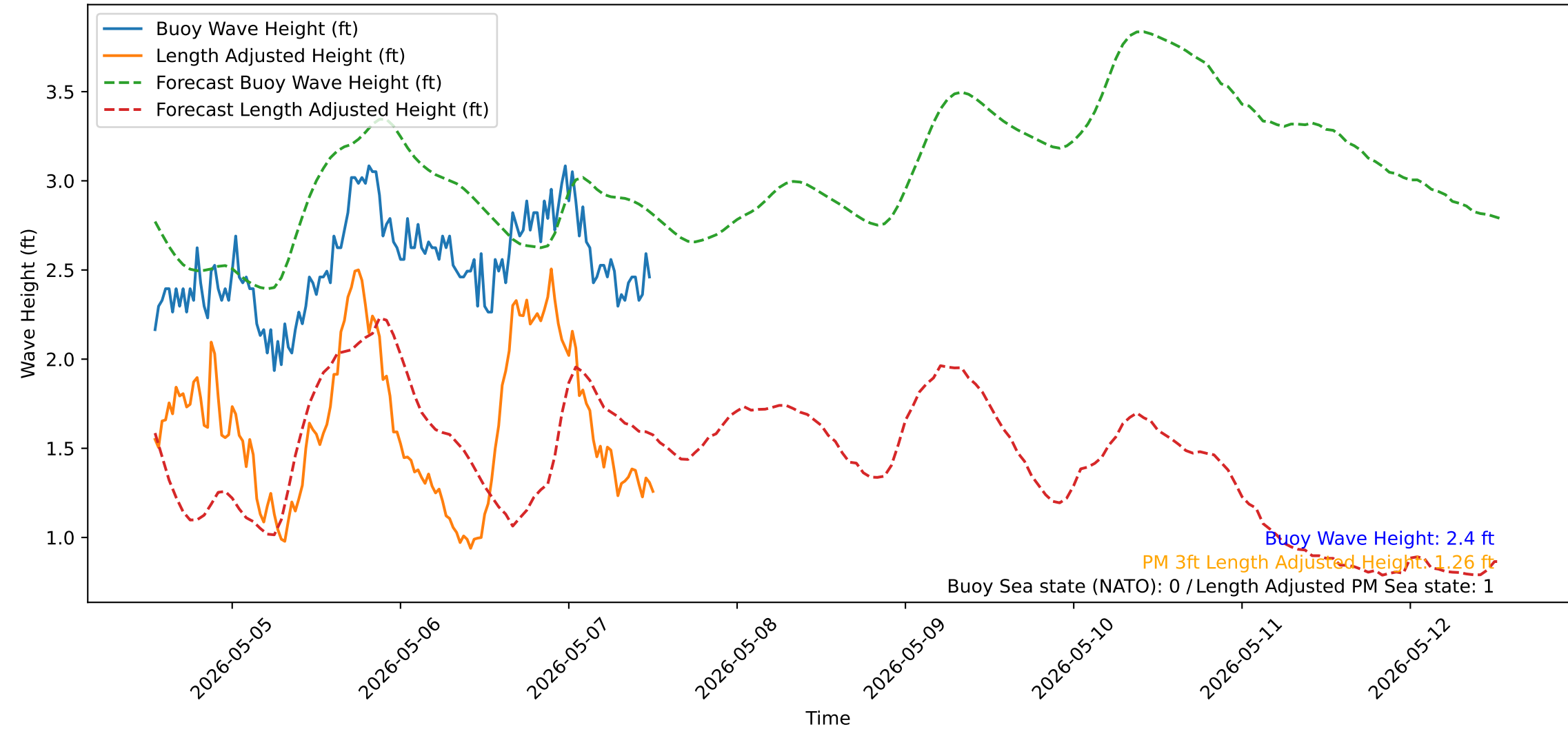
Wave Heights over Time for Red Beach at 2026-05-07 12:50:51
